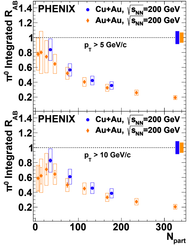
FIG. 7. Comparison of integrated R_{AB} for \pi^0 measured as a function of N_{part} in Cu+Au and Au+Au collisions at \sqrt{s_{NN}} = 200 GeV. Uncertainties are the same as in the Fig. 6. The lower limit of integration is p_T = 5 GeV/c on panel (a), p_T = 10 GeV/c on panel (b).
