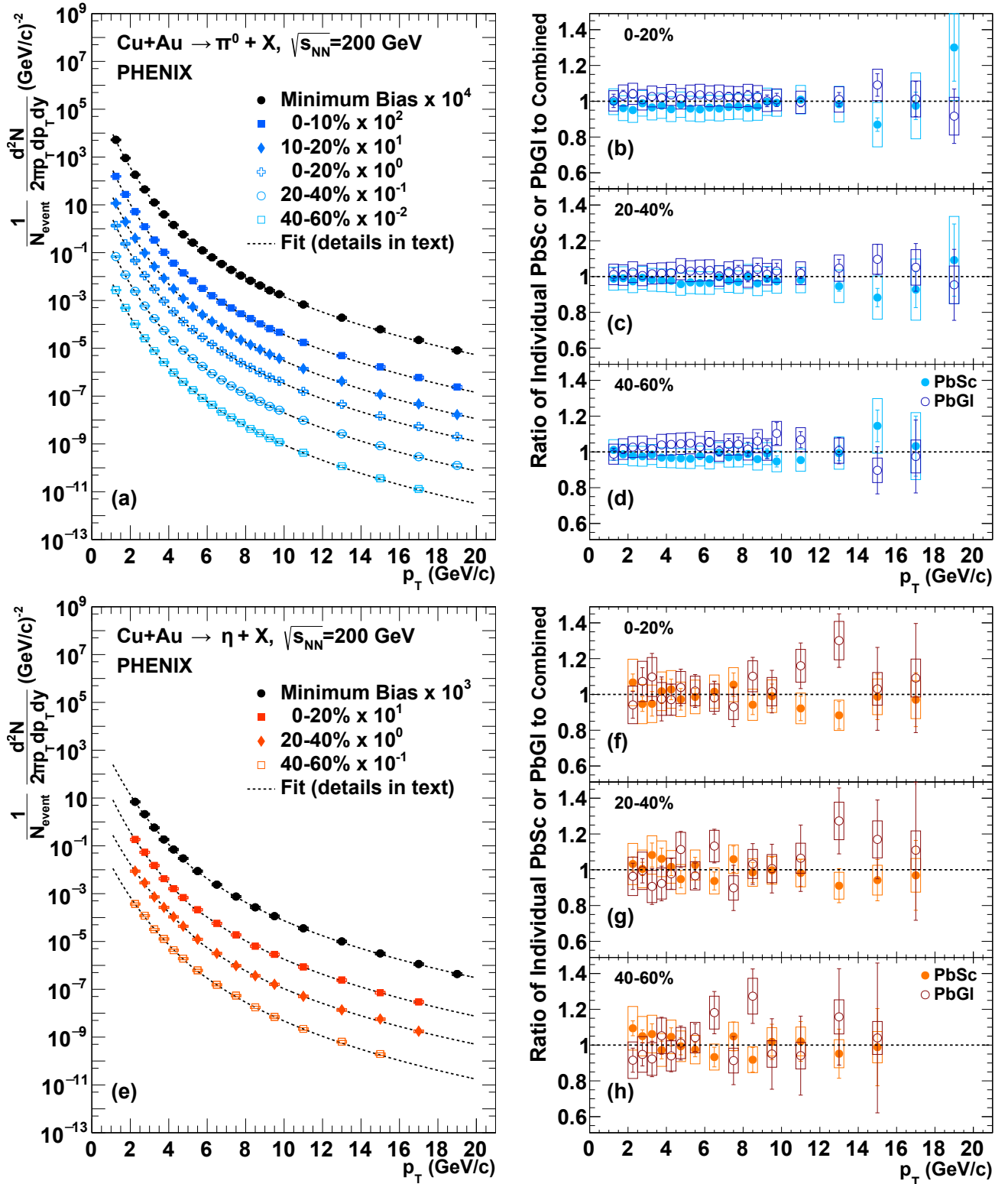
FIG. 3. Left: \pi^0 (a) and \eta (e) invariant p_T -spectra measured in different centrality intervals of Cu+Au collisions at \sqrt{s_{NN}}=200 GeV. The dashed curves are a fit with two Hagedorn-type functions with an asymptotic power-law ( p_T^{-n} ) behavior. Right: ratios of \pi^0 (b-d) and \eta (f-h) yields measured in PbSc or PbGl subsystem to the averaged ones. Error bars represent a quadratic sum of statistical and type-A systematic uncertainties. Error boxes in the right panel correspond to the quadratic sum of systematic uncertainties, which are uncorrelated between PbSc and PbGl.
