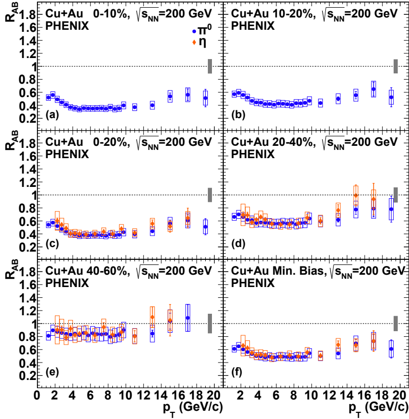
FIG. 5. R_{AB} of \pi^0 and \eta mesons measured as a function of p_T in different centrality intervals of Cu+Au collisions at \sqrt{s_{NN}}=200 GeV. Error bars represent a quadratic sum of statistical and type-A systematic uncertainties from Cu+Au and p+p measurements, respectively. Error boxes represent type-B systematic uncertainties from Cu+Au and p+p measurements. Solid and open boxes at unity represent type-C systematic uncertainties from the T_{AB} values) and p+p , respectively. The reference p+p measurements are published in [12] for \pi^0 and in [30, 38] for \eta (see details in the text).
