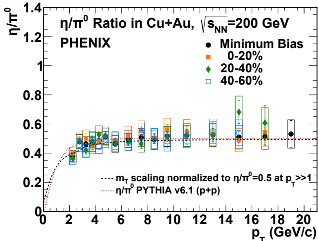
FIG. 4. Ratios of \eta and \pi^0 yields measured as a function of p_T in different centrality intervals of Cu+Au collisions at \sqrt{s_{NN}} = 200 GeV. Dashed curve shows the m_T scaling curve normalized to 0.5 at high momentum (see text). Error bars represent a quadratic sum of statistical and type-A systematic uncertainties for \pi^0 and \eta yields. Error boxes represent a quadratic sum of type-B systematic uncertainties for \pi^0 and \eta yields.
