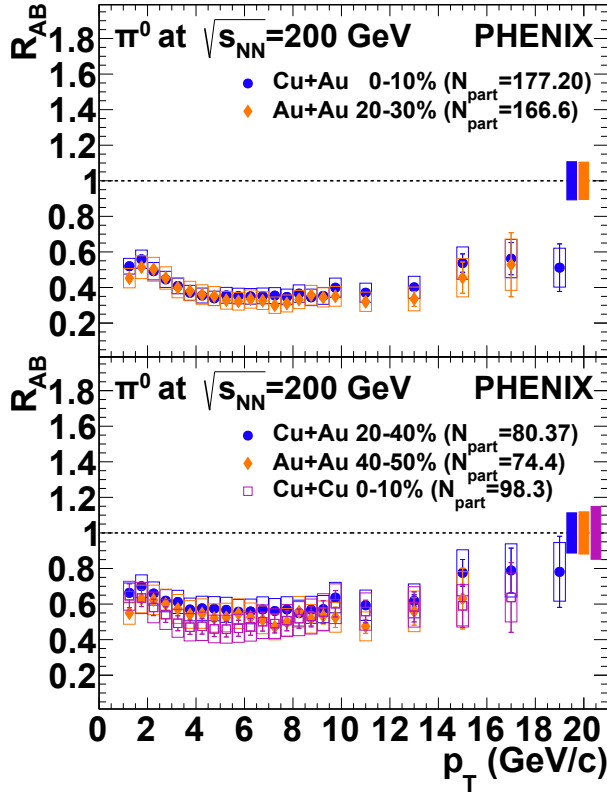
FIG. 6. Comparison of \pi^0 R_{AB} measured in Cu+Au, Au+Au and Cu+Cu collisions at \sqrt{s_{NN}} = 200 GeV and comparable N_{part} . Error bars represent a quadratic sum of statistical and type-A systematic uncertainties from Cu+Au and p+p measurements. Open boxes are Type-B systematic uncertainties for Cu+Au and p+p collisions. The three boxes at unity are type-C systematic uncertainties from p+p and heavy-ion collisions. The boxes from left to right correspond to Cu+Au, Au+Au and Cu+Cu measurements, respectively.
