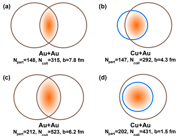
FIG. 1. Cartoon showing Au+Au and Cu+Au collisions with comparable N_{\text{part}} . On panel (b) the overlap area is asymmetric, and part of the dilute surfaces of Au and Cu (corona) overlap.
