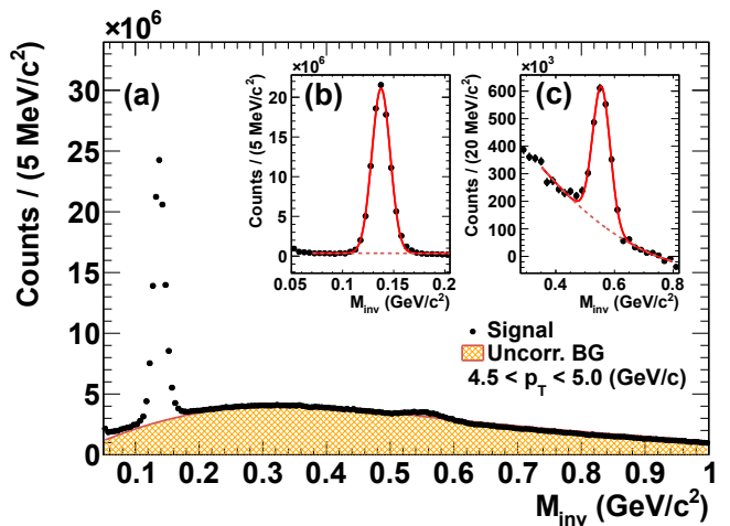
FIG. 2. Example of an invariant mass plot ( 4.5 < p_T < 5.0 GeV/c). (a) The foreground (photon pairs from the same event) is shown as points, the shaded area is the scaled mixed event background. Inset (b) shows the \pi^0 peak area after mixed event subtraction; the Gaussian fit to the peak and the first order polynomial fit to the residual background are also shown. Inset (c) shows the \eta peak area with the Gaussian fit and second order polynomial for the residual background.
