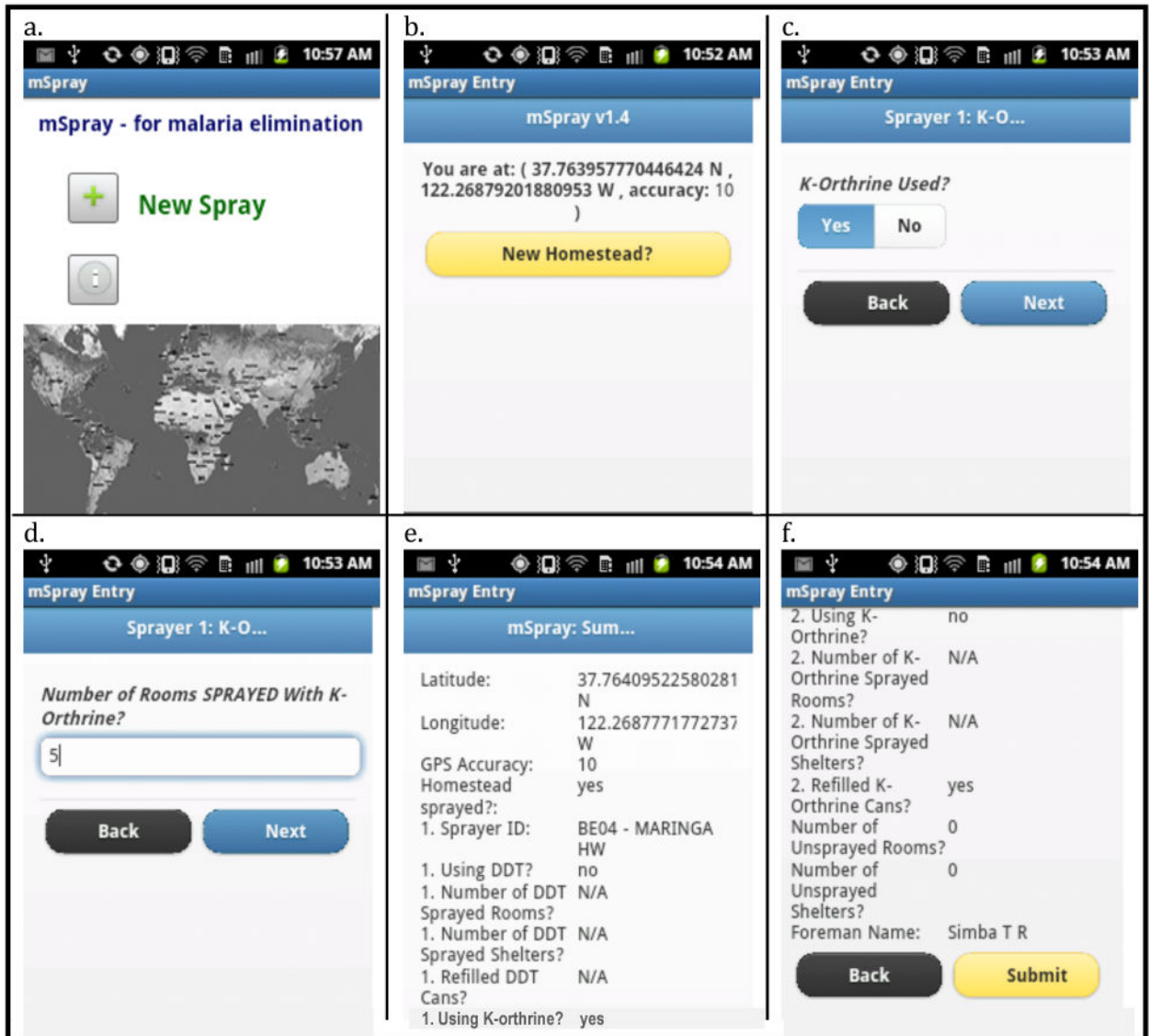
Figure 1. Select screens on the mSpray app
