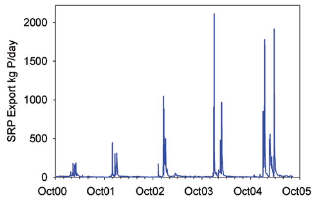
Figure 3. (a) Seasonal trends in SRP concentrations in the Pajaro River. (b) Seasonal trends in SRP export from Santa Clara/San Benito Counties, reflecting rainfall pulses.
