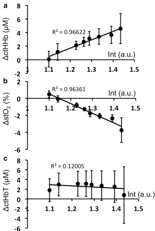
FIGURE 6 Relationship between the change in deoxyhemoglobin concentration \Delta\text{ctHHb} ( a ), hemoglobin oxygen saturation \Delta\text{stO}_2 ( b ), total oxyhemoglobin concentration \Delta\text{ctHbT} ( c ), and the change in the NADH fluorescence intensity ( \text{Int} ), during arterial occlusion. Error bars represent standard deviation.
