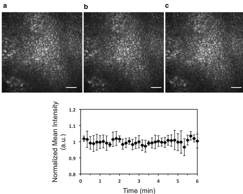
FIGURE 4 Representative TPEF in vivo images of human keratinocytes from time series corresponding to (a) t = 2 min (b) t = 4 min (c) t = 6 min. Scale bar is 20\ \mu\text{m} . The graph represents the average of normalized mean intensities of TPEF images as a function of time. Error bars represent standard deviation.
