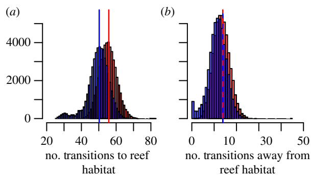
Figure 3. Estimated number of transitions to and from reef habitats within acanthomorph fishes. (a) Histogram of the estimated number of transitions from non-reef to reef habitat in the real data (blue) and the non-phylogenetic null (red). (b) Histogram of the estimated number of transitions from reef to non-reef habitats in the real data (blue) and the non-phylogenetic null (red). Estimated using a total of 50 000 stochastic character maps generated in SIMMAP [27]. The vertical lines indicate the average number of transitions. These distributions illustrate the variability in the number of transitions owing to the uncertainty in the character mapping as well as the tree topology, branch lengths and reef-living.
