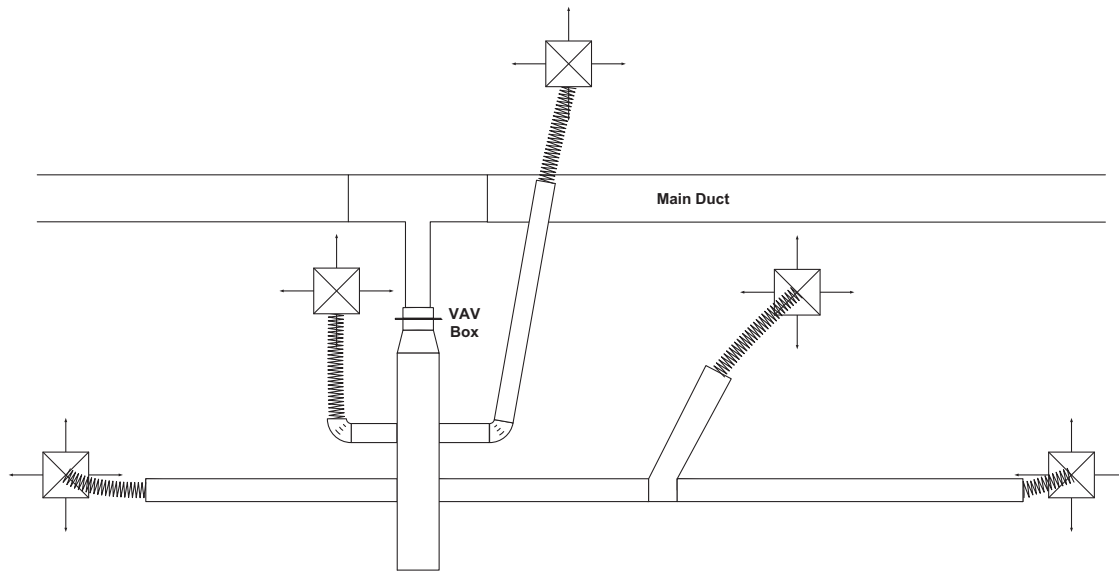
Fig. 2. System section in Sacramento office building that was used for validating modified fan pressurization protocol.
