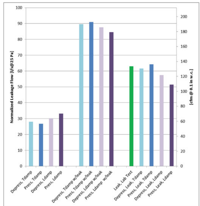
Fig. 3. Section leakage determined using the modified fan pressurization protocol under different conditions: pressurization (Press) and depressurization (Depress), tight (Tdamp) and leaky (Ldamp) VAV box inlet damper, with and without added leak.
