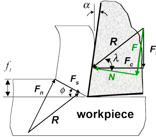
Figure 5. Cutting diagram.
