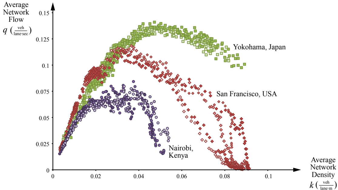
Figure 2.3. Experimental Macroscopic Fundamental Diagrams (MFDs) from measurement in Yokohama (Geroliminis & Daganzo, 2008) and simulations in San Francisco (Geroliminis & Daganzo, 2007) and Nairobi (Gonzales et al. , 2011)
