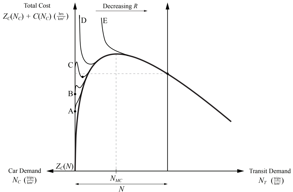
Figure 4.6. Total generalized cost of car and transit in the evening with congestion
