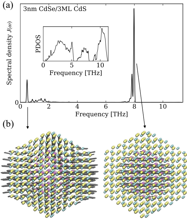
Figure 2: (a) The calculated spectral density of a 3nm core, 3ML shell CdSe/CdS NC using our model. The inset shows the phonon density of states for this core-shell NC. (b) The motions of one acoustic phonon mode and one optical phonon with the strongest coupling to the exciton are shown. Color schemes: blue-Cd, purple-Se, yellow-S, black arrows-phonon mode motion.
