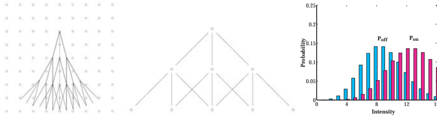
Figure 2: Left panel: the tree structure superimposed on the lattice. Centre panel: a pyramid structure used in the simulations on the rectangular grid. Right panel: Typical distributions of P_{\text{on}}, P_{\text{off}}
