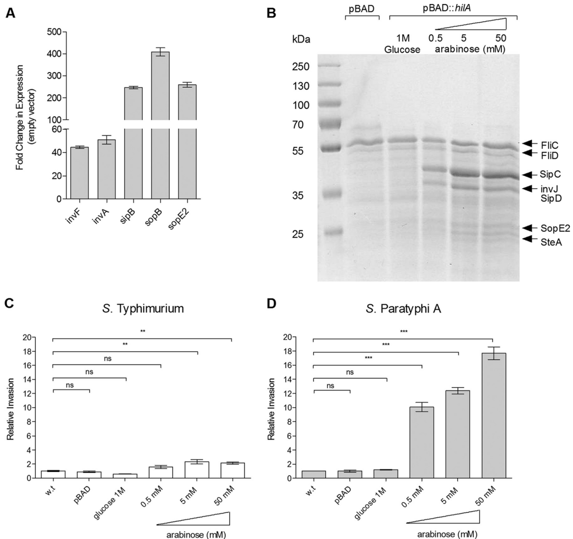
FIG 5 Induced expression of SPI-1 increases S. Paratyphi A invasion. (A) Total RNA was harvested from S. Paratyphi A 45157 carrying pBAD18 or pBAD::hilA grown in LB supplemented with 100 \mu l/ml ampicillin and 50 mM arabinose to late logarithmic phase aerobically and was subjected to qRT-PCR. The fold change in the abundance of SPI-1 gene transcripts (normalized to rpoD ) in S. Paratyphi A harboring pBAD::hilA is shown relative to their expression in S. Paratyphi A carrying pBAD18. The indicated values present the means and the SEM from three independent RT-PCR experiments from two independent RNA extractions. (B) S. Paratyphi A cultures were grown aerobically in LB to logarithmic phase and normalized to an OD 600 of 1.2. Secreted fractions from S. Paratyphi A carrying pBAD18 (lane 2) or pBAD::hilA grown in the presence of 1 M glucose (lane 3) or increasing arabinose concentrations (lanes 4 to 6) were separated on SDS-12% polyacrylamide gels and stained with Coomassie G-250. (C) S. Typhimurium SL1344 (wild type) and its isogenic strains carrying pBAD or pBAD::hilA were grown in LB, LB supplemented with 1 M glucose, or LB with increasing concentrations of arabinose under aerobic conditions and used to infect HeLa cells. Invasion is shown relative to that of the wild-type strain (grown in LB supplemented with 50 mM arabinose), presenting a 3.7\% \pm 0.76\% invasion rate (from the infecting inoculum) under these conditions. (D) S. Paratyphi A 45157 and its isogenic strains carrying pBAD or pBAD::hilA were grown and used to infect HeLa cells as described for panel C. Invasion is shown relative to that of the S. Paratyphi A wild-type strain, presenting, on average, 0.05\% \pm 0.001\% invasion. ANOVA with Dunnett's multiple-comparison test was implemented to compare the invasion of the different strains to that of the wild type. The results represent the means and SEM from at least three biological replicates. **, P < 0.01 ; ***, P < 0.0001 ; ns, not significant.
