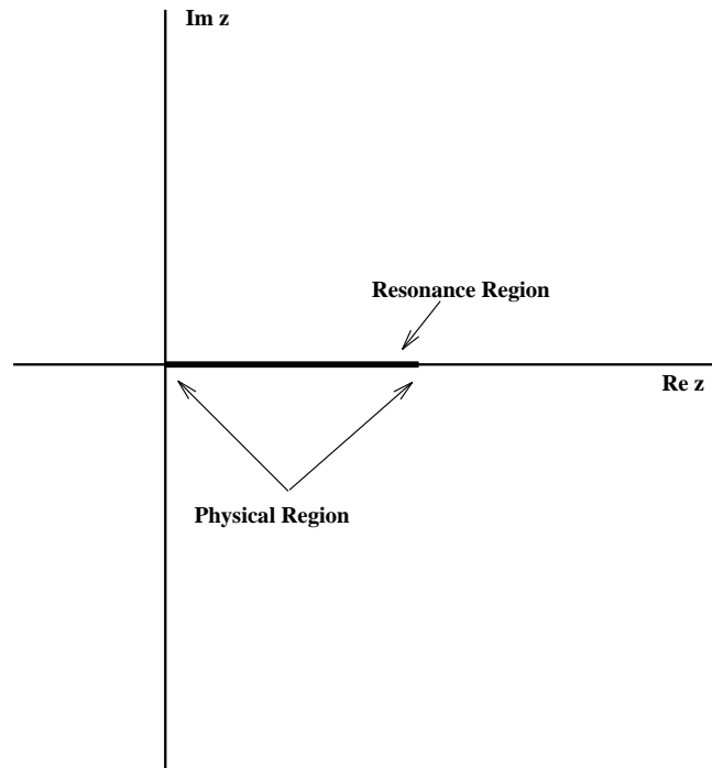
Figure 4 The location of the physical and resonant regions in the complex z -plane. The variable z is the energy of the final hadronic system in the semileptonic B decay, in the B restframe.
