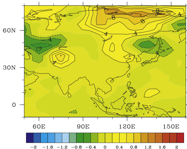
Figure 7. Differences in the July mean surface air temperature ( ^{\circ}\text{K} ) between the experiments CHIN and AERO.
