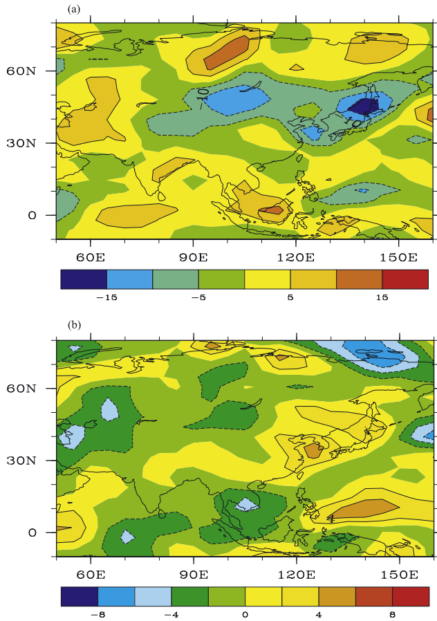
Figure 6. Differences in the July mean (a) net surface solar fluxes ( \text{W m}^{-2} ) and (b) cloud cover (%) between the experiments CHIN and AERO.
