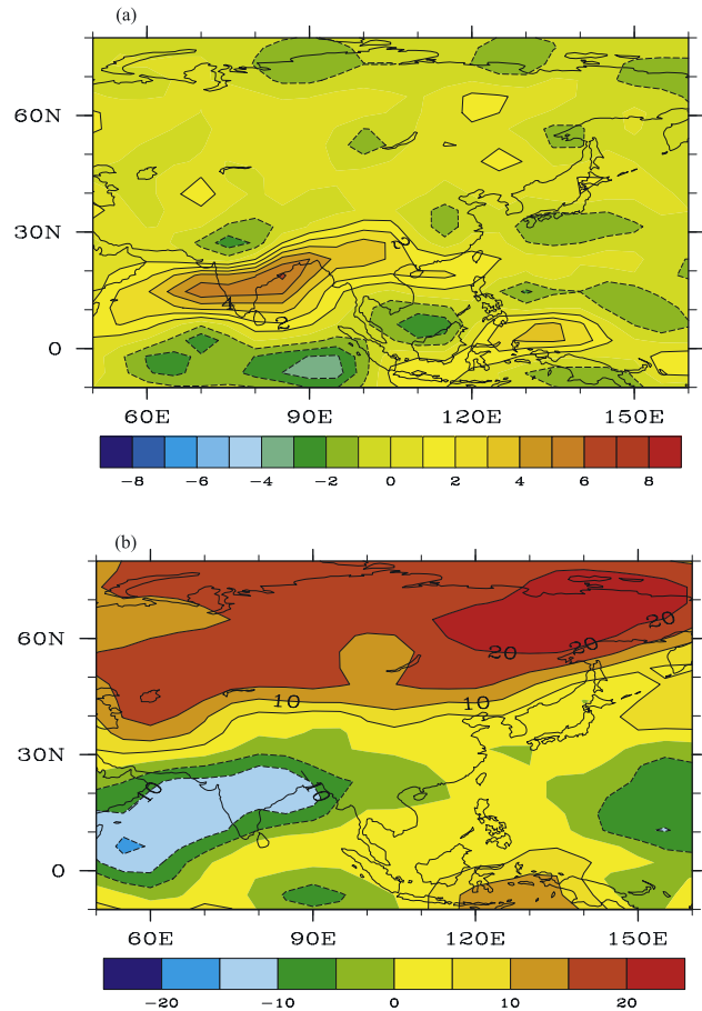
Figure 8. Differences in the July mean (a) precipitation ( \text{mm d}^{-1} ) and (b) OLR ( \text{W m}^{-2} ) between the experiments CHIN and AERO.
