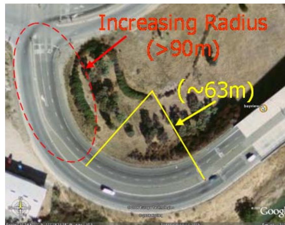
Figure 4.6 Exit ramp from northbound I-580 to Bayview Ave. (Google Map)
