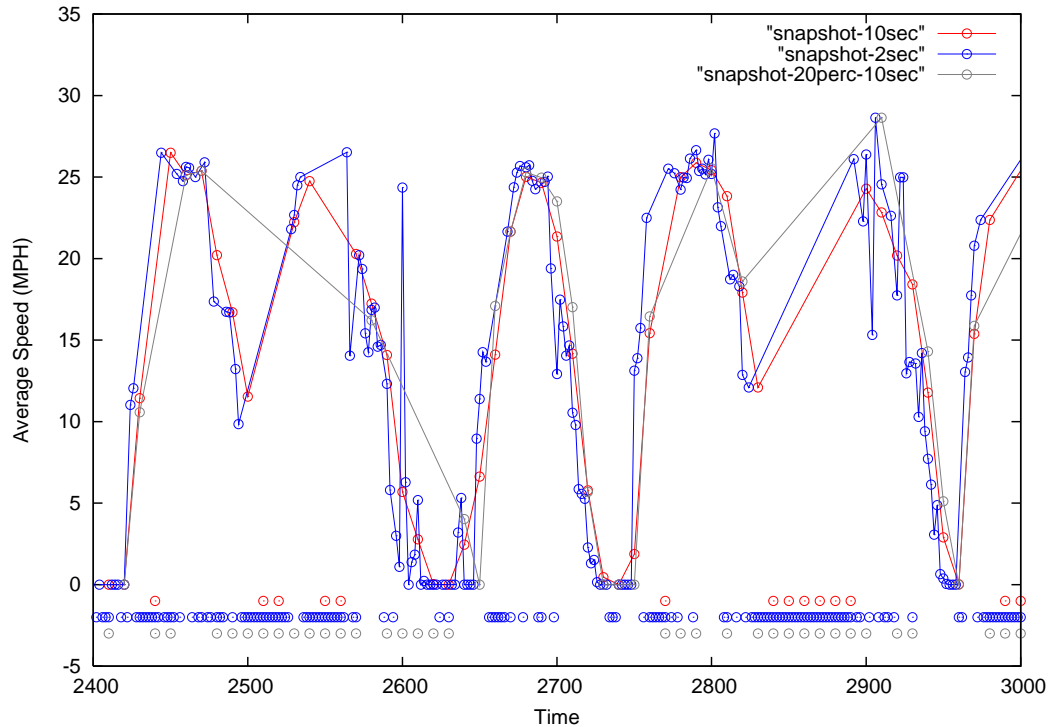
FIGURE 4.26 Simulation snapshot data averaged over 2 s and 10 s intervals and 20% market penetration averaged over 10 s.
