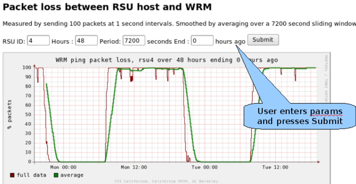
Figure 3.3 Graph of Packet Loss
