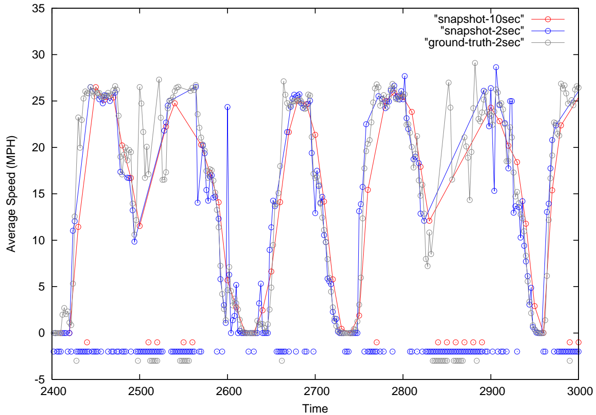
FIGURE 4.22 Effects of Probe Snapshot Sampling on Speed Estimates at 50-100 m from Intersection.
