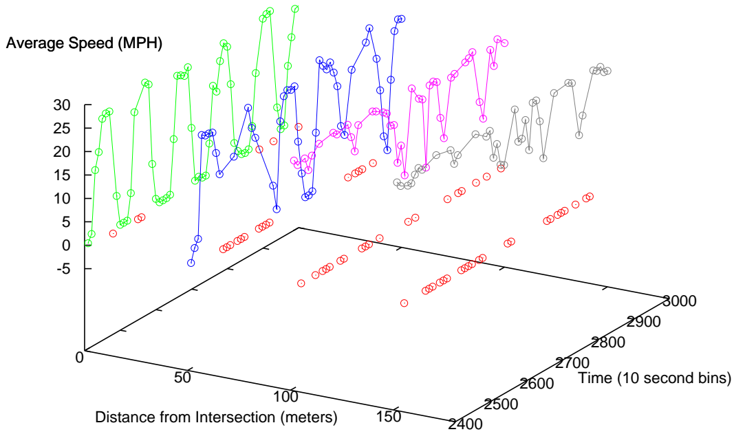
FIGURE 4.23 Aggregation of complete vehicle trajectories at 20% market penetration
