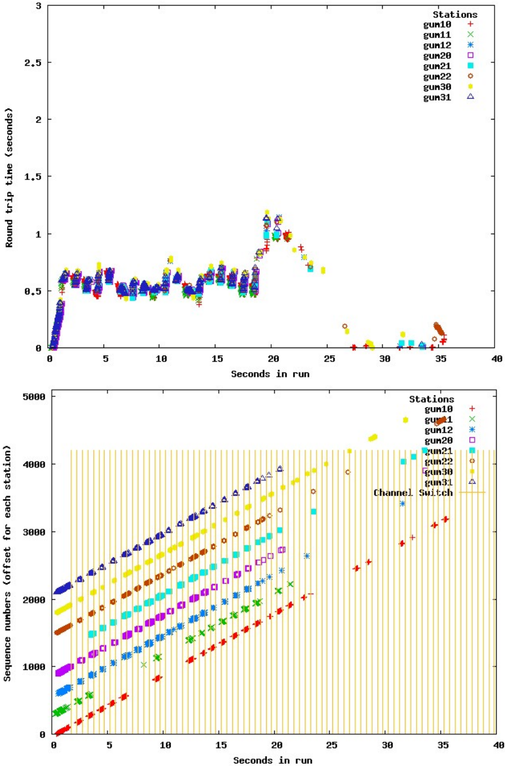
Figure 3.25 Eight radios, each sending 200 byte packets at 10 ms intervals, with background channel switching twice a second, during a short ride on a test track at Richmond Field Station.
