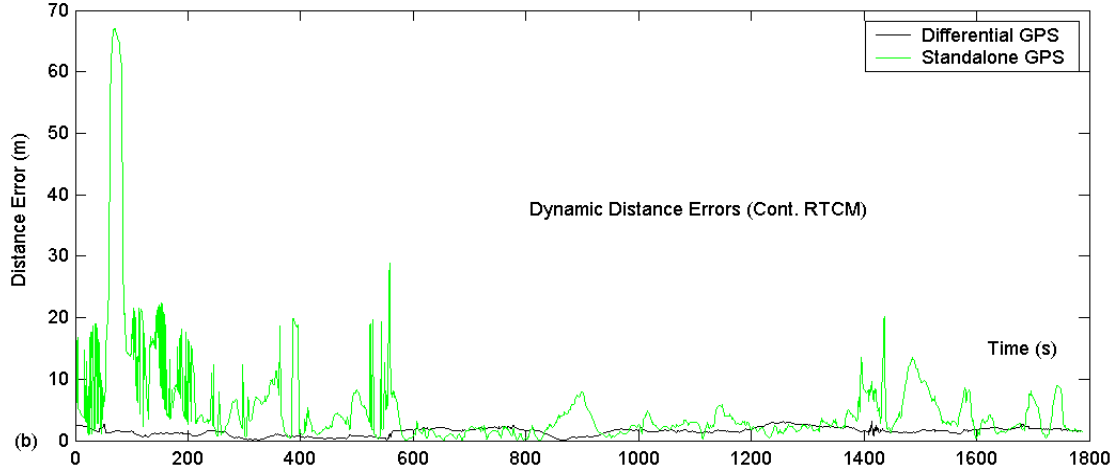
Figure 4.49 Positioning error for uncorrected (green) and corrected (black) local differential GPS system [Du et al., 2006].
