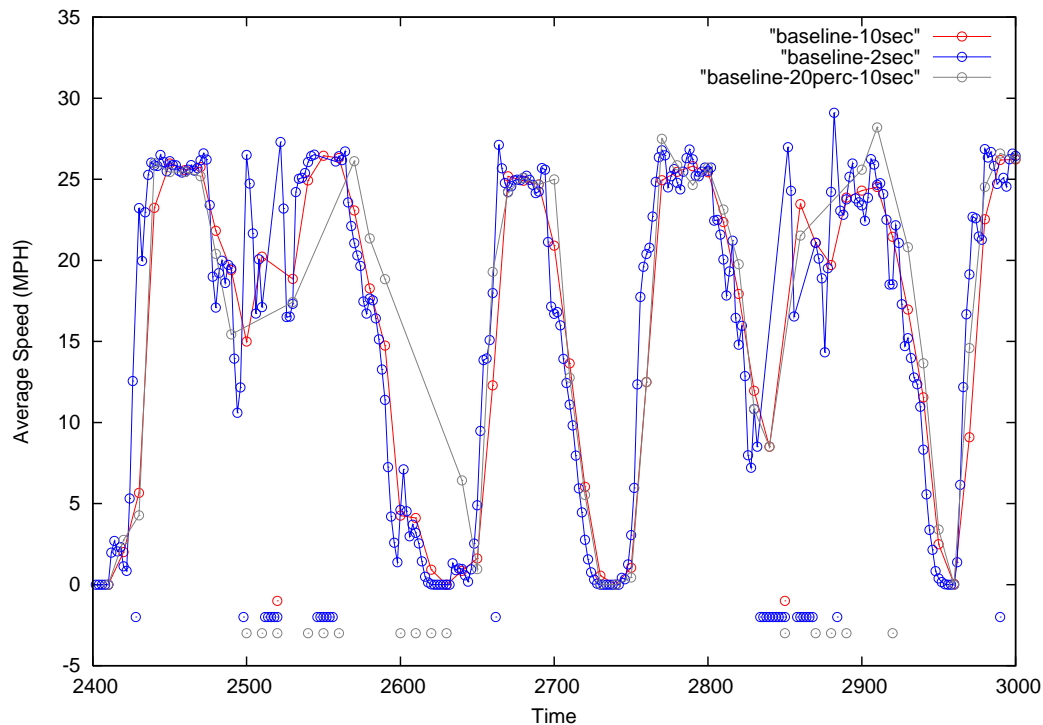
FIGURE 4.25 Raw simulation speed profile averaged over 2 s and 10 s intervals and 20% market penetration averaged over 10 s
