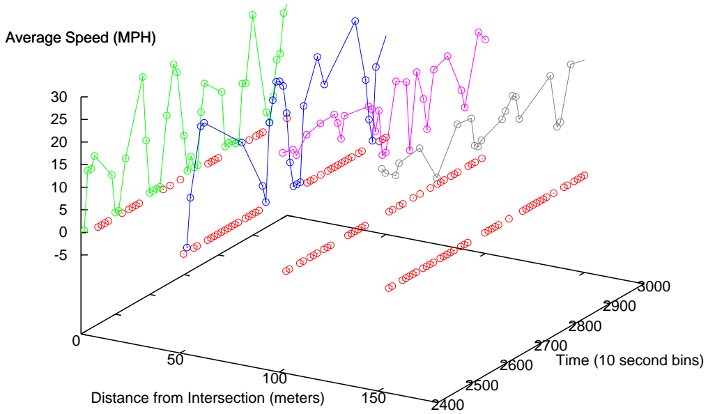
FIGURE 4.24 Aggregation of probe snapshots at 20% market penetration
