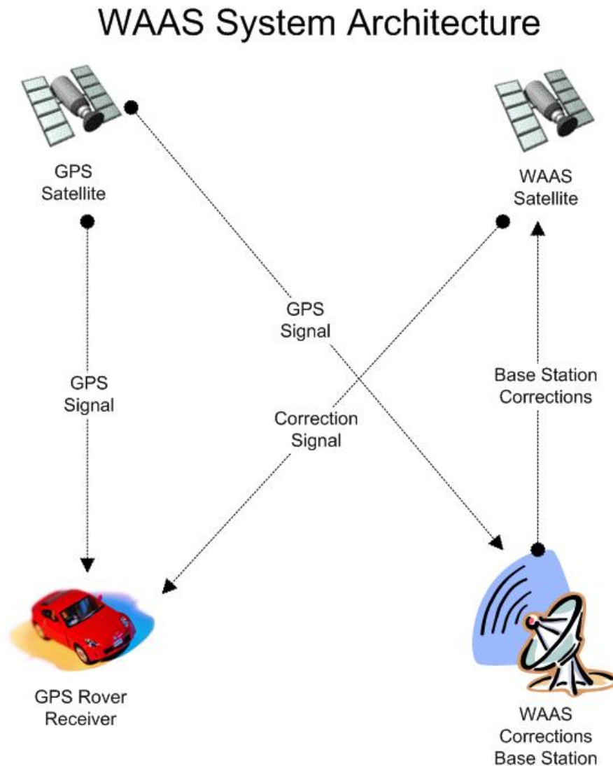
Figure 4.56 Proposed WAAS architecture for potential VII CALIFORNIA implementation.
