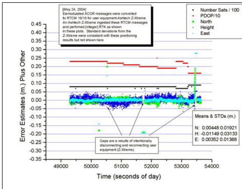
Figure 4.45. HA-NDGPS evaluation of compaction of RTCM 18/19 message types [FHWA,2005].
