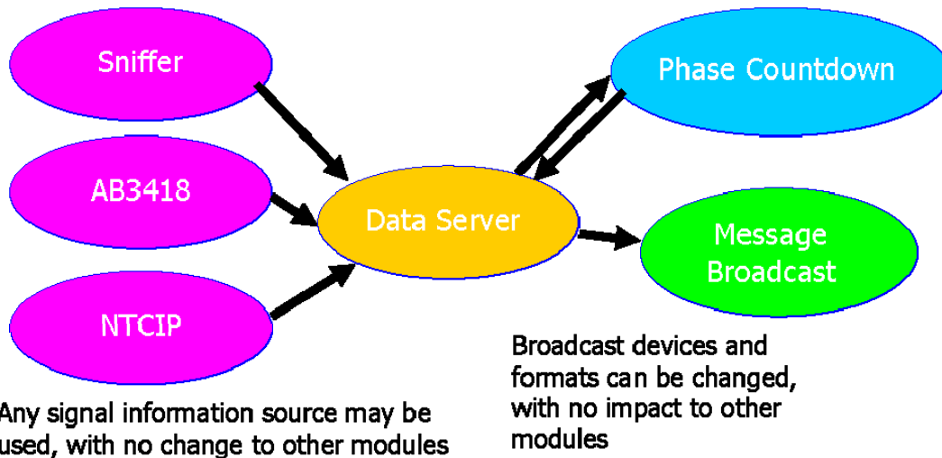
FIGURE 4.36 Modular design of signal phase acquisition and broadcast system
