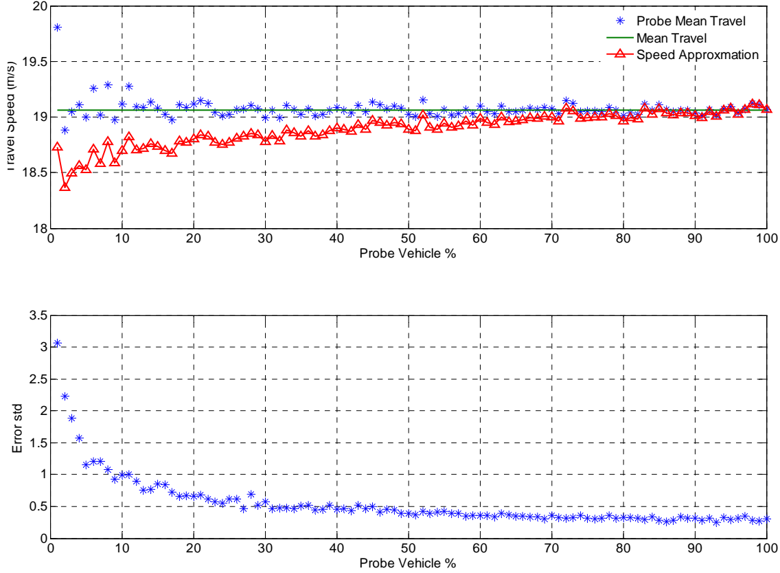
FIGURE 4.29 Performance of the Cruise Speed Estimation Model
