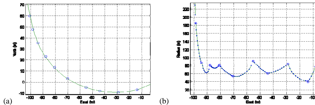
Figure 4.3 (a) Road curve fitted by splines (b) Radius of curvature derived from splines
