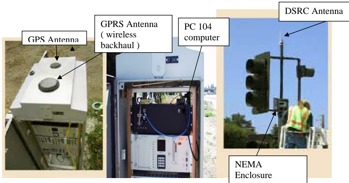
Figure 2.3 Left and Center: VII California RSE Mounted in Type 332 Cabinet on Caltrans Right of Way; Right: DSRC Radio Enclosure and Antenna Mounted on Ramp Meter Signal Pole at Freeway Onramp.
