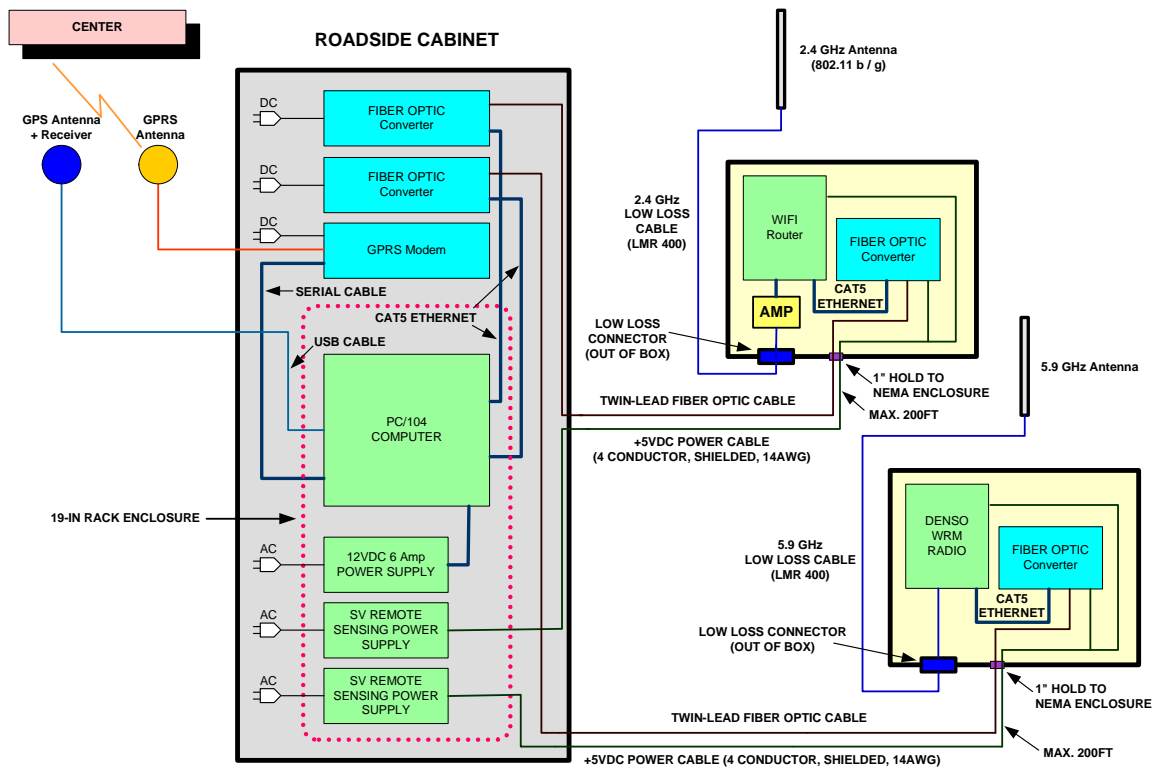
Figure 4.52 VII CALIFORNIA proposed RSE architecture [VII CALIFORNIA, 2006a].
