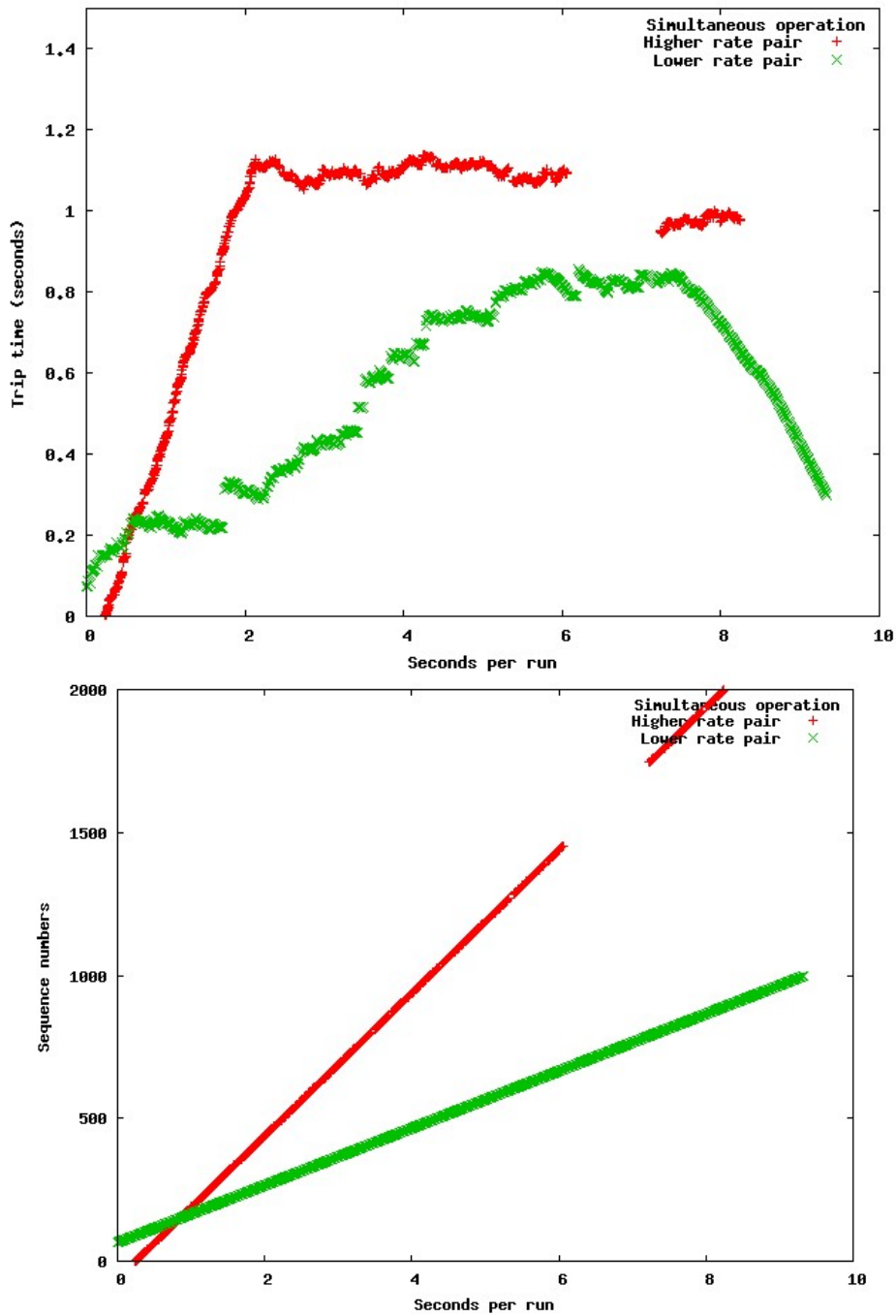
Figure 3.14 Large increase in trip time due to interference between a higher rate pairwise communications stream (1480 byte packets at 4 ms interval between sends) and a lower rate stream (1480 byte packets at 10 ms interval between sends). Note that the scale for trip time is in seconds; the lower graph shows sequence numbers.
