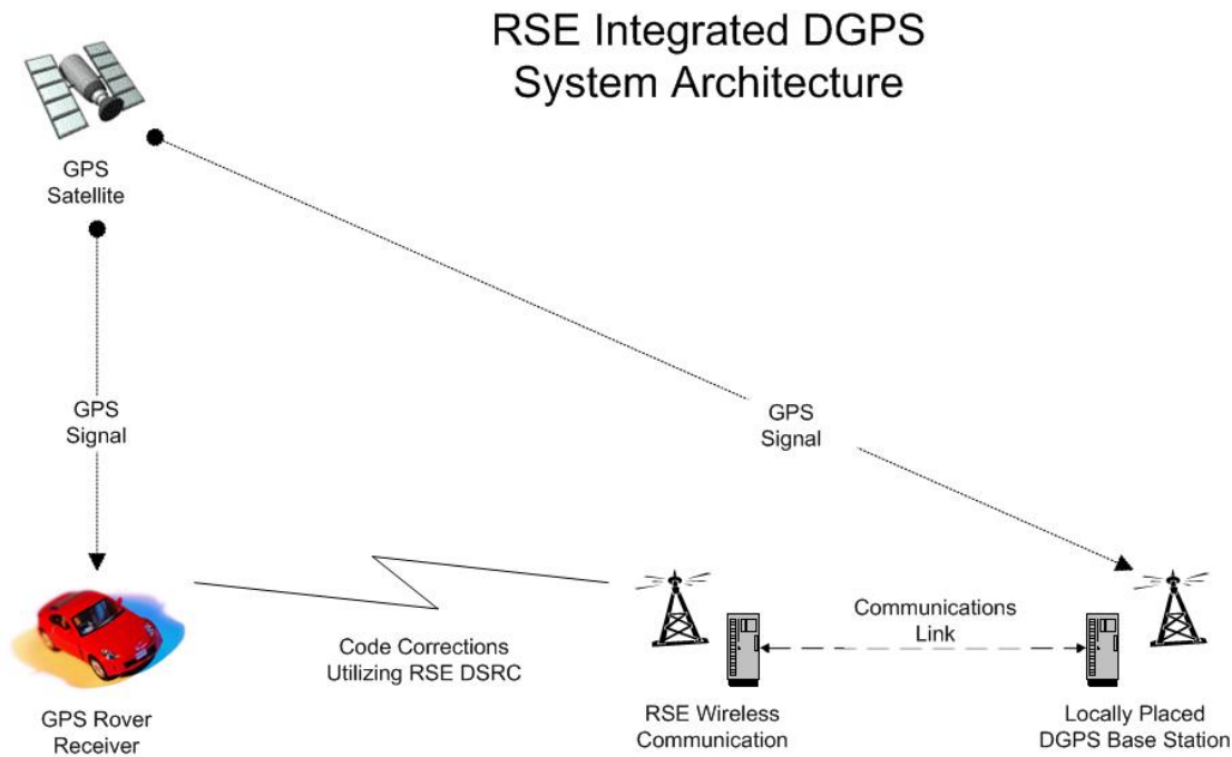
Figure 4.58 Proposed RSE integrated DGPS architecture for potential VII CALIFORNIA implementation.
