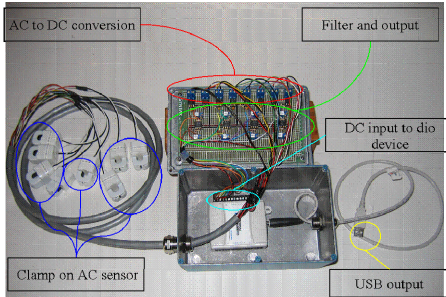
FIGURE 4.35 Depiction of “clamp-on” signal sniffer.
