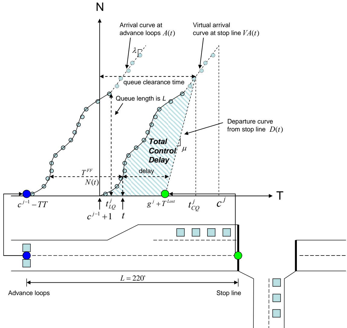
FIGURE 4.30 Delay Calculation Model with Typical Semi-actuated Control Layout
