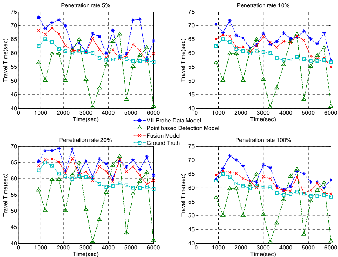
FIGURE 4.33 Model Performance Comparisons for a NB Link
