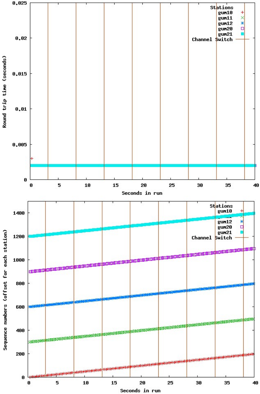
Figure 3.18 In this case, sw2, the send rate is half that of sw1, and round trip time remains low.
