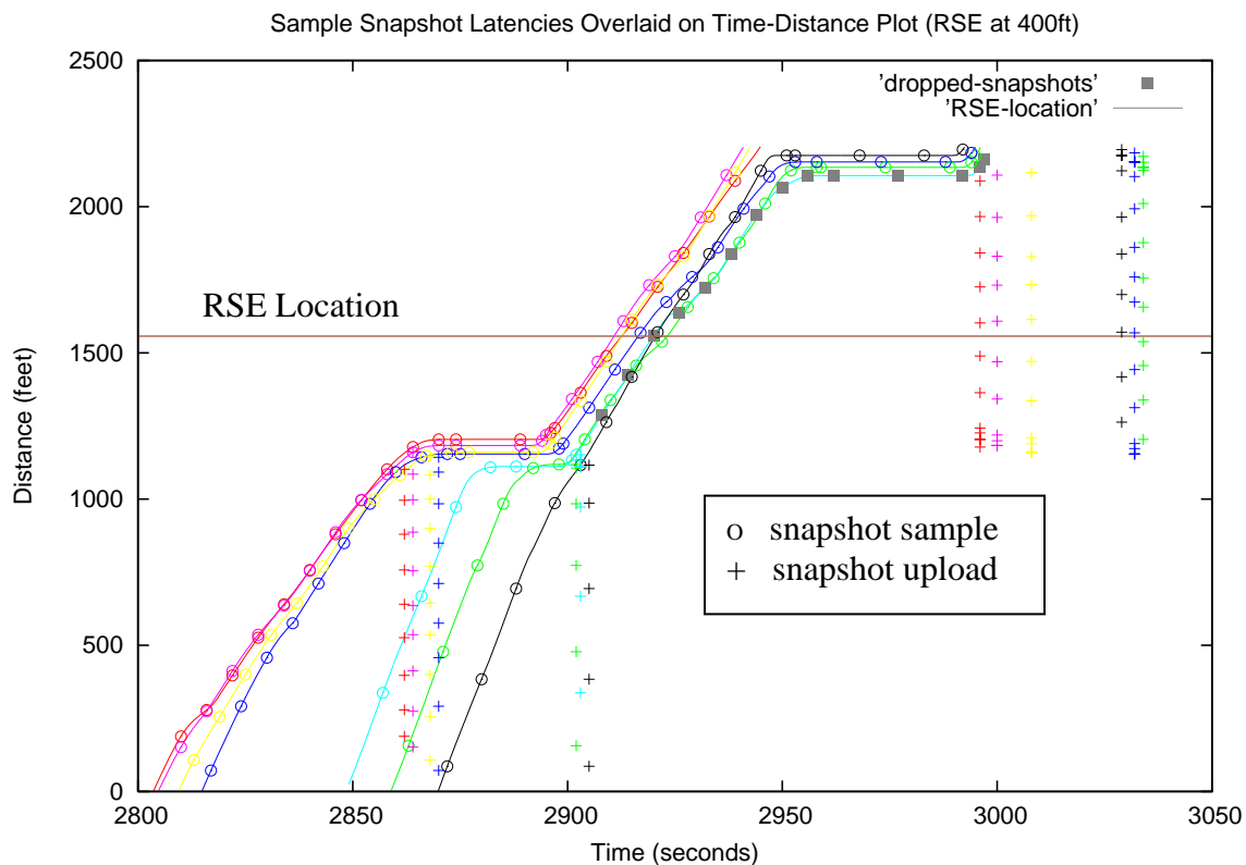
FIGURE 4.17 Examples of Delays between Probe Snapshot Sampling and Message Uploading to RSE.
