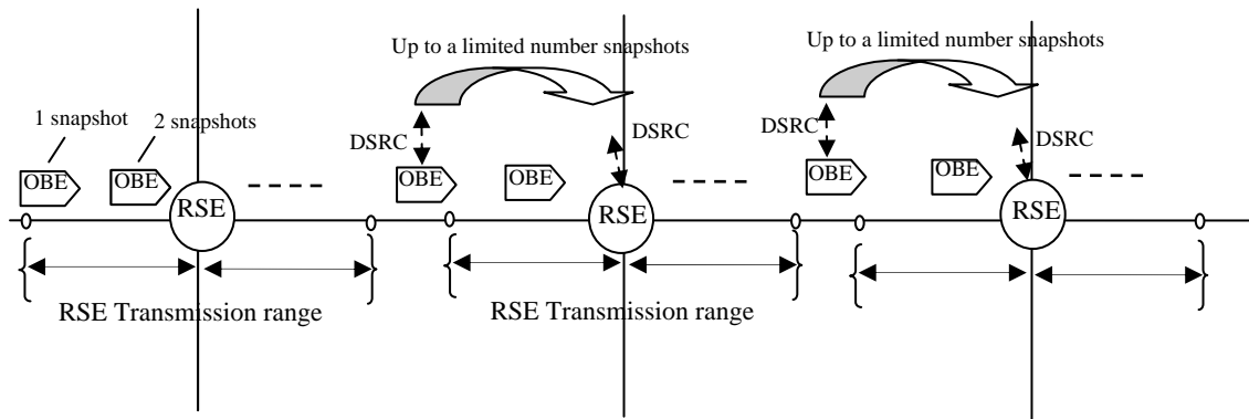
FIGURE 4.27 VII Probe Data Collection Process
