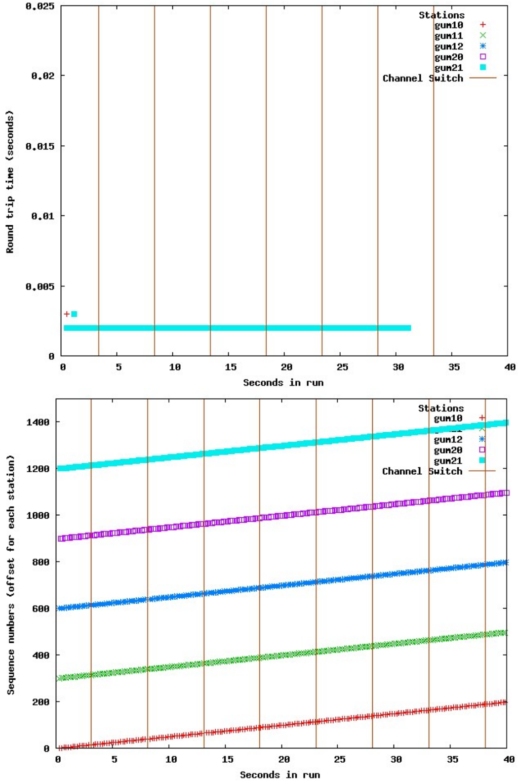
Figure 3.19 In this case, sw3, the send rate is twice that of sw1, and but the delivery of packets, as shown by sequence numbers remains good and the round trip time remains low.
