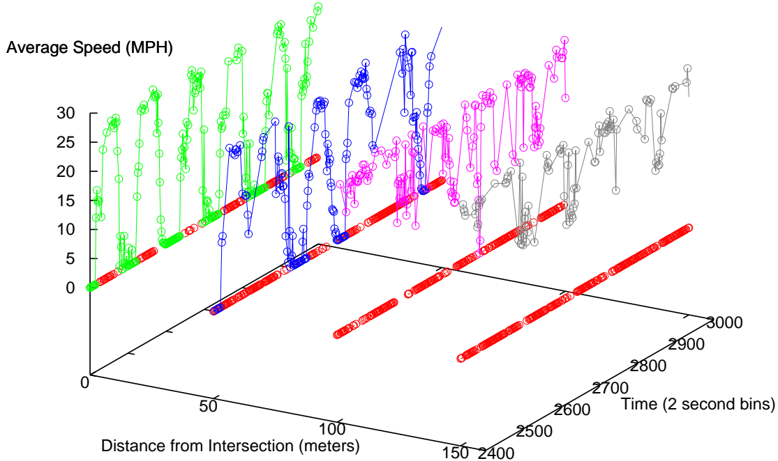
FIGURE 4.21 Average Speeds Derived from Five Minutes of Probe Snapshots.
