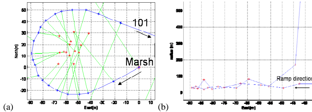
Figure 4.10 (a) Preliminary curvature estimates by CCS algorithm (b) Preliminary estimates of curvature radii by CCS algorithm
