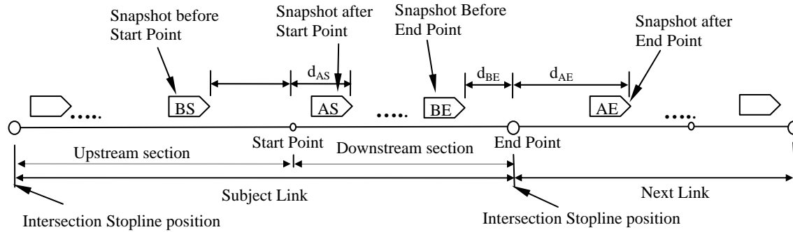
FIGURE 4.28 Typical snapshots distribution near around downstream section
