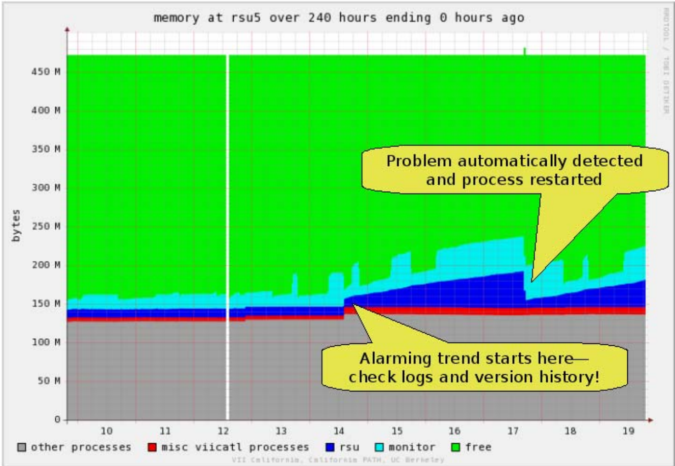
Figure 3.7 Graph of Memory Usage
