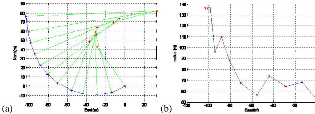
Figure 4.7 (a) Preliminary Curvature Estimates by CCS Algorithm (b) Preliminary Estimates of Curvature Radii by CCS Algorithm
