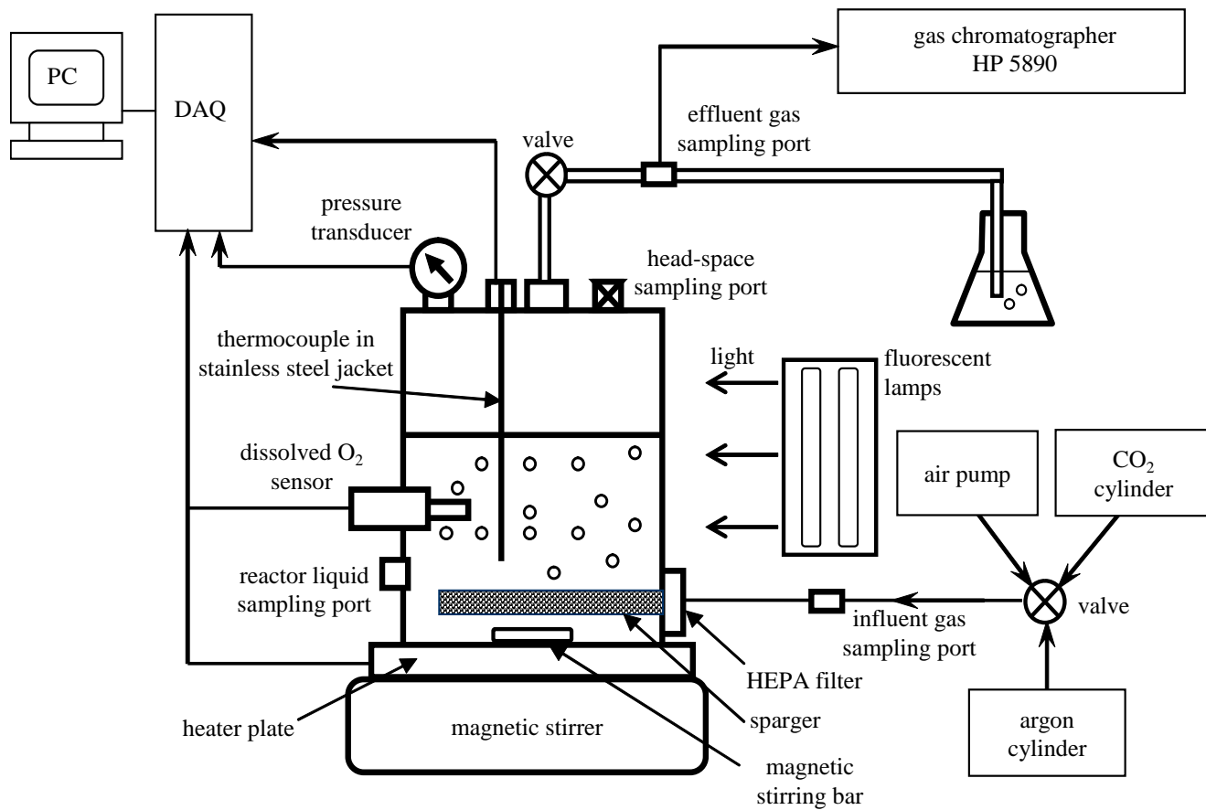
Figure 1: Schematic of the front view of the experimental setup and instrumentation.
