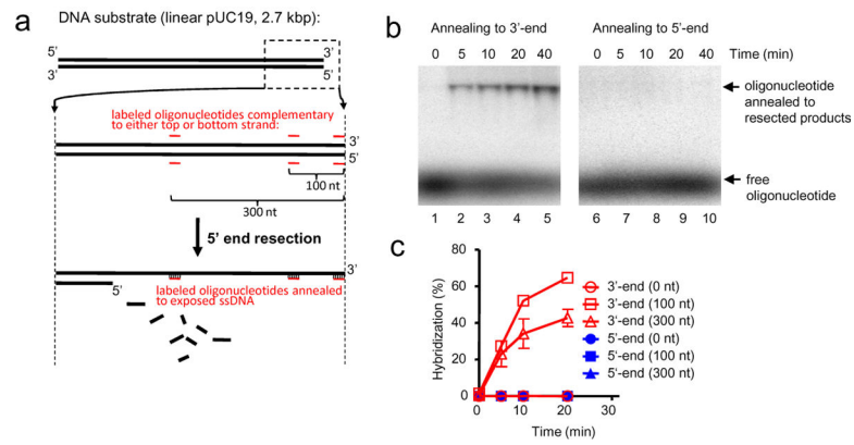
Figure 2. Sgs1, Dna2, and RPA preferentially resect the 5'-terminated strand of a DNA break a , Assay. b , Annealing of oligonucleotide to resection products (0.5 nM Sgs1, 0.5 nM Dna2, and 3 \mu M RPA) using probe complementary to either top (3'-) or bottom (5'-) strand, 300 nucleotides from end. c , Quantification of DNA end resection at various distances from DSB, based on experiments as shown in b .
