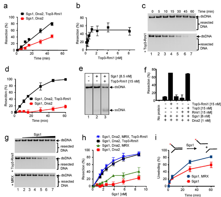
Figure 4. Top3-Rmi1 and MRX complexes stimulate DNA resection by Dna2-Sgs1-RPA a , Resection kinetics: Sgs1 (0.3 nM), Dna2 (1 nM), RPA (3 \mu M), and Top3-Rmi1 heterodimer (10 nM). b , Top3-Rmi1-dependent stimulation of DNA resection: Sgs1 (0.5 nM), Dna2 (0.5 nM) and RPA (3 \mu M). c , Resection kinetics in high salt buffer (5 mM Mg^{2+} and 100 mM Na^+ ): Sgs1 (7.5 nM), Dna2 (1 nM), RPA (3 \mu M), and Top3-Rmi1 heterodimer (15 nM). d , Quantification of experiments as in c . e , DNA unwinding in high salt buffer; RPA (3 \mu M). f , Resection in high salt buffer; RPA (3 \mu M). g , Stimulation of resection in high salt buffer by Top3-Rmi1 (15 nM) and MRX (20 nM) using Dna2 (1 nM), RPA (3 \mu M), Sgs1 (0, 1.3, 1.7, 2.5, 3.8, 5.7 and 8.6 nM). h , Quantification of experiments as in g . i , Unwinding of Y-structure DNA in high salt buffer: Sgs1 (200 pM); RPA (2.25 nM); and MRX (5 nM).
