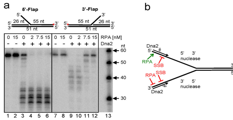
Figure 3. RPA promotes 5'→3' degradation by Dna2 and inhibits 3'→5' degradation a , Duplex DNA substrates containing either a 5'- or 3'-ssDNA flap (red asterisk indicates the 32 P-label) incubated with Dna2 (15 nM) and indicated RPA. b , Illustration summarizing results from panel a and Supplementary Figs. 4 and 5 showing modulation of ssDNA nuclease activities of Dna2.
