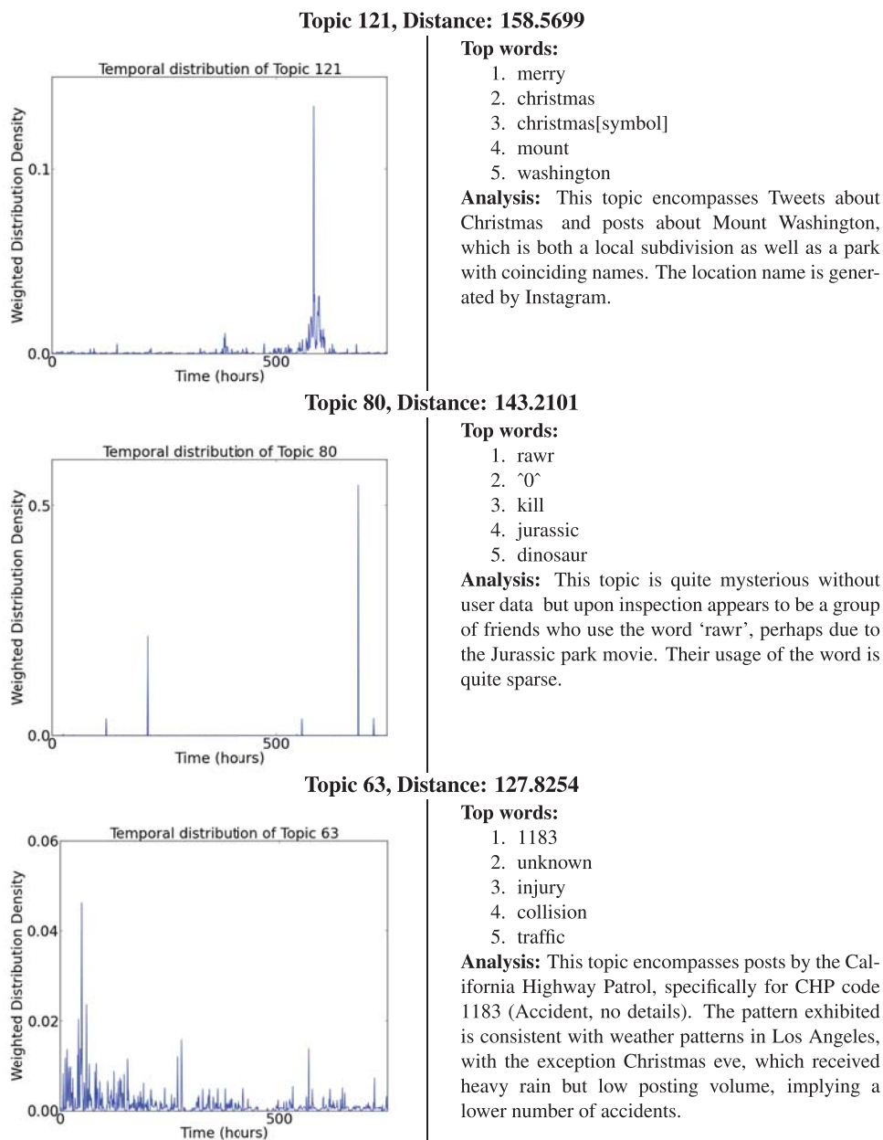
FIG. 2. Display of three of the 'furthest' topic temporal histograms from the Uniform weighting using the EMD. On the right of each section an interpretation of the topic is provided.
