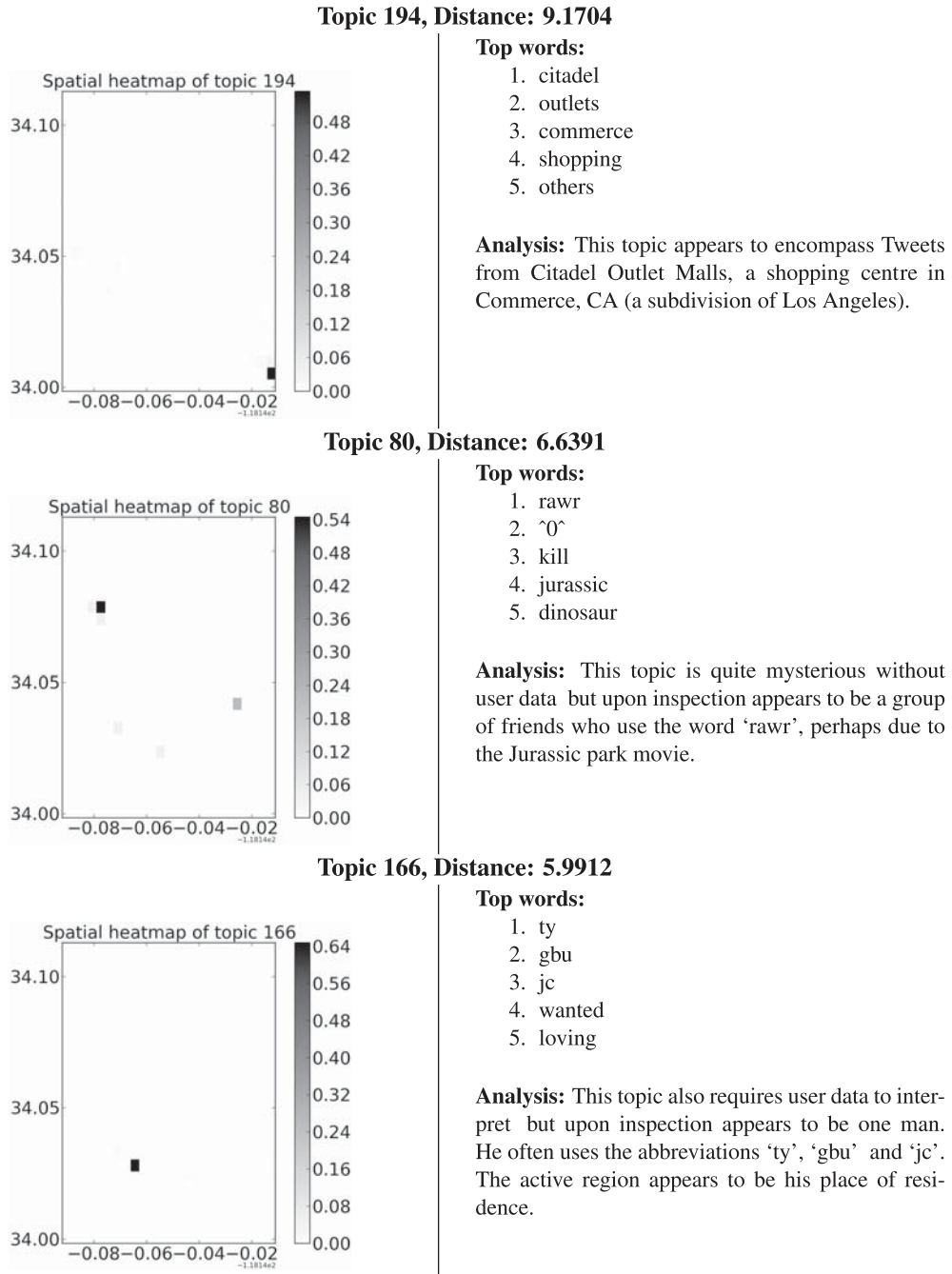
FIG. 4. We here display three of the 'furthest' topic spatial histograms from the Uniform weighting using the EMD. On the right of each section we provide an interpretation of the topic. The axes are longitude and latitude coordinates (the x -axis is relative to 118^\circ W).
