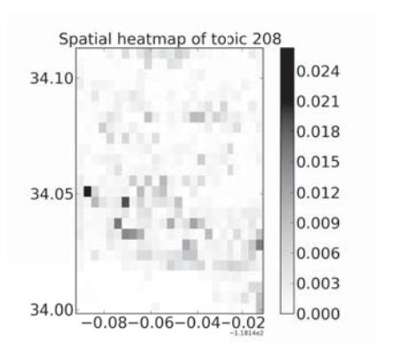
FIG. 5. Display of one 'far' topic spatial histograms and one 'close' topic spatial histogram, as measured by the EMD from the Uniform weighting. An interpretation of the topic is provided. The axes are longitude and latitude coordinates (the x -axis is relative to 118^\circ W).
