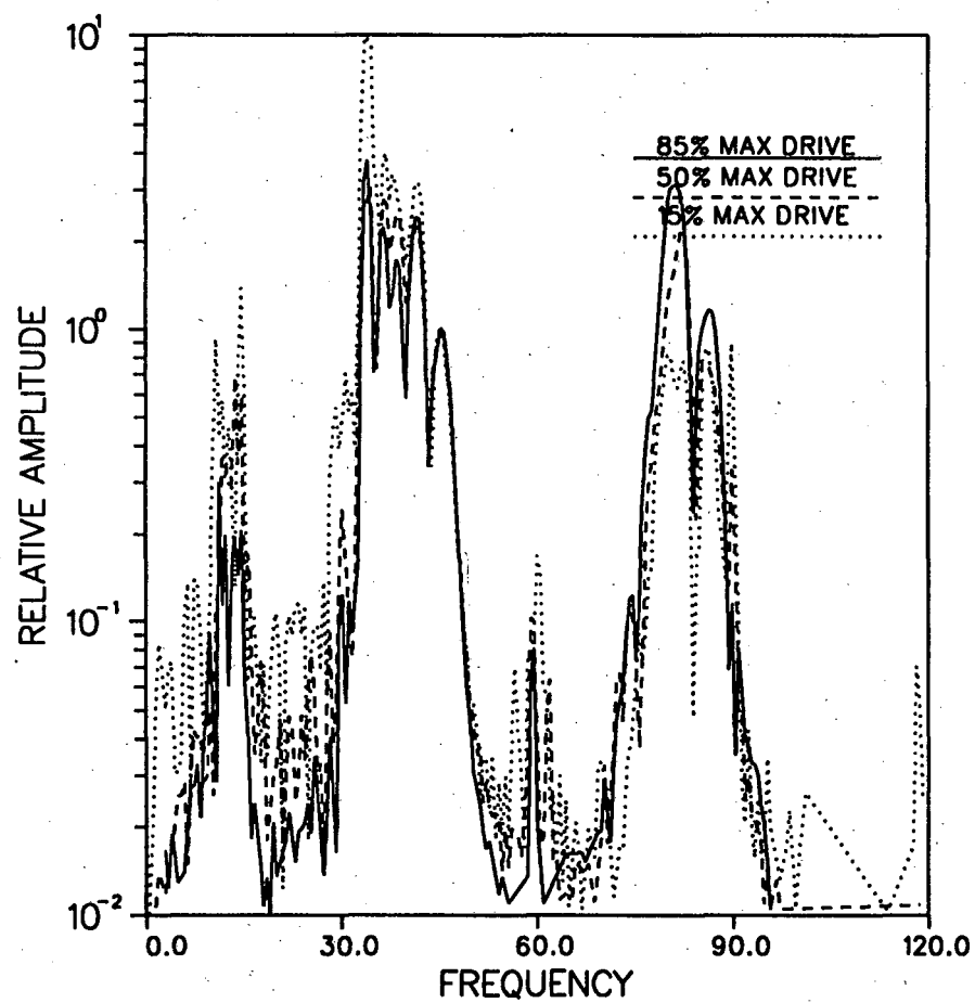
Figure 7i. NTS VSP data. Plots of spectral amplitude for the 45 Hz direct arrival at three drive levels (15%, 50% and 85%). The left side plot is for a 1200 ft source offset and the right side plot is for a 1400 ft source offset.
