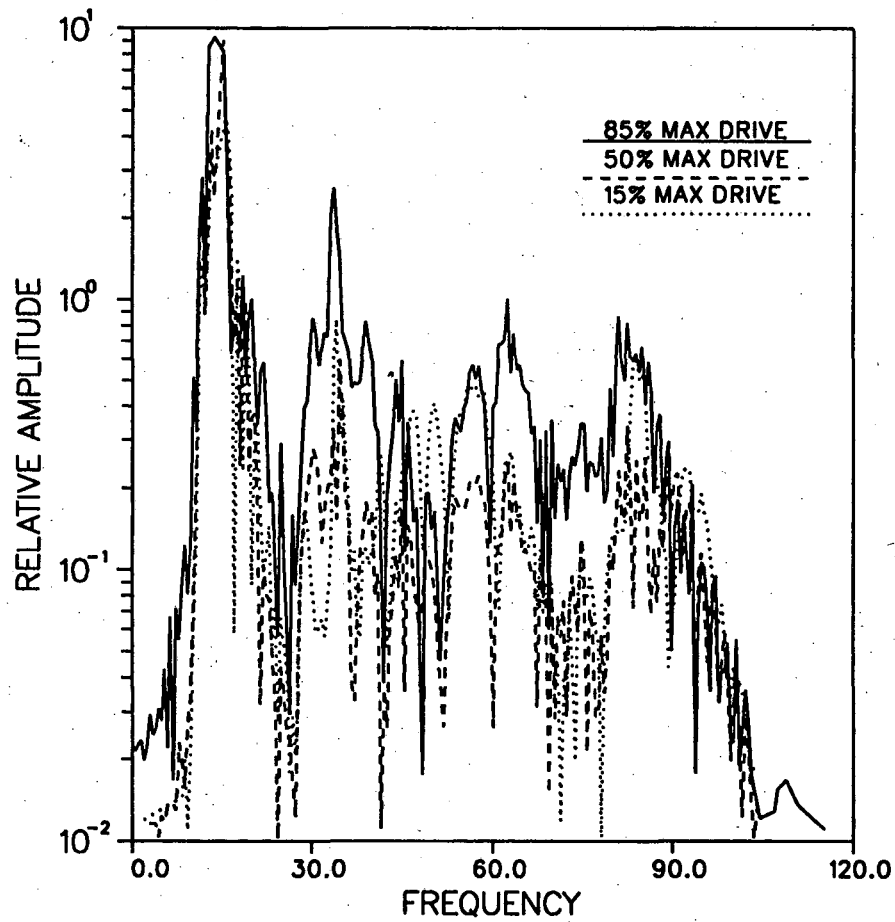
Figure 7a. NTS VSP data. Plots of spectral amplitude for the 20 Hz direct arrival at three drive levels (15%, 50% and 85%). The left side plot is for a 400 ft source offset and the right side plot is for a 600 ft source offset.
