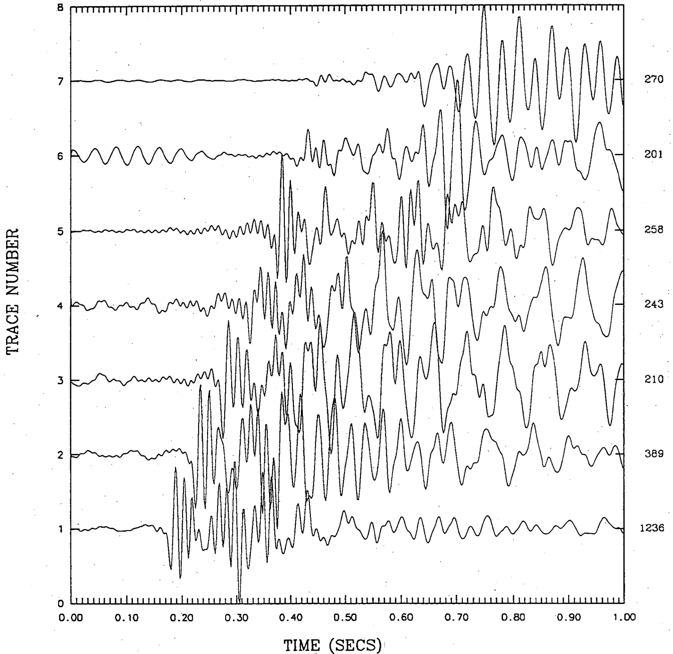
Figure 5a. Correlated data traces from the NTS walk-away VSP experiment. The vibrator was at 85% output. Traces 1 through 7 are, respectively, 400 to 1600 ft source offset at 200 ft increment. The traces are plotted with the maximum amplitude having the same height for each trace. The relative amplitudes are written at the end of each trace. The receiver was at 400 ft depth. Note the variation in waveform with increasing offset.
