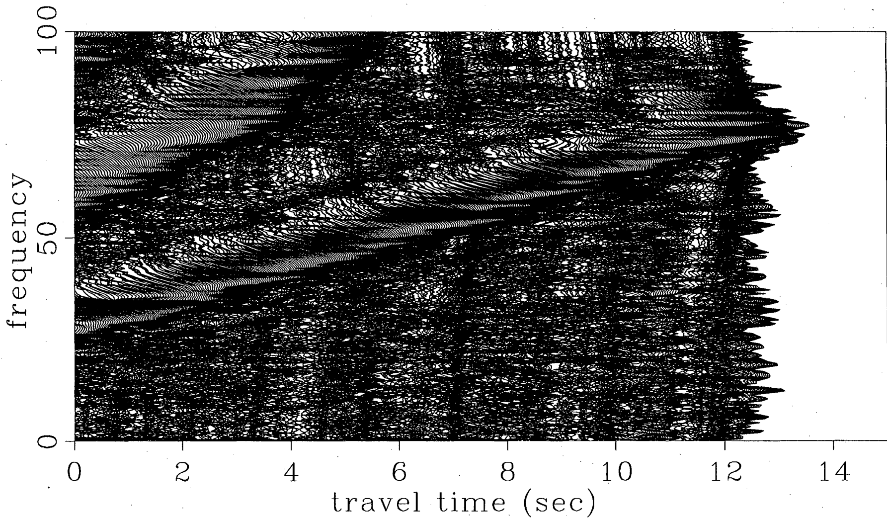
Figure 6. NTS VSP data. Plot of spectral amplitude versus time for the vertical component. A trace is plotted at each time step with the trace amplitude being the spectral amplitude for each frequency. The high amplitude peak from 0 to 12 sec increasing in frequency and time is the vibrator sweep, at higher frequency the first harmonic is seen from 0 to 5 sec where it leaves our analysis band.
