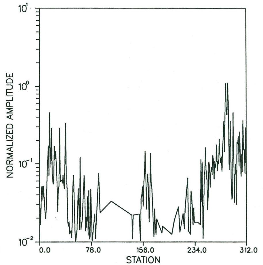
Figure 11b. Spectral amplitude ratio versus offset for third (left) and fourth (right) harmonic of the 23 Hz LANL data (Figure 8b). The station spacing is 110 ft. The source is at station 165.
