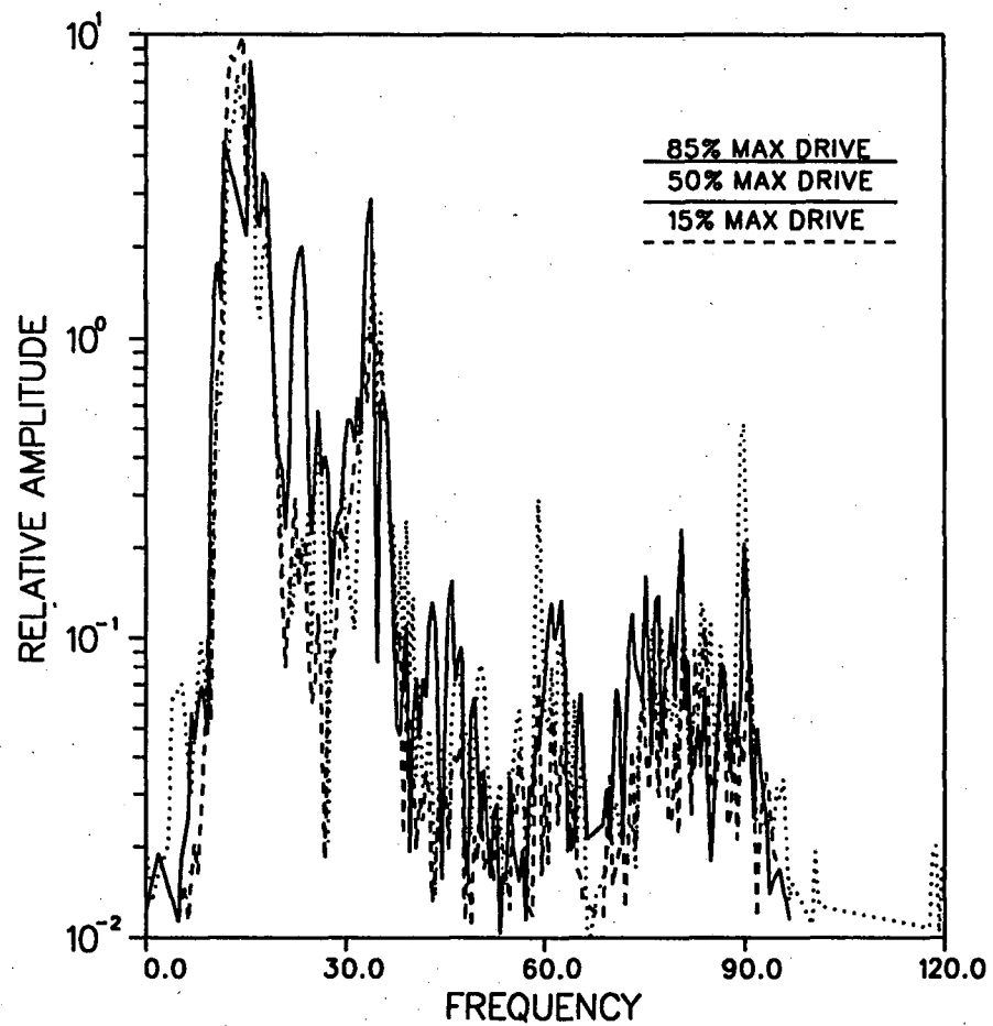
Figure 7b. NTS VSP data. Plots of spectral amplitude for the 20 Hz direct arrival at three drive levels (15%, 50% and 85%). The left side plot is for a 800 ft source offset and the right side plot is for a 1000 ft source offset.
