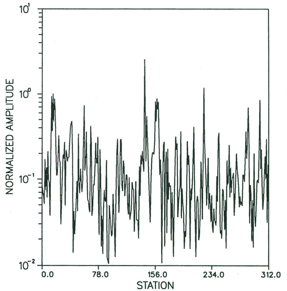
Figure 12. Spectral amplitude ratio versus offset using 12 seconds of LANL data. Left side is first harmonic of 13 Hz, right side is first harmonic of 23 Hz data. The station spacing is 110 ft. The source is at station 165. LANL.
