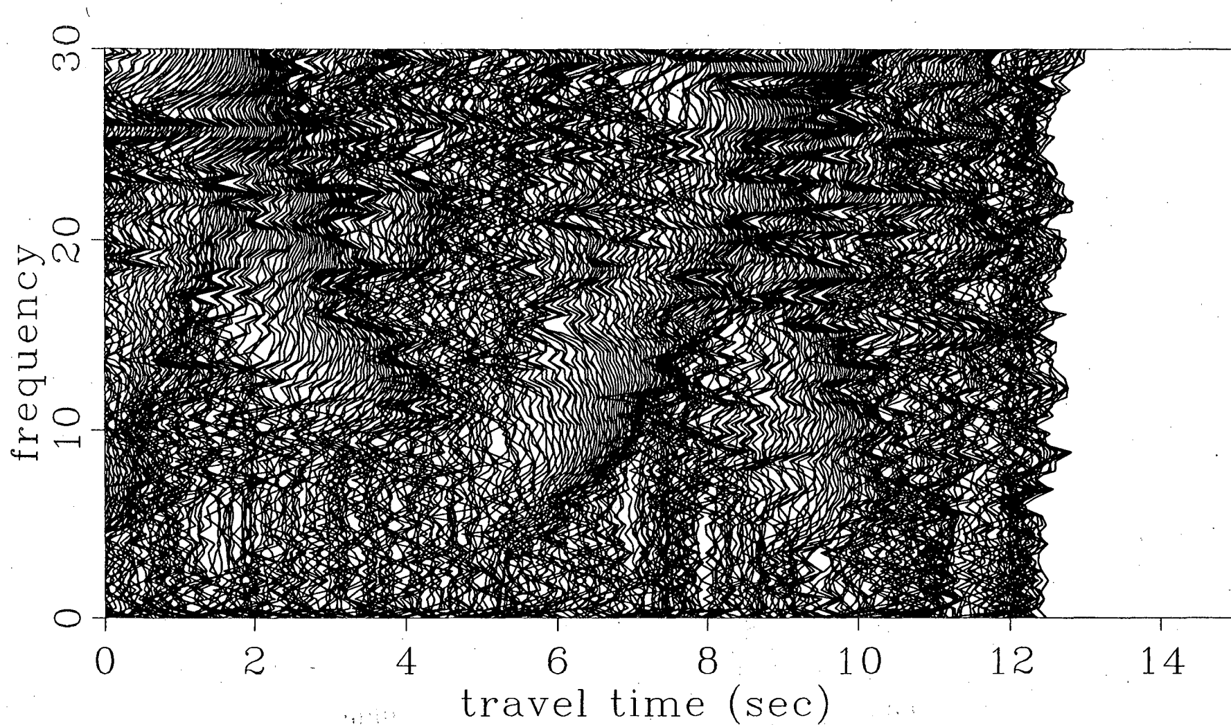
Figure 19b. Frequency vs time decomposition of the data in Figure 19a for 0 to 30 Hz. Amplitudes in db. The subharmonics below the crossing sweeps are evident in this bandwidth.
