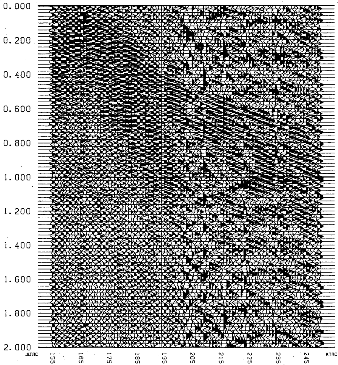
Figure 20. Crossing sweep LANL data correlated with the difference sweep, 40 to 0 to 40 Hz (actual sweep was -40 to 40 Hz). The first P-wave arrival can be clearly seen, and possible reflections are at later times.
