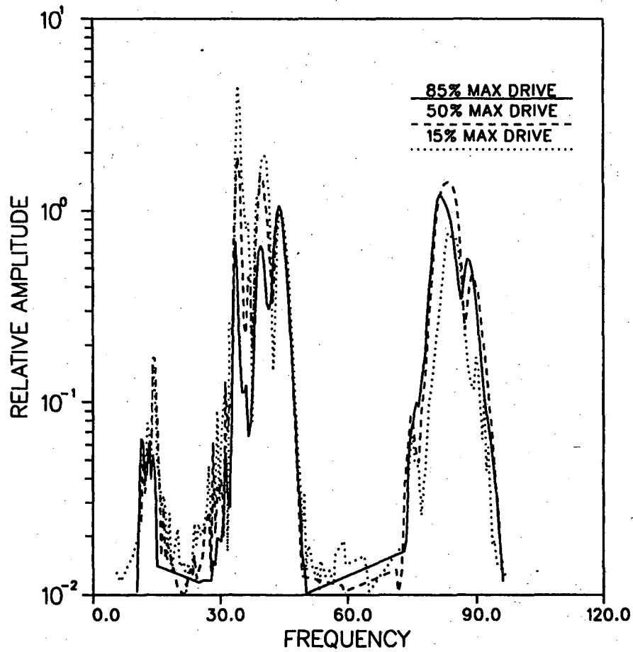
Figure 7g. NTS VSP data. Plots of spectral amplitude for the 45 Hz direct arrival at three drive levels (15%, 50% and 85%). The left side plot is for a 400 ft source offset and the right side plot is for a 600 ft source offset.
