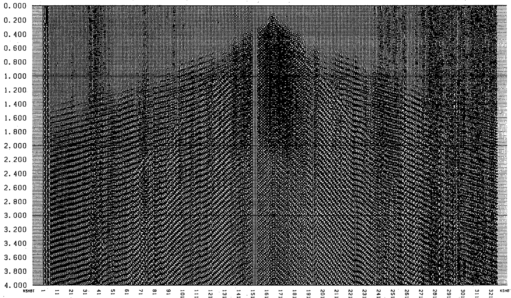
Figure 8a. Data traces from LANL experiment showing one shot gather for three vibrators shaking at 13 Hz. Note the P-wave and surface wave arrivals.
