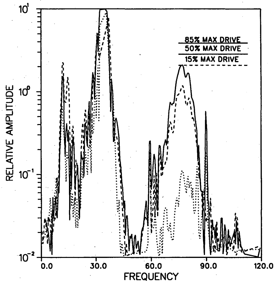
Figure 7e. NTS VSP data. Plots of spectral amplitude for the 40 Hz direct arrival at three drive levels (15%, 50% and 85%). The left side plot is for a 800 ft source offset and the right side plot is for a 1000 ft source offset.
