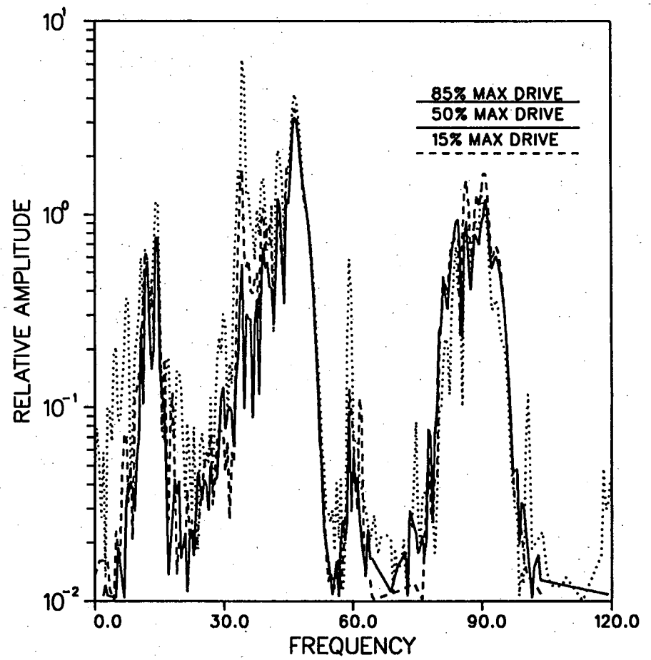
Figure 7k. NTS VSP data. Plots of spectral amplitude for the 50 Hz direct arrival at three drive levels (15%, 50% and 85%). The left side plot is for a 800 ft source offset and the right side plot is for a 1000 ft source offset.
