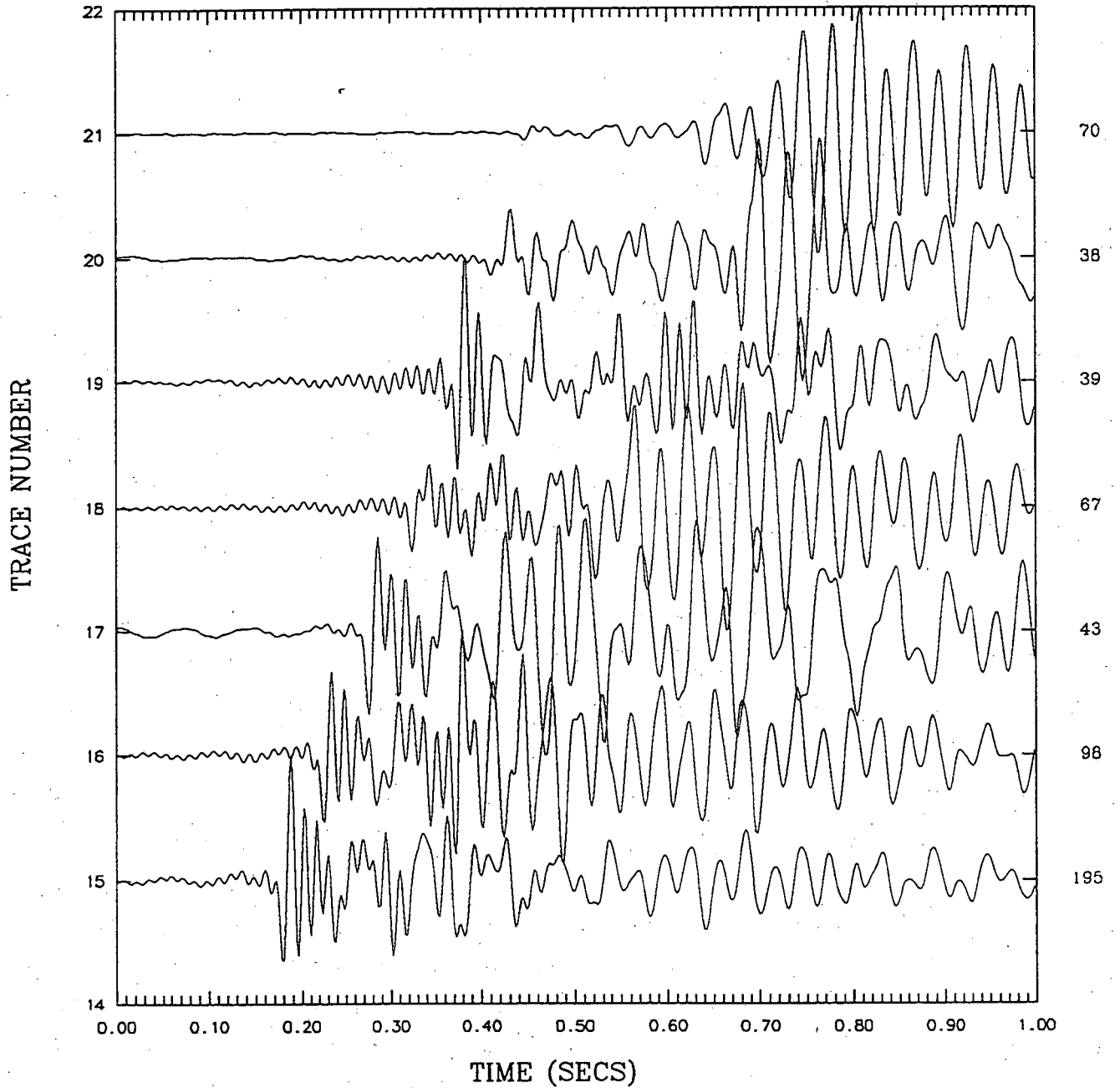
Figure 5c. Correlated data traces from the NTS walk-away VSP experiment. The vibrator was at 15% output. Traces 15 through 21 are 400 ft to 1600 ft source offset at 200 ft increment. The traces are plotted with the maximum amplitude having the same height for each trace. The relative amplitudes are written at the end of each trace. The receiver was at 400 ft depth. Note the variation in waveform with increasing offset. By comparing 5a, 5b and 5c, we see that source location has a larger effect on waveform than source strength.
