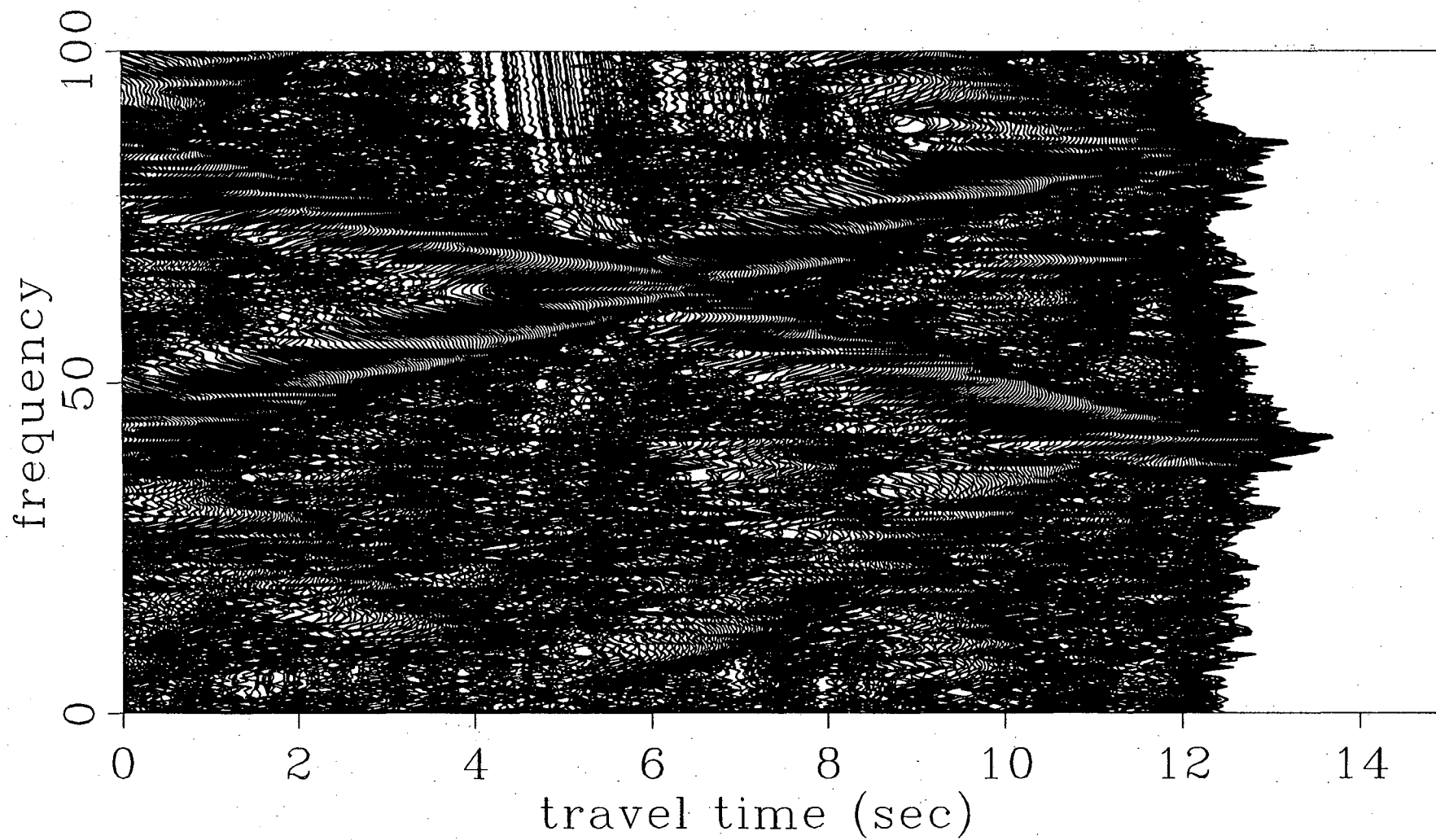
Figure 19a. Frequency vs time decomposition of a horizontal component for the NTS crossing sweep data 0 to 100 Hz. Amplitudes in db.
