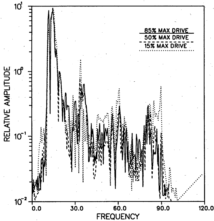
Figure 7c. NTS VSP data. Plots of spectral amplitude for the 20 Hz direct arrival at three drive levels (15%, 50% and 85%). The left side plot is for a 1200 ft source offset and the right side plot is for a 1400 ft source offset.
