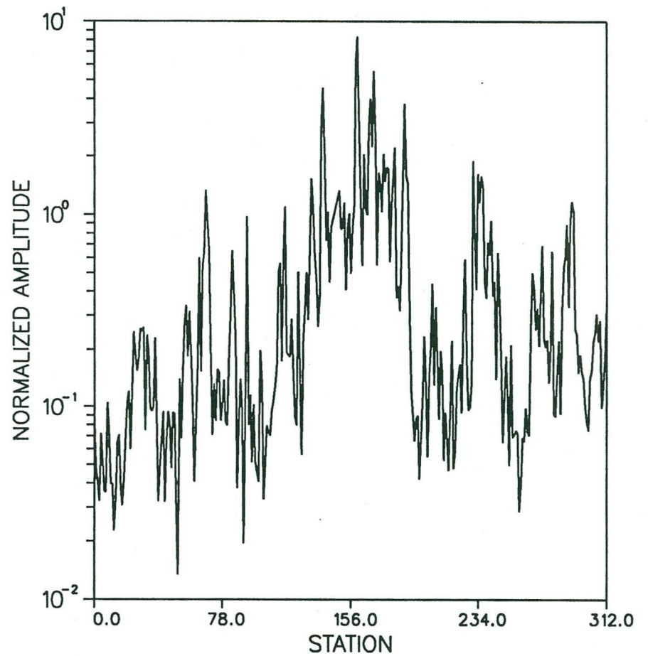
Figure 10a. Spectral amplitude ratio versus offset for first (left) and second (right) harmonic of the 13 Hz LANL data (Figure 8a). The station spacing is 110 ft. The source is at station 165.
