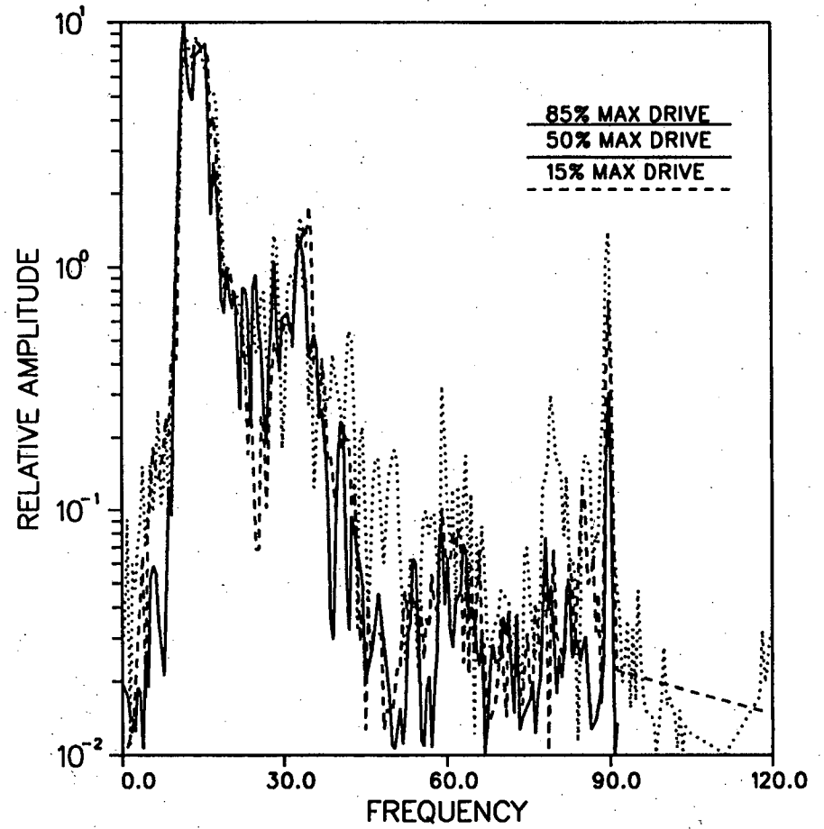
Figure 7c. NTS VSP data. Plots of spectral amplitude for the 20 Hz direct arrival at three drive levels (15%, 50% and 85%). The left side plot is for a 1200 ft source offset and the right side plot is for a 1400 ft source offset.
