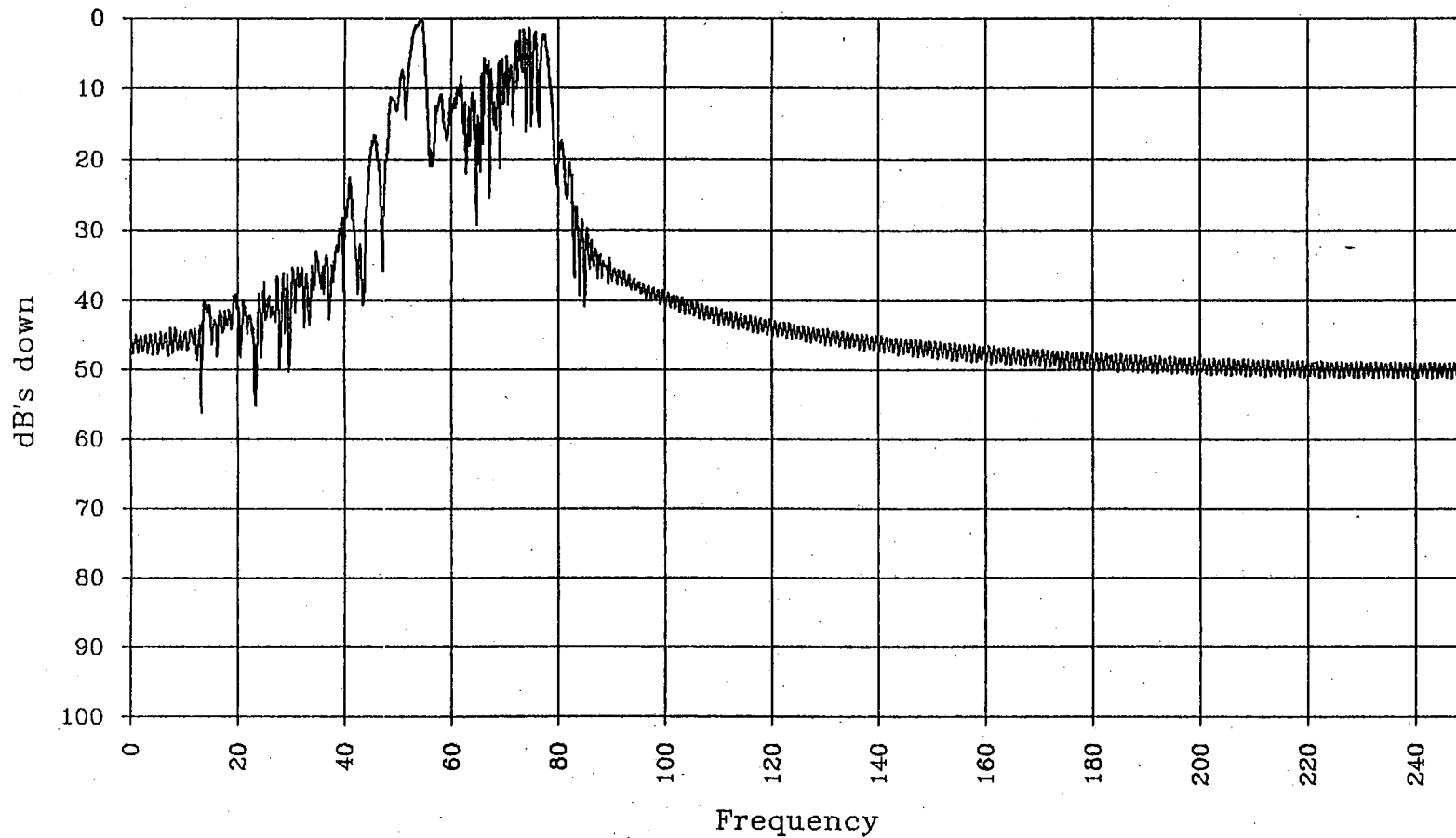
Figure 17a. Spectra for the vertical component of the NTS dual sweep experiment with a stack of 10 sweeps. While the most energy is from 50 to 80 Hz, there is a peak at ~15 Hz.
