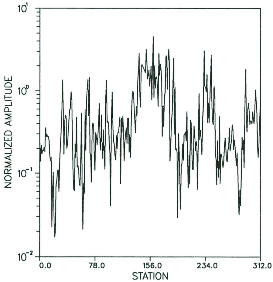
Figure 12. Spectral amplitude ratio versus offset using 12 seconds of LANL data. Left side is first harmonic of 13 Hz, right side is first harmonic of 23 Hz data. The station spacing is 110 ft. The source is at station 165. LANL.
