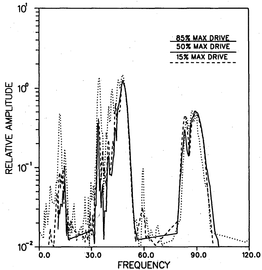
Figure 7j. NTS VSP data. Plots of spectral amplitude for the 50 Hz direct arrival at three drive levels (15%, 50% and 85%). The left side plot is for a 400 ft source offset and the right side plot is for a 600 ft source offset.
