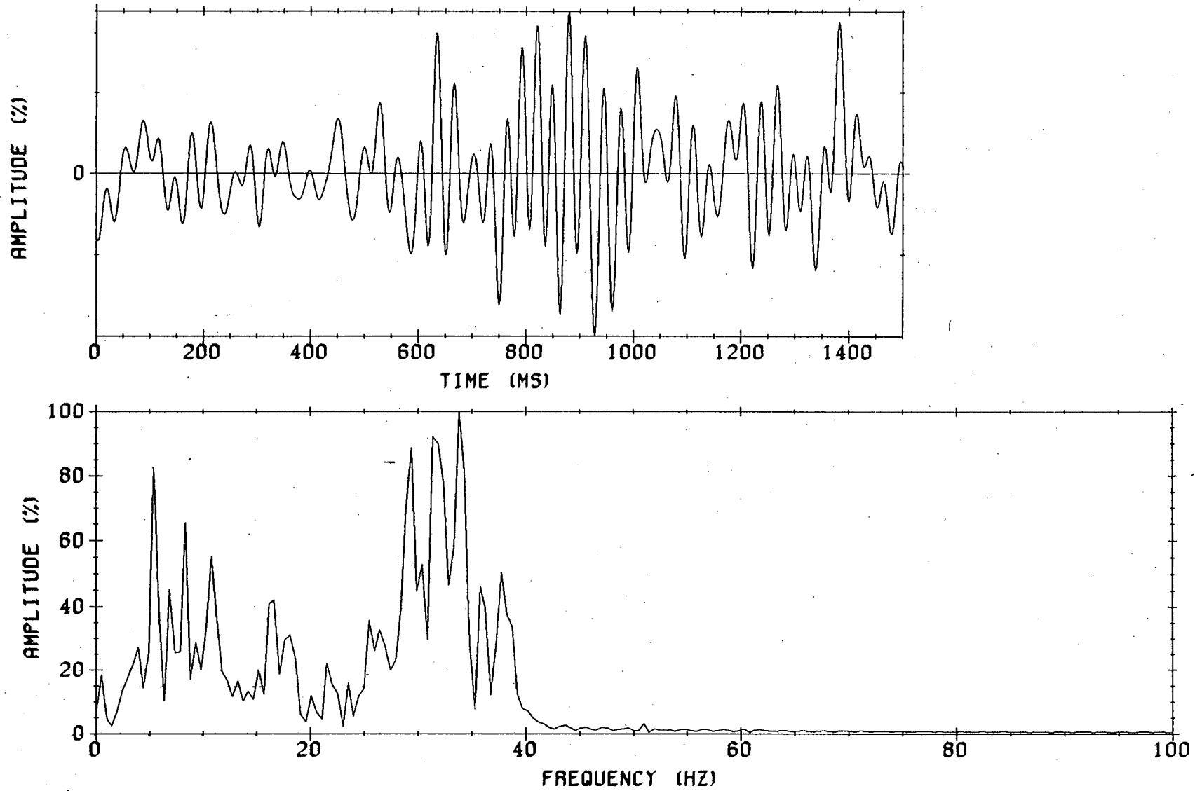
Figure 21. Time series (top) and spectra (bottom) for one trace from the data in Figure 20. The main energy is from 25 to 40 Hz, although there is measurable energy below 10 Hz.
