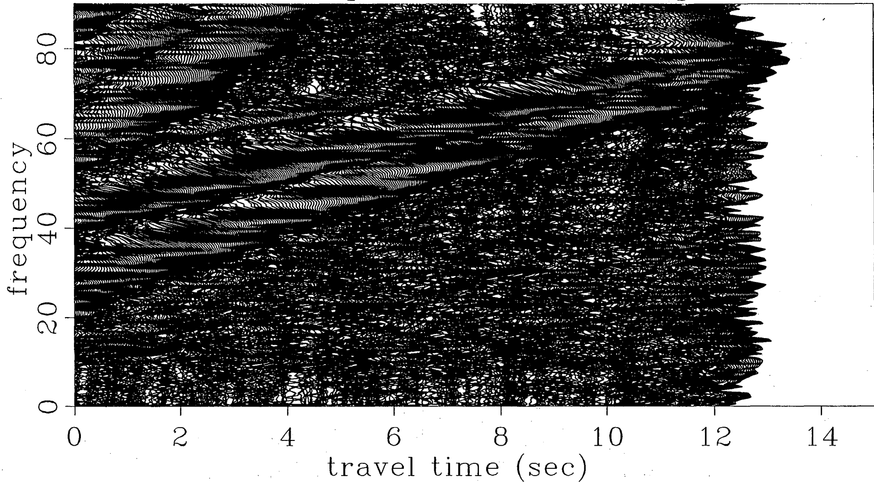
Figure 17c. Frequency vs time decomposition of horizontal component for the NTS dual upsweep data. Amplitude in db. The two upsweeps, 25 to 76 Hz and 40 to 79 Hz, can be seen.
