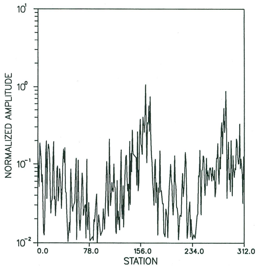
Figure 11a. Spectral amplitude ratio versus offset for first (left) and second (right) harmonic of the 23 Hz LANL data (Figure 8b). The station spacing is 110 ft. The source is at station 165.
