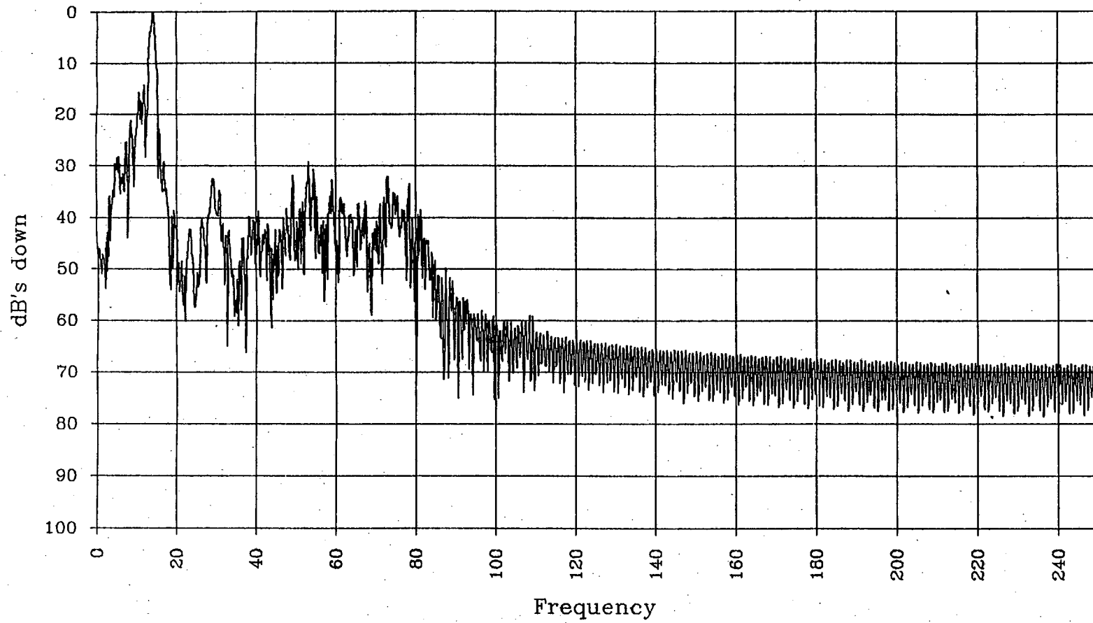
Figure 17b. Same data as 17a, but with a 3 to 15 Hz bandpass filter applied. We see a peak at about 14 Hz.
