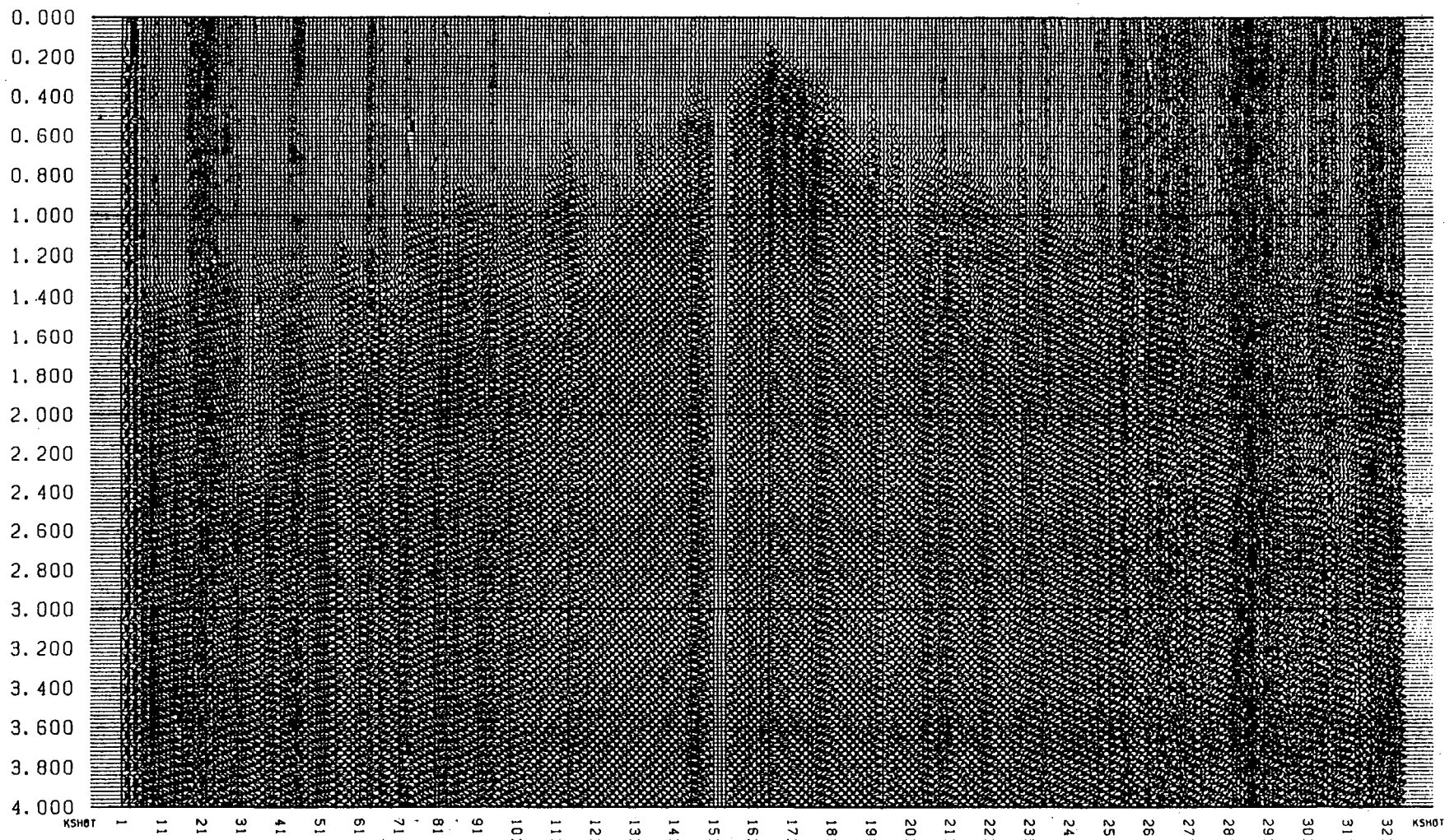
Figure 8b. Same as Figure 8a, with vibrators shaking at 23 Hz.
