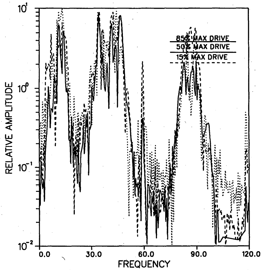
Figure 71. NTS VSP data. Plots of spectral amplitude for the 50 Hz direct arrival at three drive levels (15%, 50% and 85%). The left side plot is for a 1200 ft source offset and the right side plot is for a 1400 ft source offset.
