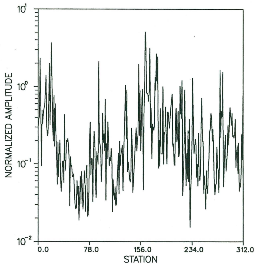
Figure 14. LANL data. Spectral amplitude ratio versus offset for the first harmonic of 31 Hz data (left) and 43 Hz data (right). The station spacing is 110 ft. The source is at station 165.
