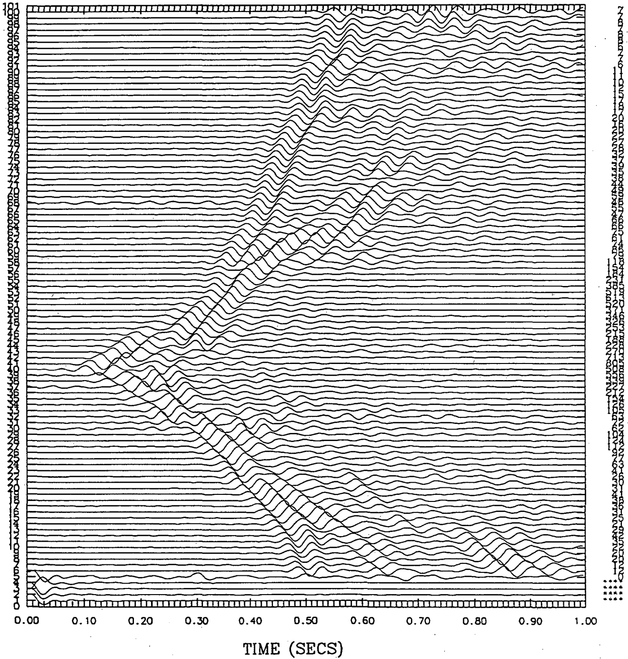
Figure 1. Correlated data traces from the Tehachapi Mountains seismic reflection profile. Each trace is plotted such that its maximum amplitude is one trace spacing. The relative maximum amplitude is printed at the end of each trace. The first 5 traces are not data.
