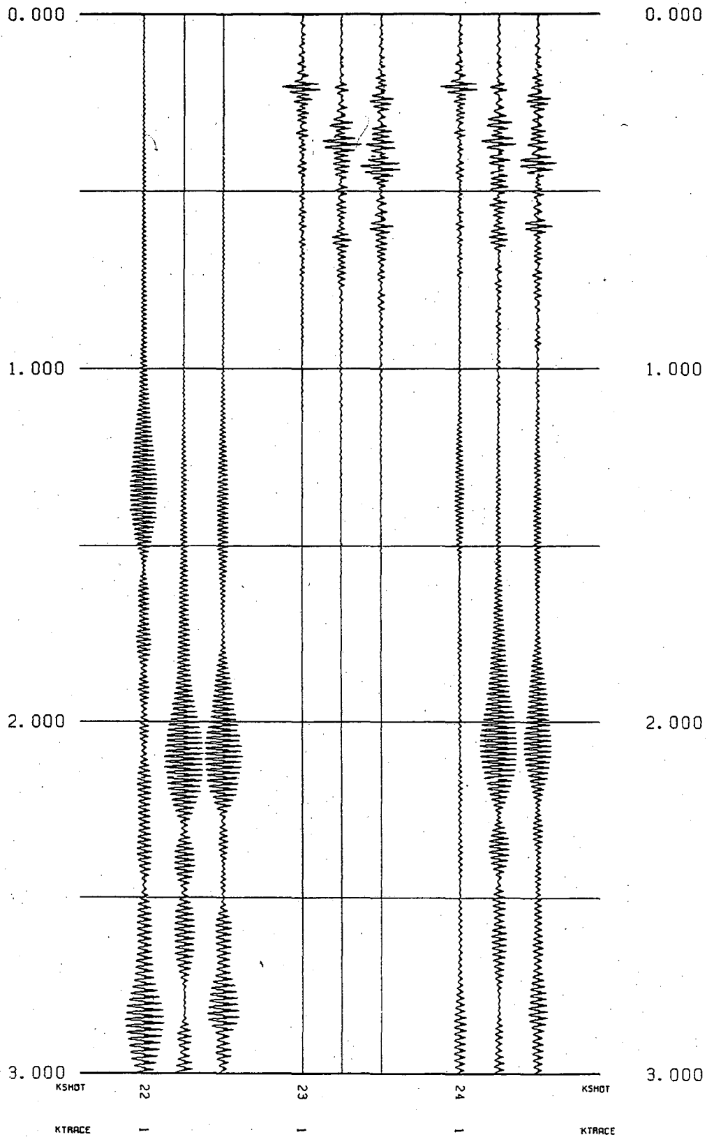
Figure 18b. Dual sweep NTS data correlated with a 40 to 79 Hz sweep. The three sets of three-component data had, left to right, a source with 25 to 75 Hz sweep, a source with 40 to 79 Hz sweep, and both sources simultaneously.
