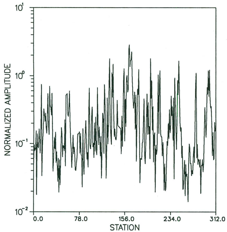
Figure 14. LANL data. Spectral amplitude ratio versus offset for the first harmonic of 31 Hz data (left) and 43 Hz data (right). The station spacing is 110 ft. The source is at station 165.
