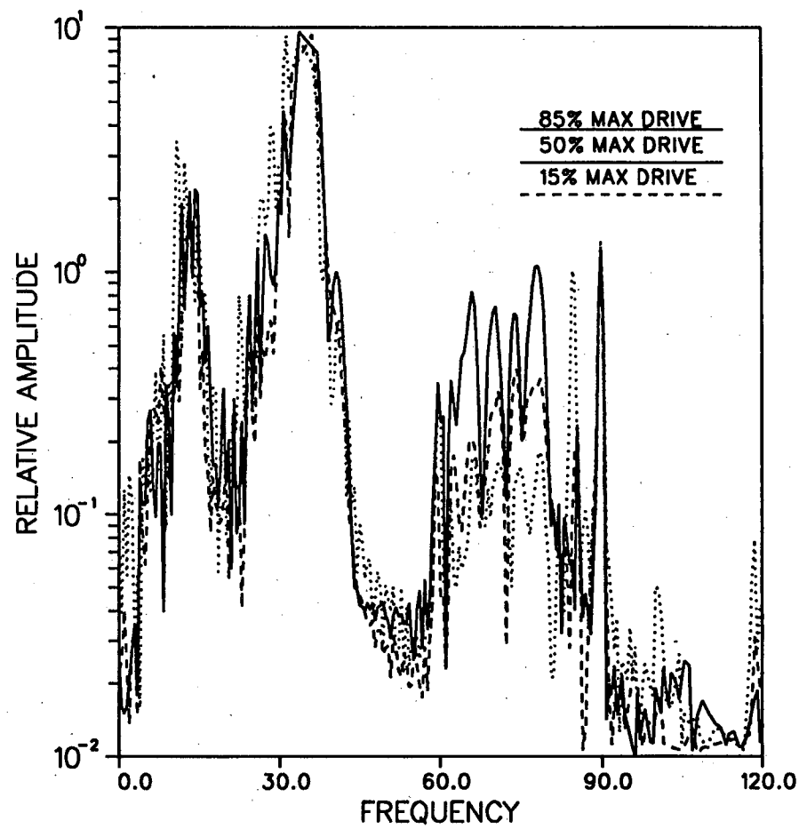
Figure 7f. NTS VSP data. Plots of spectral amplitude for the 40 Hz direct arrival at three drive levels (15%, 50% and 85%). The left side plot is for a 1200 ft source offset and the right side plot is for a 1400 ft source offset.
