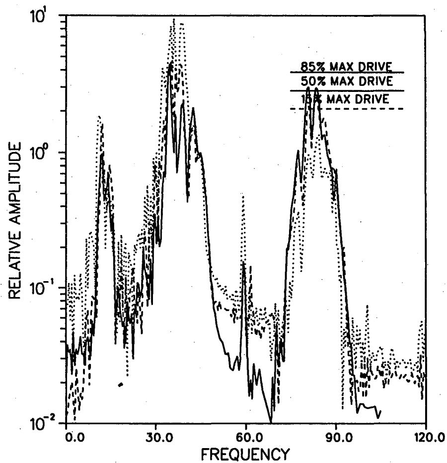
Figure 7h. NTS VSP data. Plots of spectral amplitude for the 45 Hz direct arrival at three drive levels (15%, 50% and 85%). The left side plot is for a 800 ft source offset and the right side plot is for a 1000 ft source offset.
