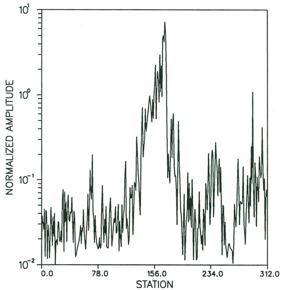
Figure 10b. Spectral amplitude ratio versus offset for third (left) and fourth (right) harmonic of the 13 Hz LANL data (Figure 8a). The station spacing is 110 ft. The source is at station 165.
