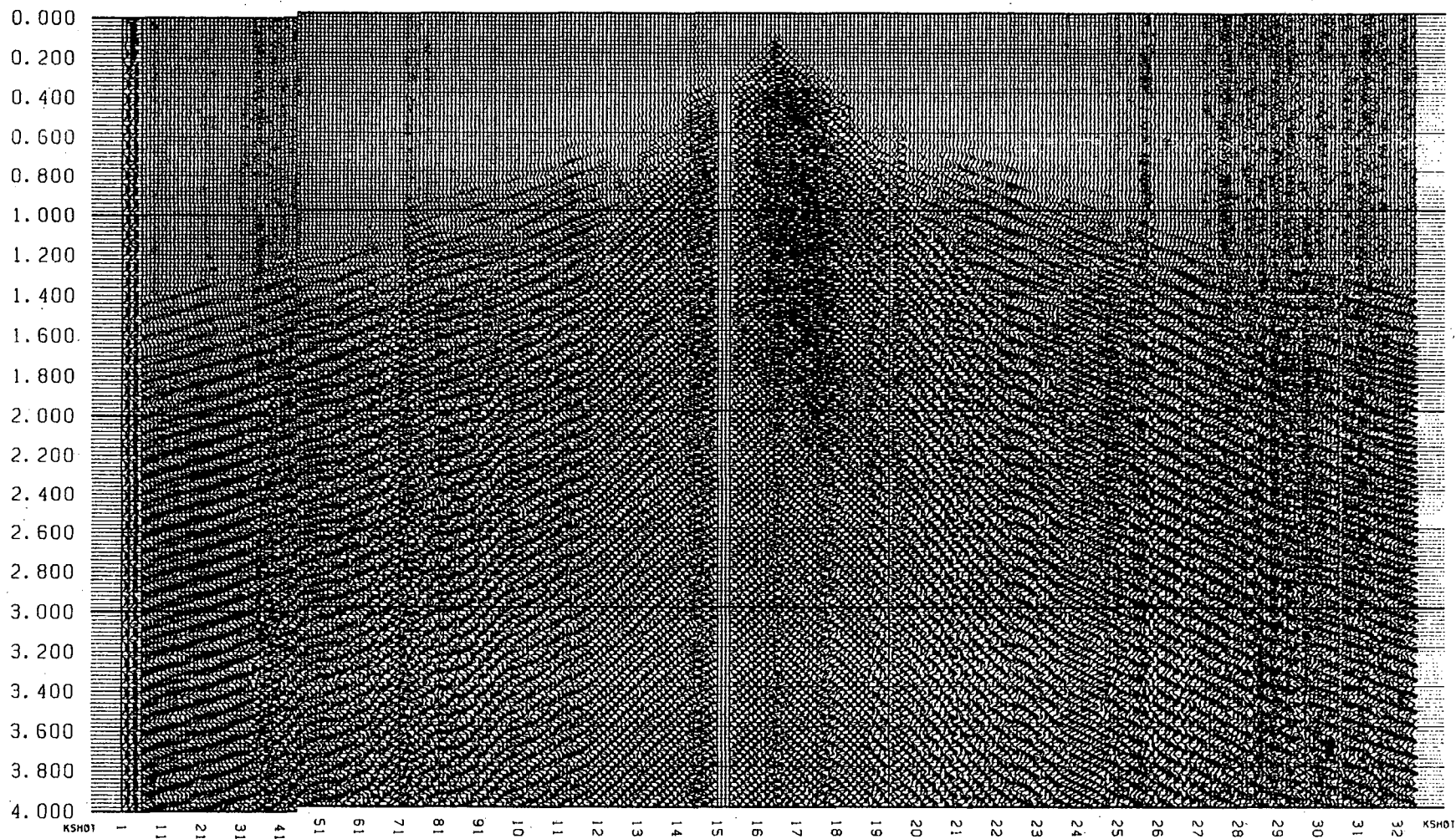
Figure 8c. Data traces from LANL experiment showing a shot gather for simultaneous sweeping of 13 Hz and 23 Hz by three vibrators each.
