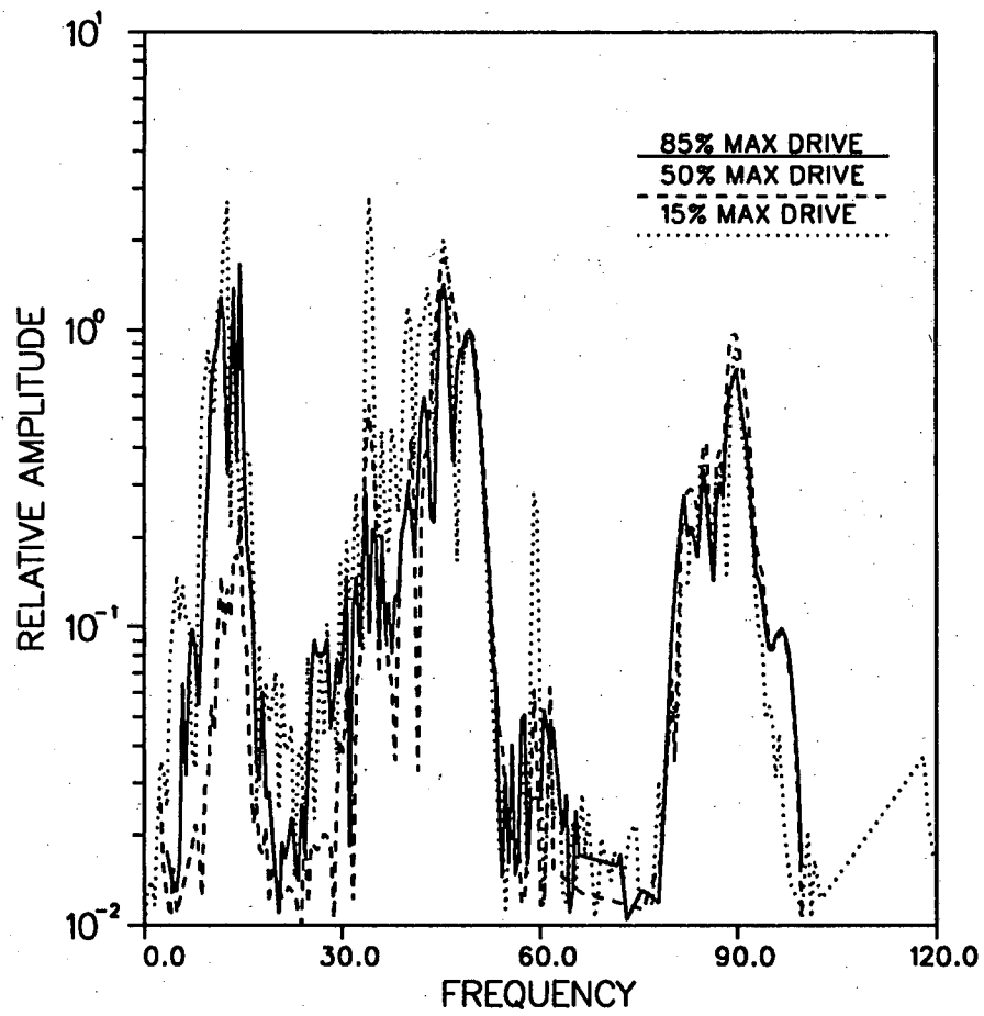
Figure 7k. NTS VSP data. Plots of spectral amplitude for the 50 Hz direct arrival at three drive levels (15%, 50% and 85%). The left side plot is for a 800 ft source offset and the right side plot is for a 1000 ft source offset.
