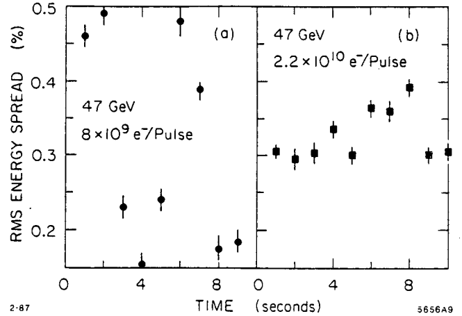
Fig. 8. Measurement of the energy width, \sigma_E/E , as a function of time for two different Linac intensities.
