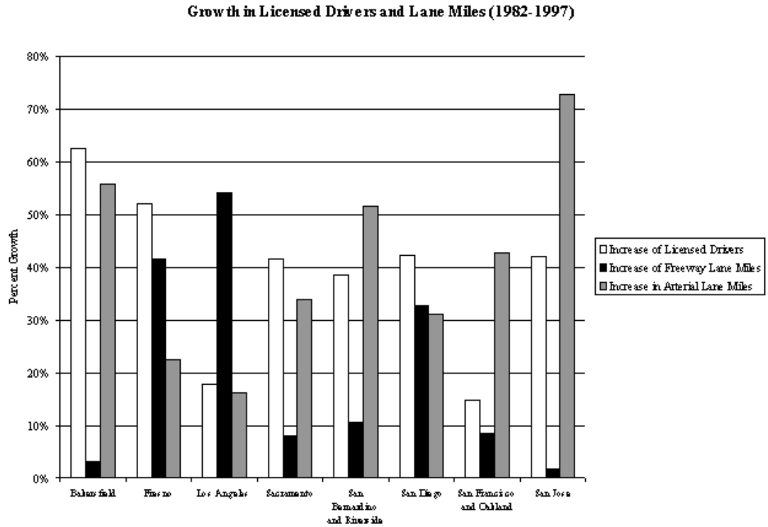
Figure 6b - Growth in Drivers Compared to Increases in Highway and Arterial Capacity
