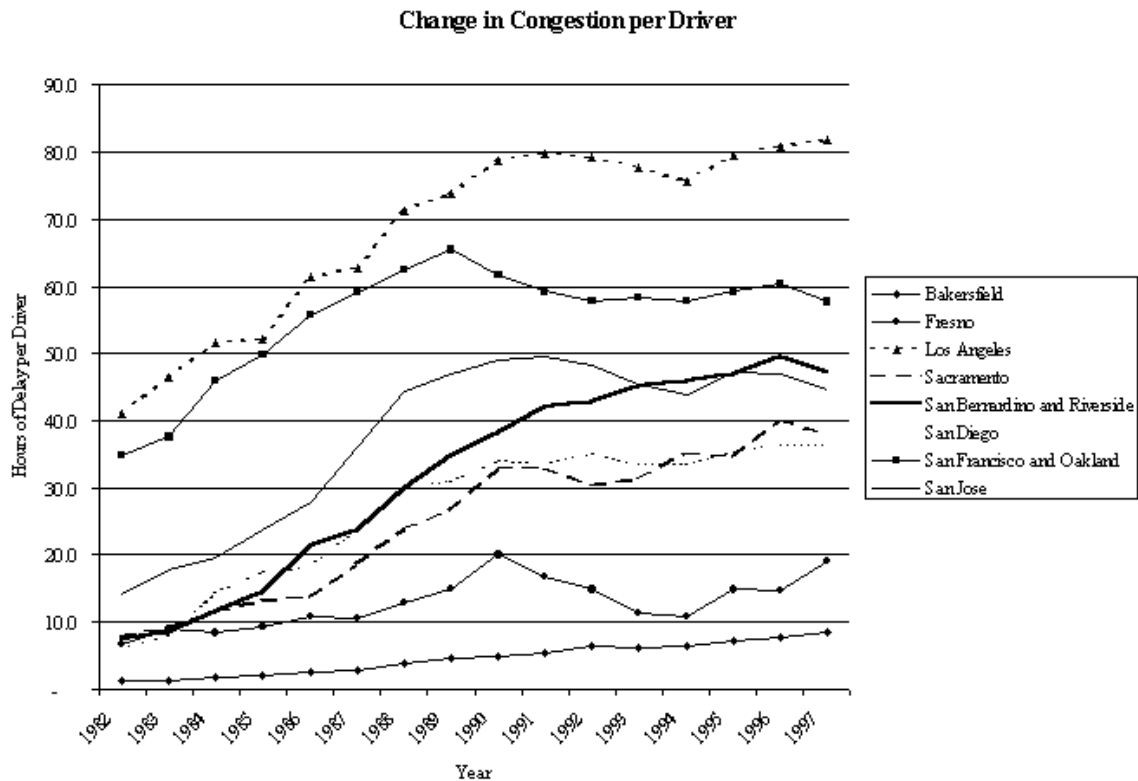
Figure 8b - Change in Traffic Delay Measured Per Driver
