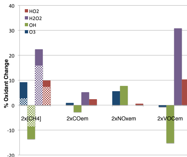
Figure A1. Sensitivity of oxidant concentrations to a doubling in [\text{CH}_4] or emissions of \text{CO} , \text{NO}_x , or \text{VOCs} relative to a simulation of preindustrial oxidant chemistry (Sofen et al., 2011). Each bar represents the fractional change in Southern Hemisphere extratropical lower tropospheric ( \leq 2 km) oxidant concentration. The checkered segment of the \text{CH}_4 sensitivity study indicates the fraction of the oxidant changes for which \text{CH}_4 -derived \text{CO} is responsible.
