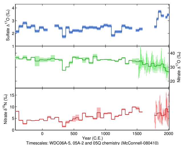
Figure 2. Measurements of \Delta^{17}\text{O}(\text{SO}_4^{2-}) , \Delta^{17}\text{O}(\text{NO}_3^-) , and \delta^{15}\text{N}(\text{NO}_3^-) in the upper 577 m of the WAIS Divide ice core. Each horizontal line segment indicates the time interval of that sample. Shading indicates the measurement uncertainty based on the replicate analysis of standards ( \Delta^{17}\text{O}(\text{SO}_4^{2-}) ) or replicate sample measurements ( \Delta^{17}\text{O}(\text{NO}_3^-) , \delta^{15}\text{N}(\text{NO}_3^-) ). The recent part of the nitrate isotope records are measured at 1 m resolution (see Fig. 4 for an expanded version of this record); the 1 m resolution measurements and their analytical uncertainty are shown in thin lines and shading and the thick lines through this portion of the \Delta^{17}\text{O}(\text{NO}_3^-) and \delta^{15}\text{N}(\text{NO}_3^-) indicate the concentration-weighted isotopic values at the resolution of the \Delta^{17}\text{O}(\text{SO}_4^{2-}) .
