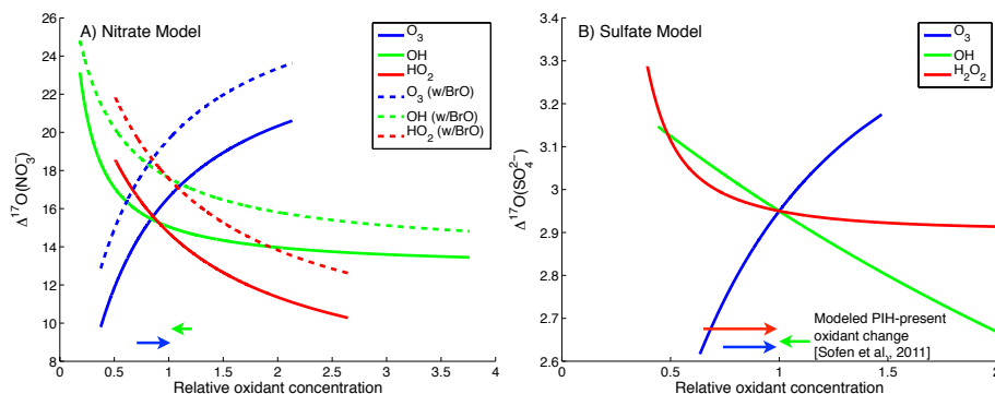
Figure 5. Sensitivity of (A) \Delta^{17}\text{O}(\text{NO}_3^-) and (B) \Delta^{17}\text{O}(\text{SO}_4^{2-}) to variations in each oxidant, normalized to the mean oxidant concentrations ( = 1.0 ) of the present-day South American and Southern Ocean boundary layers, respectively. Dashed lines indicate results when 1 \text{ pmol mol}^{-1} BrO is included as both an oxidant of NO in \text{NO}_x cycling and as an oxidant of \text{NO}_2 , which leads to nitrate formation via the hydrolysis of \text{BrONO}_2 . Arrows at the bottom indicate the fractional change in oxidant abundances over the Southern Ocean between preindustrial Holocene and present-day chemical transport model simulations (Sofen et al., 2011) for reference.
