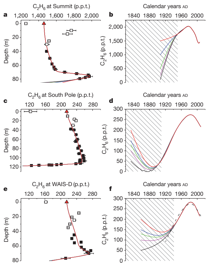
Figure 1 | Ethane mixing ratios in firn air at three sites, and the atmospheric histories derived from these measurements. a–f , Results for Summit ( a, b ), South Pole ( c, d ) and WAIS-D ( e, f ). Filled and open squares in a, c and e show measurements with estimated uncertainties (error bars, \pm 2 s.e.) (Supplementary Data). Solid lines in a, c and e show modelled firn profiles for the three respective sites, with the five different atmospheric histories (solid lines) shown in b, d and f . These five atmospheric histories were obtained by inverse modelling of the measurements with five different boundary conditions at t_0 that are identified by different colours, each representing a different pre-industrial mixing ratio for ethane. The data points in the top 35 m (Summit and South Pole) and 40 m (WAIS-D) of the firn are subject to the effects of seasonal variations in surface ethane levels (Supplementary Information) and are ignored during inverse modelling (open squares in a, c and e ). The inversions were forced with contemporary annual-mean surface mixing ratios of 1,460 p.p.t. at Summit and 215 p.p.t. at South Pole and WAIS-D (red triangles in a, c and e ) (Supplementary Information). The South Pole atmospheric history is overlaid on the independently derived WAIS-D atmospheric histories for comparison (dashed line in f ). The inversions are sensitive to assumptions about the pre-industrial ethane levels before 1950, 1940 and 1910 at Summit, WAIS-D and South Pole, respectively (shaded areas), implying that only the inversion results for the later years are valid atmospheric histories.
