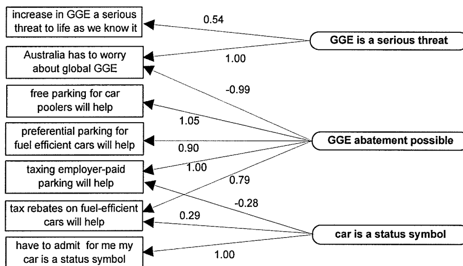
Figure 11: Flow Diagram of the Measurement Submodel Factors
