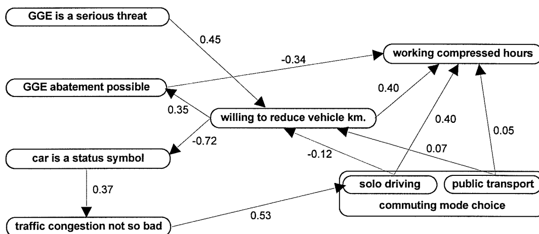
Figure 12: Flow Diagram of the Causal structure of the Endogenous Variables
