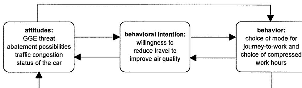
Figure 1: Conceptual Flow Diagram of Causal Influences
