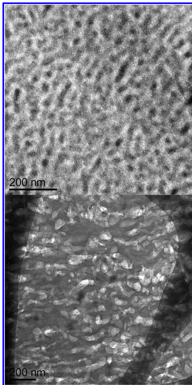
Figure 5. Transmission electron microscopy (TEM) images for (a) dry PSS-PE membrane and (b) hydrated PSS-PE quenched after equilibration in liquid water at T = 25 °C. In the dry sample, the PSS phase is dark. In the hydrated sample, the water-swollen PSS phase appears bright. Both samples (unstained) appear to have a disordered cylindrical morphology, although the cylinders in the hydrated membrane appear to be more extended.
