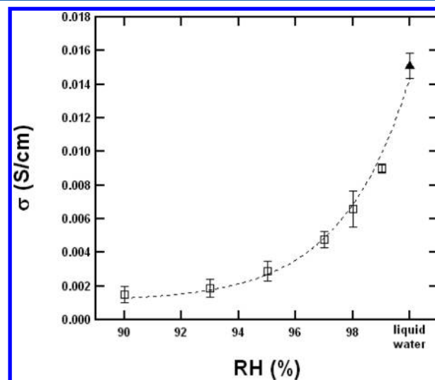
Figure 8. Proton conductivity, \sigma , of PSS-PE in humid vapor ( \square ) and liquid water ( \blacktriangle ) plotted as a function of relative humidity, RH, at T = 25 °C. Humid vapor data were obtained after equilibration in liquid water. The dashed curve represents a power-law fit through the humid vapor data.
