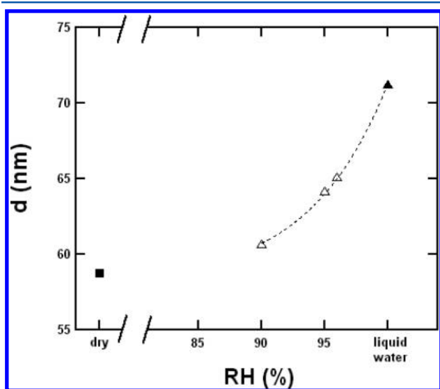
Figure 6. Domain size, d , of a PSS-PE sample hydrated in humid vapor ( \Delta ) plotted as a function of relative humidity, RH, at T = 25 °C. The domain size in the dry ( \blacksquare ) and liquid-water-equilibrated states ( \blacktriangle ) are also presented. This data is from a single experiment, experimental error of d , based on repeated measurements on similar samples, is expected to be less than 1 nm.
