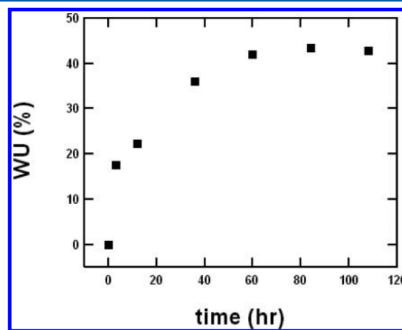
Figure 2. Water uptake, WU , of a PSS-PE sample in liquid water (■) at T = 25 °C as a function of time. The estimated uncertainty in the equilibrated value of WU , based on repetitions on different samples, is about 1%.
