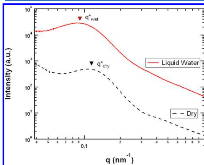
Figure 4. SAXS profiles of a PSS-PE sample in the dry state and after equilibration in liquid water at T = 25 °C.
