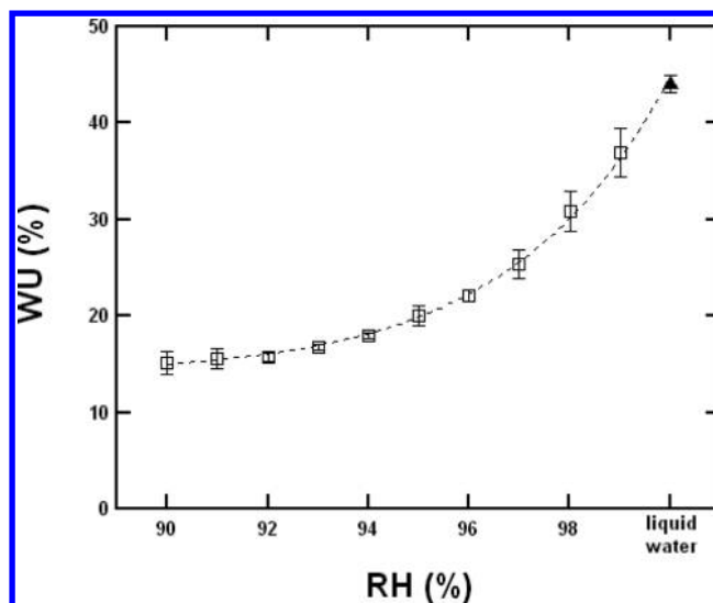
Figure 7. Water uptake, WU , of PSS-PE in humid vapor ( \square ) and in liquid water ( \blacktriangle ) plotted as a function of relative humidity, RH, at T = 25 °C. The dashed curve represents a power-law fit through the humid vapor data.
