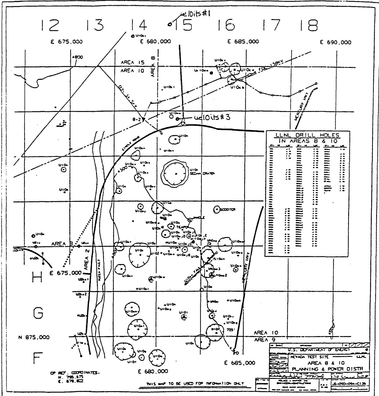
Figure 1. Map of areas 8 and 10 in the northeast corner of Yucca Valley at the Nevada Test Site.
