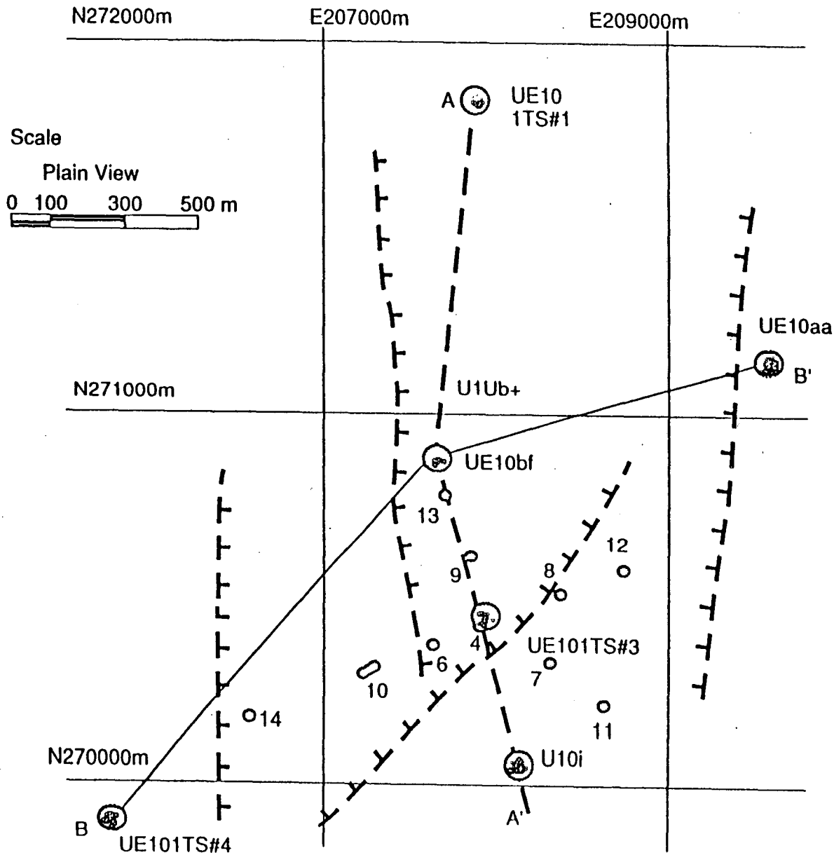
Figure 2. Enlarged map of the area near hole UE10ITS3. The lines AA' and BB' denote the locations of cross-sections shown in Figures 3 and 4, respectively.
