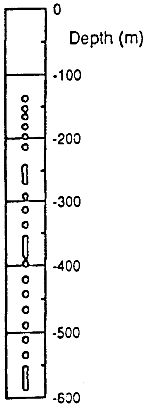
Figure 5. The locations of source and receiver points for the VSP survey.
