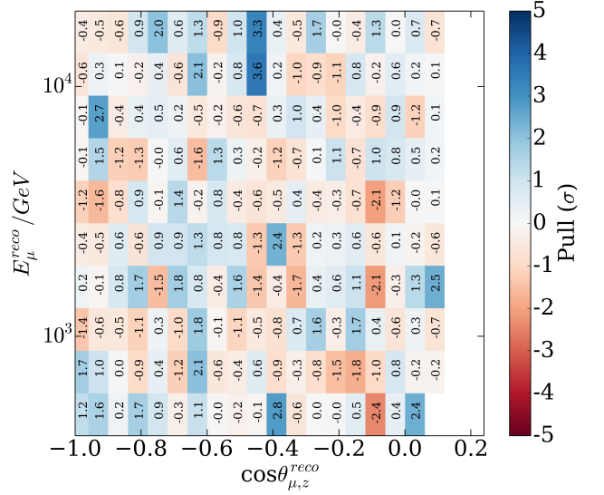
FIG. 3. The statistical-only pulls (shape+rate analysis) per reconstructed energy and zenith angle bin at the best nuisance parameter fit point for the no-sterile hypothesis. The shown empty bins are those that were evaluated in the analysis but had no data events remaining following cuts.
