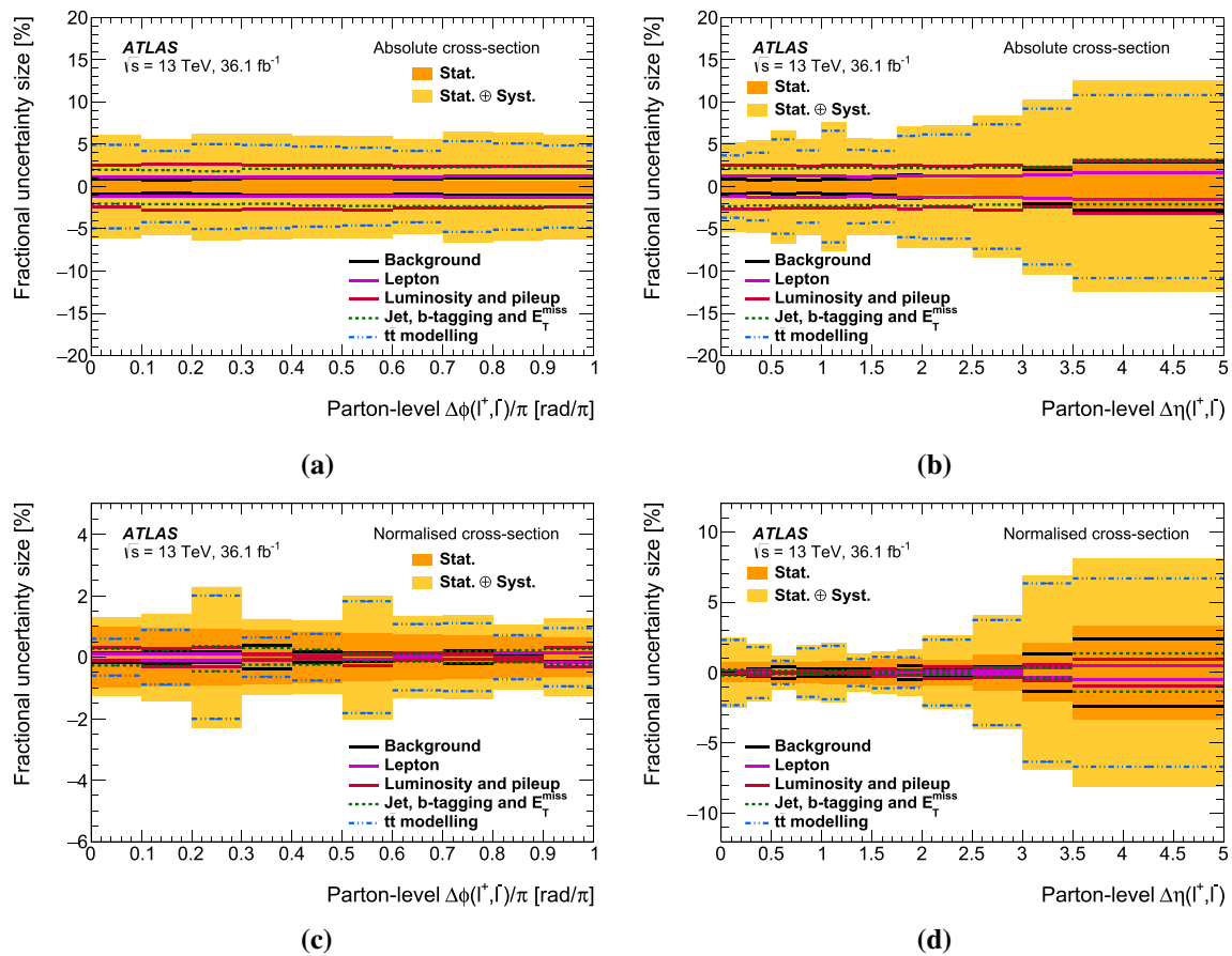
Fig. 7 Systematic uncertainties for the parton-level differential cross-sections: ( top ), absolute a \Delta\phi and b \Delta\eta and ( bottom ), normalised c \Delta\phi and d \Delta\eta . The t\bar{t} modelling uncertainties refer to the contributions
