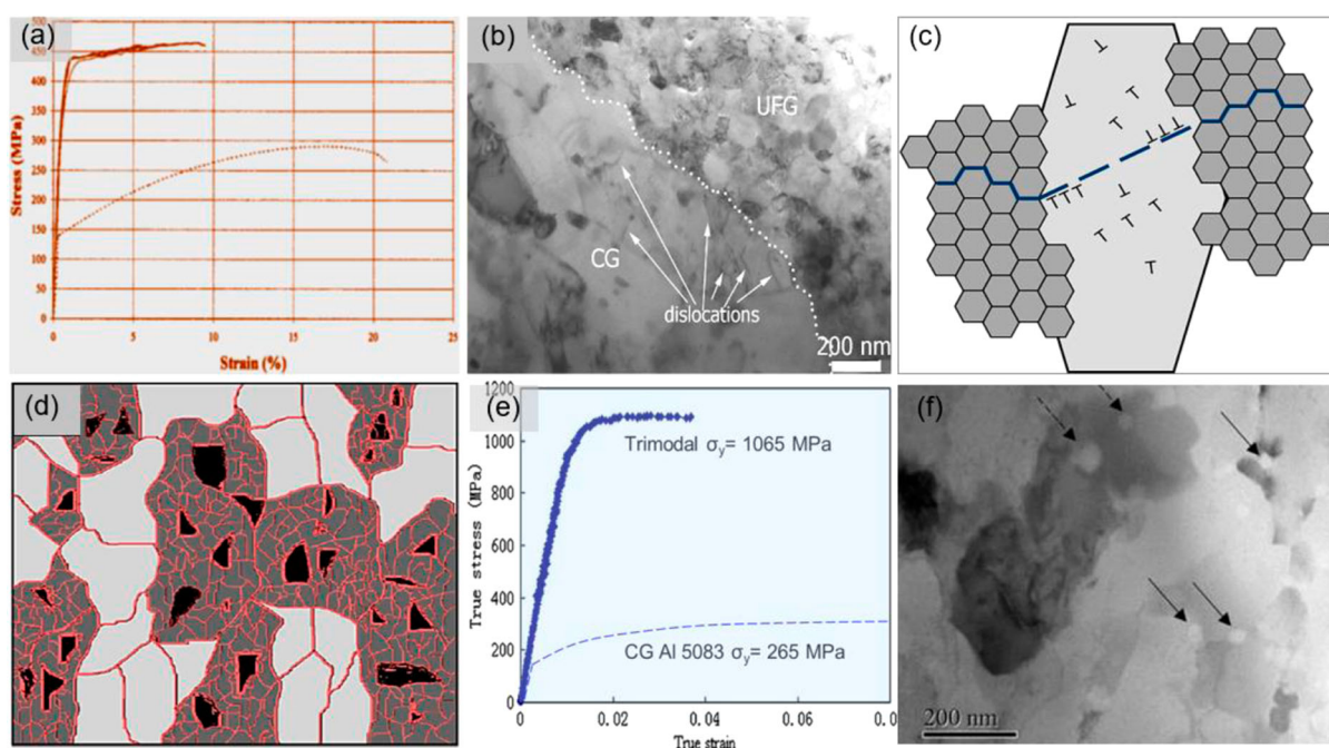
Figure 9. Multi-modal structured materials: (a) Tensile properties of bimodal structured 5083Al alloy [170], (b) High-density dislocation distributed in the CG region [174], (c) Cracks propagate through the NGs, but were blunted when they encounter ductile coarse grains, (d) Structure of trimodal 5083Al composite [175], with (e) high strength of 1065 MPa and a tensile strain-to-failure value 4% [172], and (f) B_4C particles located at NG boundaries highlighted by black arrows [177].
