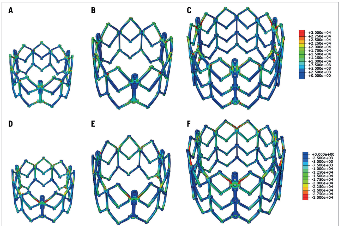
Figure 7. Maximum and minimum principal stress on transcatheter heart valve stent. Maximum (A6C) and minimum (dD6F) principal stresses of stent of 23 mm, 26 mm, and 29 mm SAPIEN XT at mean arterial pressure.
