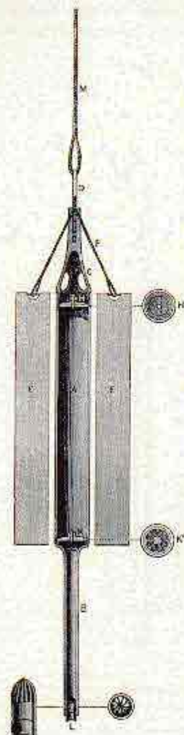
FIG. 7.—Buchanan's Combined Sounding Tube and Water-Bottle.
