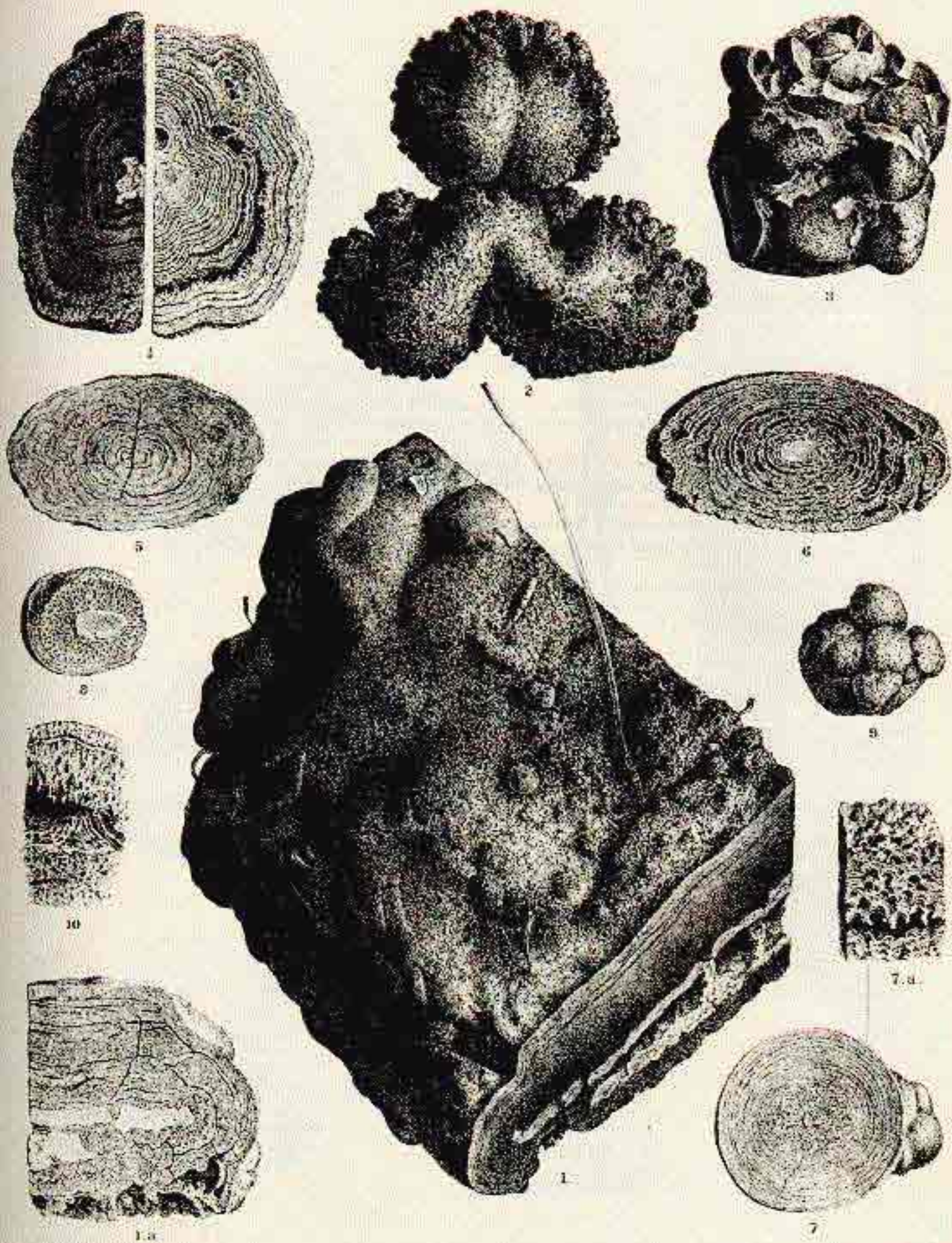
MANGANESE-IRON NODULES.
