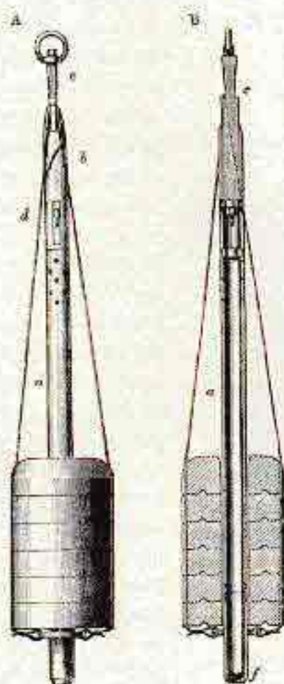
FIG. 6.—Dallie Sounding Machine.
