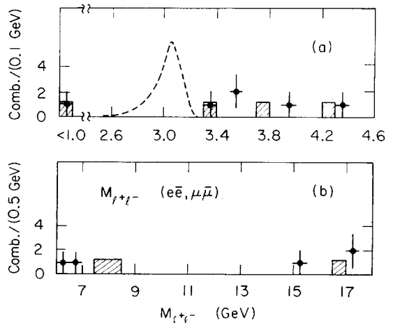
Fig. 1. Invariant mass spectra of e^+e^- , \mu^+\mu^- lepton pairs: (a) in the range 2.6–4.6 GeV, (b) in the range 6–18 GeV. The shaded events correspond to the expected invariant mass distribution from a Monte Carlo calculation with 5 quark flavors. The dotted curve of the \psi signal expected from the “non-perturbative model”.
