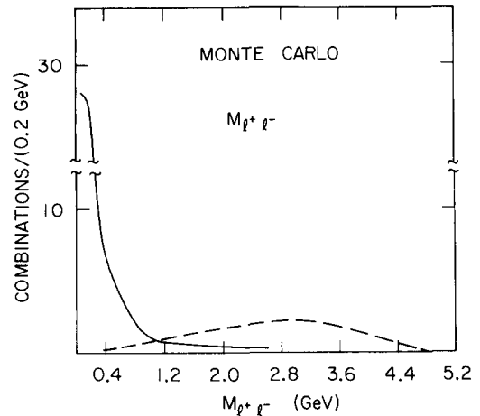
Fig. 2. Invariant mass M_{\ell^+\ell^-} distribution: the solid curve corresponds to a Monte Carlo calculation with 5 quark flavors, the dotted curve corresponds to decay B \rightarrow \ell^+\ell^- X assuming that 10% of B mesons present in the data sample undergo this decay mode.
