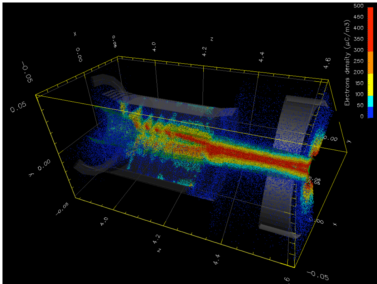
Figure 5: Snapshot of electron macroparticles, colored according to charge density (absolute value), from WARP-POSINST simulation of HCX at t = 3 \mu\text{s} .
