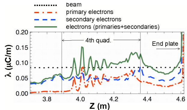
Figure 4: Line charge density \lambda (absolute value), from WARP-POSINST simulation of HCX at t = 3 \mu\text{s} .
