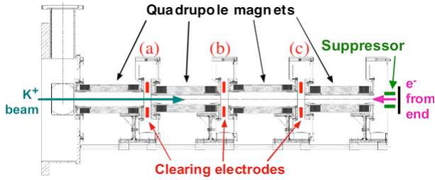
Figure 2: HCX in region of 4 quadrupole magnets, with clearing electrode rings between magnets and a suppressor electrode ring after the last magnet.
