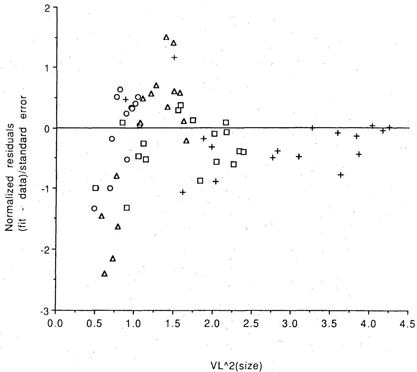
Figure 14: Normalized residuals vs. VL^2(\text{size}) for the VL(\text{size}) generalized fit (4 point type & below)
