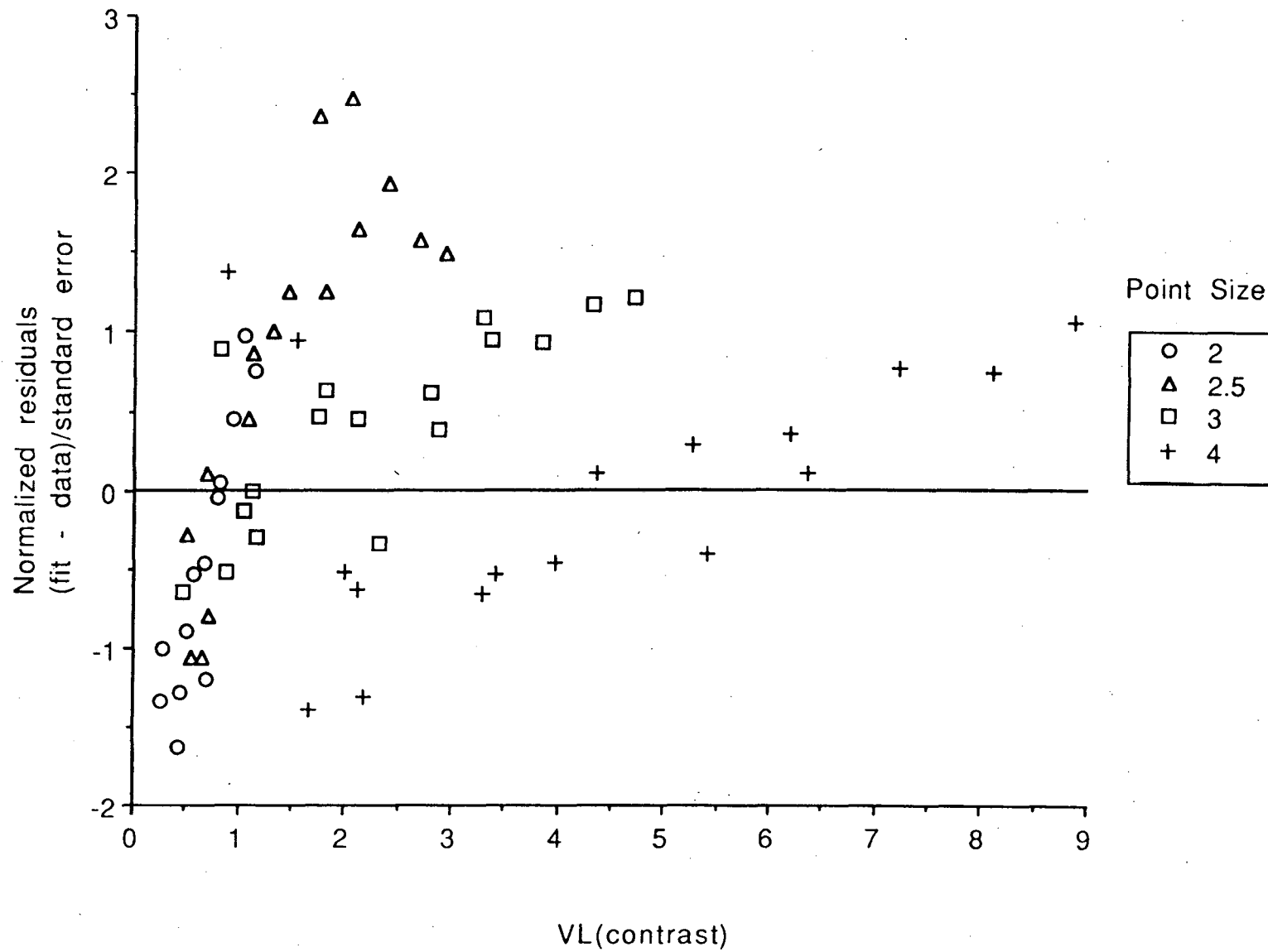
Figure 11: Normalized residuals vs. VL(contrast) for the generalized fit (4 point type & below)
