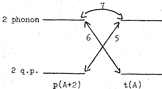
Fig. 2. Microscopic two-phonon states have parentage coefficients connecting them to other two quasi-particle states or to each other.
