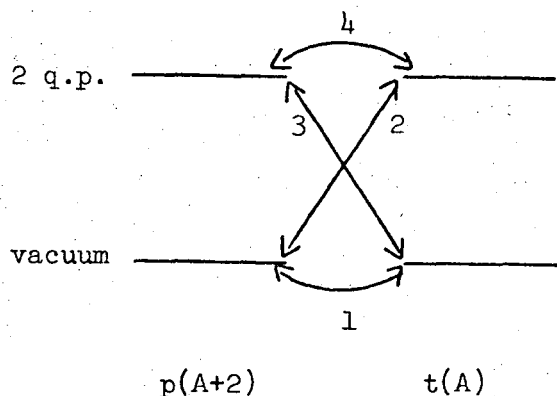
Fig. 1. Four types of parentage coefficients occur in a nucleus with vacuum ground state and two quasi-particle excited states.
