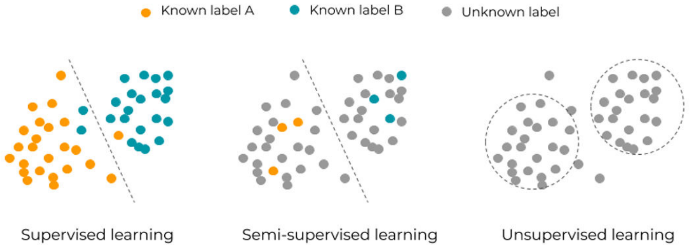
Figure 2. Three classical learning frameworks in artificial intelligence: supervised, semi-supervised, and unsupervised learning. Supervised learning relies on known input-output pairs. If some output labels are difficult or expensive to get, semi-supervised learning can apply. If no labels are available, unsupervised learning allows for a more exploratory approach of data.
