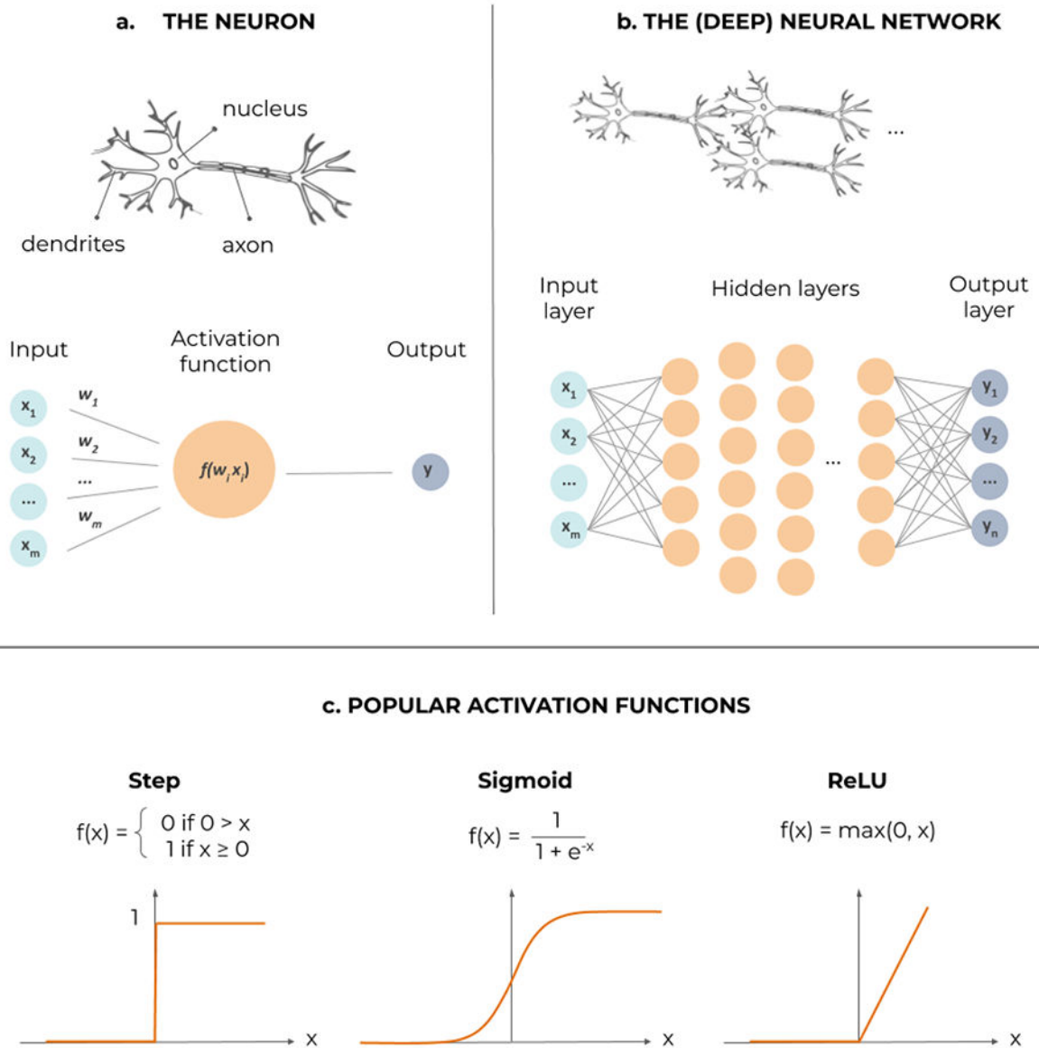
Figure 5. Artificial neural networks in a nutshell. (a) The formal neuron, processing several dendritic inputs through a nonlinear activation function f , to produce its actional output. (b) The neurons can be interconnected in a feed-forward way, into successive layers; as soon as a nonlinear ‘hidden’ layer is inserted in between the inputs and outputs, the network can potentially approximate any function; specific activation functions can be fitted in the output layer to achieve either regression or classification. (c) Examples of nonlinear activation functions in the hidden layers: the step function, from biological inspiration, the sigmoid, its continuous and differentiable surrogate, and the rectified linear unit (ReLU), that improves training of deep layers.
