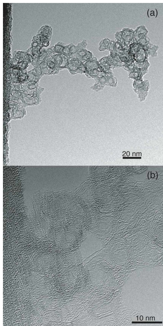
Figure 5. TEM images of a soot particle irradiated at 1064 nm with a fluence of 1 \text{ J/cm}^2 . The particle electric mobility diameter was 100 nm. (a) The aggregate in this TEM image has a branched-chain morphology similar to that of the non-irradiated particles, despite changes in the particle fine structure (b). (b) Higher-magnification TEM image of a part of the same aggregate.
