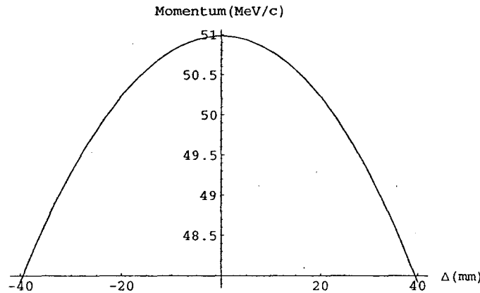
FIG. 6: Central momentum vs. \Delta
