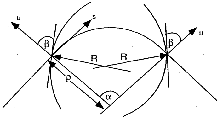
FIG. 3: Geometry of a symmetric wedge bending magnet
