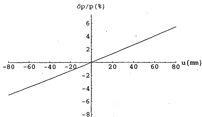
FIG. 22: Relative momentum vs. distance at the focus
