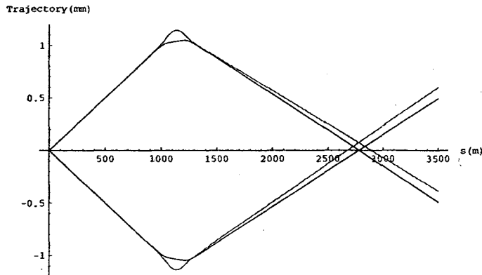
FIG. 13: Trajectories computed by numerical integration, for the measured field, for \Delta = -19.1 mm. The red curves correspond to trajectories in the bend plane, relative to the reference trajectory; the initial values are u'_0 = \pm 1 mrad. The black curves are trajectories in the non-bend plane, again corresponding to z'_0 = \pm 1 mrad.
