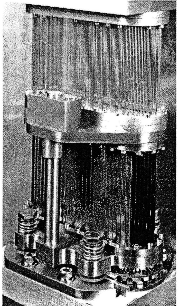
Figure 3. Flexible cage and bellows shield assembly.
