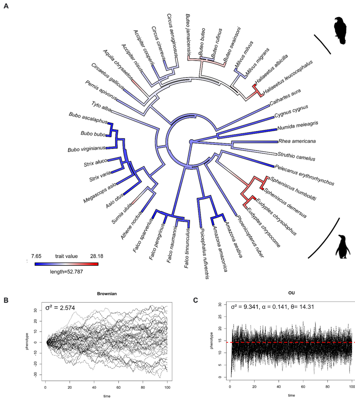
Figure 2. (A) Ancestral state reconstruction of intraocular pressure (IOP) from 43 species of birds. Red color represents high IOP, and blue color represents low IOP. (B) Simulations of IOP evolution under Brownian model with evolutionary rate (drift) parameter ( \sigma^2 ). (C) Simulations of IOP evolution under OU model with evolutionary rate (drift) parameter ( \sigma^2 ), pull rubber band (or pull towards optimum) parameter ( \alpha ), and optimum trait value ( \theta ). Red dashed line represents optimum value.
