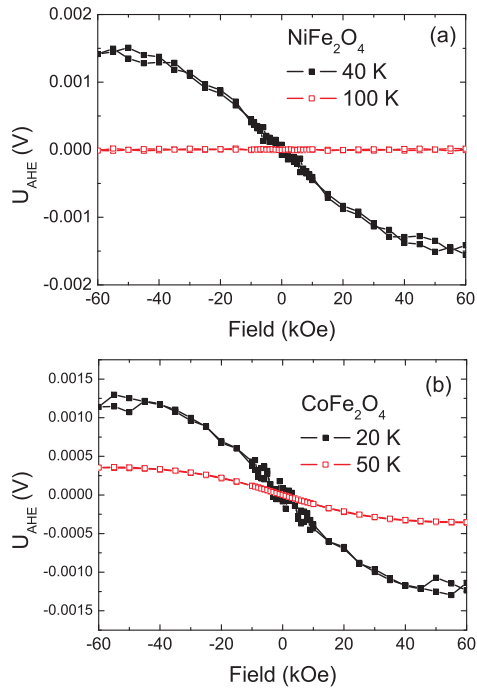
FIG. 14: Anomalous Hall voltage vs magnetic field for (a) the composites of \text{NiFe}_2\text{O}_4 nanocrystals and ZnO and (b) the composites of \text{CoFe}_2\text{O}_4 nanocrystals and ZnO.
