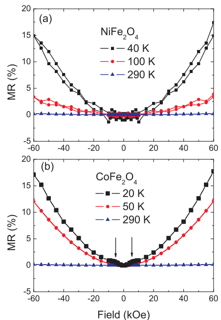
FIG. 13: The field dependent MR of (a) the composites of NiFe 2 O 4 nanocrystals and ZnO and (b) the composites of CoFe 2 O 4 nanocrystals and ZnO. The solid lines are guides to the eye.
