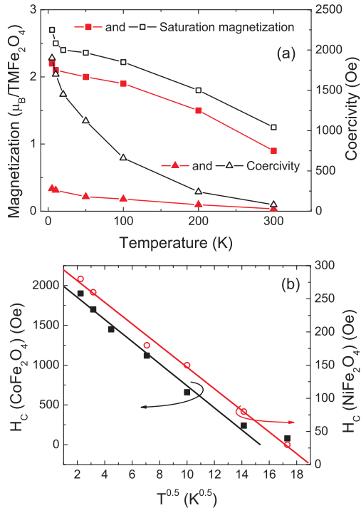
FIG. 5: (a) Temperature dependent saturation magnetization and coercivity for \text{NiFe}_2\text{O}_4 (red solid symbols) and \text{CoFe}_2\text{O}_4 (black open symbols). The solid lines are guides for eyes. (b) The plot of coercivity as a function of T^{1/2} .
