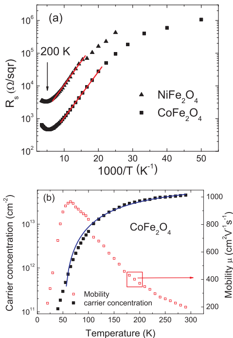
FIG. 12: (a) The temperature dependent sheet resistance (the solid lines show the linear fitting in the temperature range of 60-100 K), and (b) free carrier concentration and mobility of the composites of NiFe 2 O 4 or CoFe 2 O 4 nanocrystals and ZnO. The solid line is a fitting of carrier concentration by the function e^{-E_a/k_B T} .
