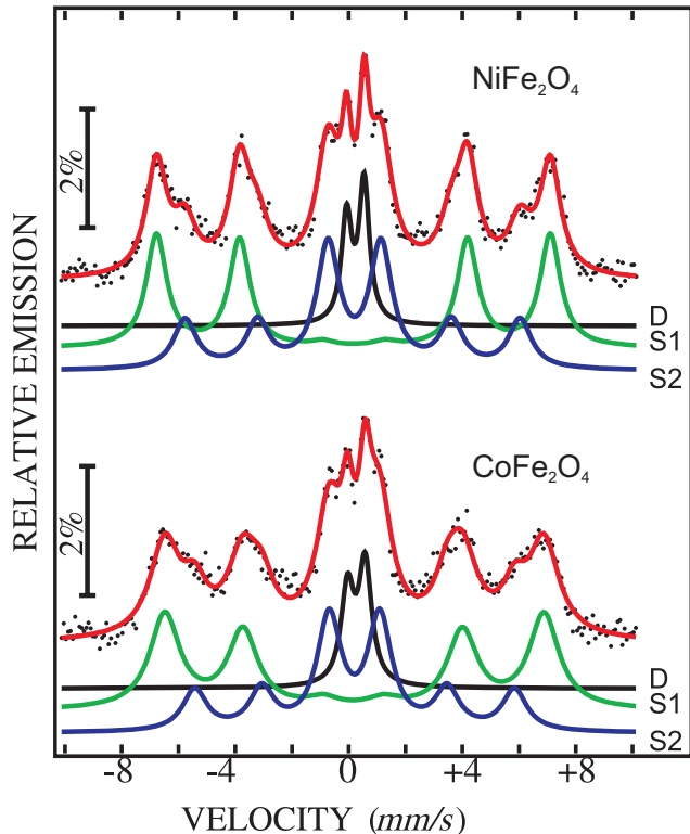
FIG. 11: Room temperature CEMS of \text{NiFe}_2\text{O}_4/\text{ZnO} and \text{CoFe}_2\text{O}_4/\text{ZnO} composites. The notations for the fitting lines are given as D (doublet) and S1, S2 (sextet).
