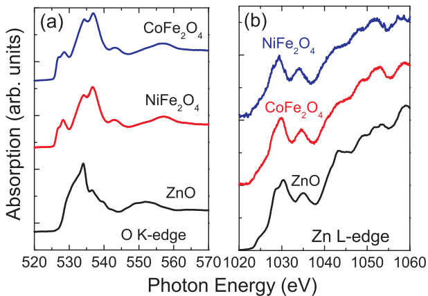
FIG. 9: The XA spectra of total electron yield (TEY) at the (a) O K-edge, and (b) Zn L-edge.
