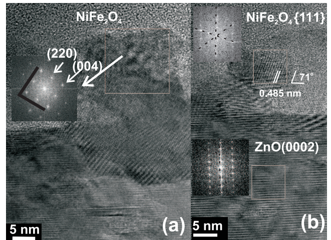
FIG. 3: High resolution TEM image for representative \text{NiFe}_2\text{O}_4 nanocrystals. (a) the specimens is tilted by 11^\circ . \text{NiFe}_2\text{O}_4 nanocrystal is identified. The black lines guide the eyes to show the cubic symmetry of the secondary phase. (b) Another \text{NiFe}_2\text{O}_4 nanocrystals with the orientation of (111)\parallel\text{ZnO}(0001) as confirmed by FFT patterns. The clearly visible planes are \text{NiFe}_2\text{O}_4(111) with an angle of \sim 71^\circ from the surface. In FFT patterns the dashed lines indicate the sets of lattice planes.
