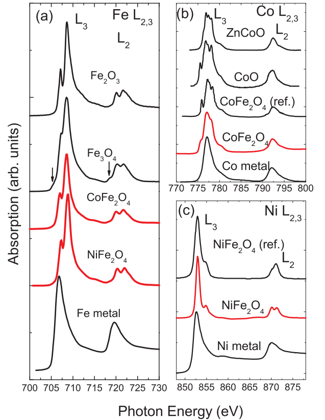
FIG. 7: XAS of \text{NiFe}_2\text{O}_4 and \text{CoFe}_2\text{O}_4 along with reference spectra from pure metal and oxides at the (a) Fe L_{2,3} -edge, (b) Co L_{2,3} -edge and (c) Ni L_{2,3} -edge. The reference spectra are taken from published papers: \text{Fe}_2\text{O}_3 41 , \text{Fe}_3\text{O}_4 41 , \text{CoO} 35 , \text{ZnCoO} 36 , \text{NiFe}_2\text{O}_4 40 and \text{CoFe}_2\text{O}_4 37 .
