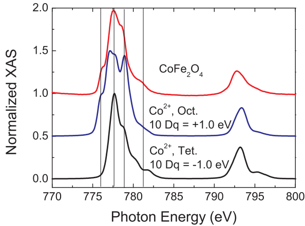
FIG. 8: The Co L 2,3 -edge XAS spectrum of CoFe 2 O 4 along with theoretical calculations for a tetrahedral ( 10 D_q = -1 eV) and an octahedral ( 10 D_q = +1 eV) coordination of Co ions..
