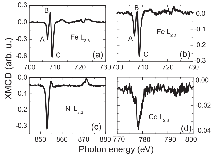
FIG. 10: XMCD at Fe, Ni and Co L 2,3 absorption edge. NiFe 2 O 4 : (a) and (c). CoFe 2 O 4 : (b) and (d). Peak labels at Fe L 3 -edge: A for Fe 2+ at octahedral sites, B for Fe 3+ at tetrahedral sites and C for Fe 3+ at octahedral sites 43 .
