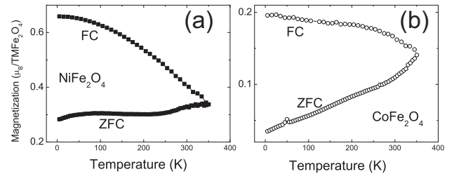
FIG. 6: ZFC/FC magnetization curves measured with a field of 50 Oe. (a) \text{NiFe}_2\text{O}_4 and (b) \text{CoFe}_2\text{O}_4 . Up to 350 K, no ZFC maximum was observed for \text{CoFe}_2\text{O}_4 .
