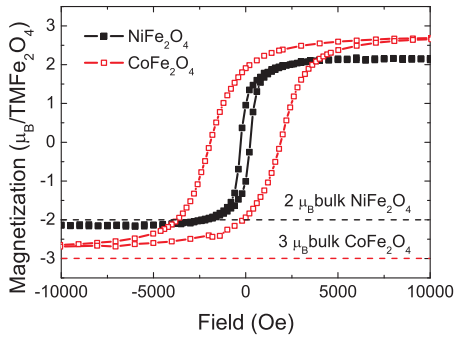
FIG. 4: Hysteresis loops measured at 5 K for \text{NiFe}_2\text{O}_4 and \text{CoFe}_2\text{O}_4 nanocrystals. They show drastic difference in coercivity field.
