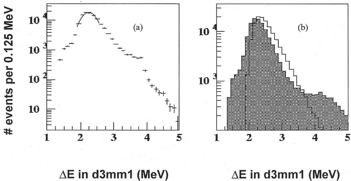
Figure 7. Histograms of the peak region in d3mm1. In 7(a), a Gaussian distribution fit to the center of the peak is shown as a curve, and the data are shown as points with error bars (in the center of the peak, the error bars are too small to be visible on this scale). In 7(b), the data are shown as a shaded histogram, and a histogram corresponding to a Landau distribution is superimposed.
