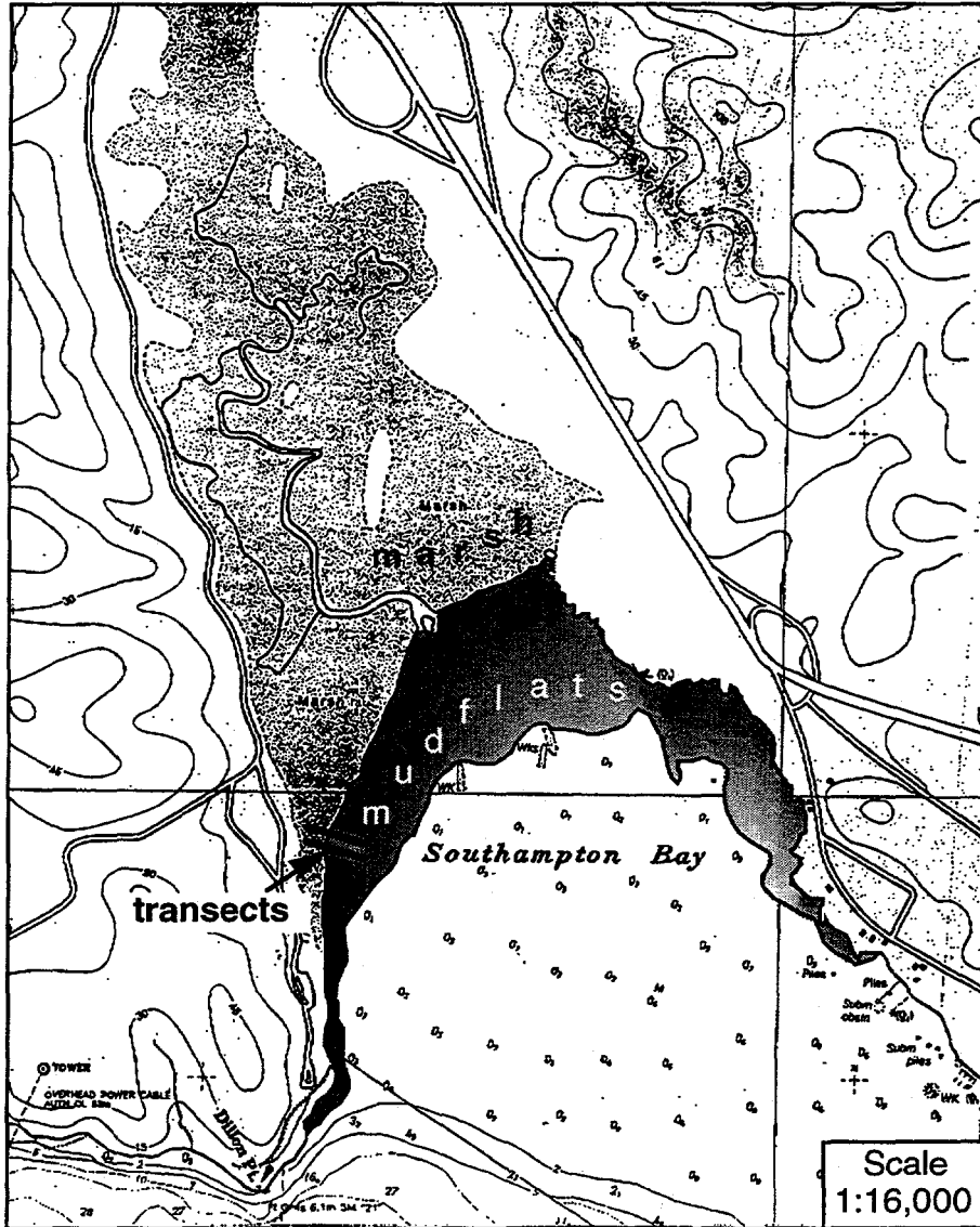
Figure 2.4 Location of sampling transects within the marshes and mudflats of Benicia State Park.
