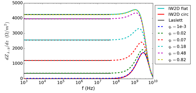
FIG. 9. Transverse indirect space charge per unit of length for b = 0.35 cm and \beta = 0.9 as a function of frequency for different q_r = (a - b)/(a + b) compared with the circular and flat beam pipe given by IW2D, and with theory which uses the Laslett coefficients at low frequency.
