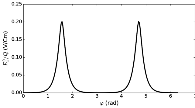
FIG. 5. Longitudinal electric field per unit of charge in the elliptic beam pipe of the SPS accelerator at the injection energy, calculated in \mu_0 = 0.1 at 100 MHz as a function of \varphi .
