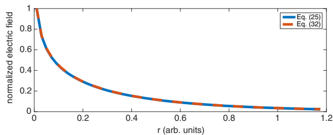
FIG. 3. Comparison between the Green's function in free space computed with Eq. (25) (blue line) and Eq. (32) (red dashed line) with 120 summation terms, as a function of the radial coordinate and \varphi = \pi/2 , for a focal distance F = 1 .
