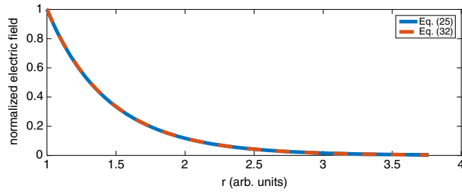
FIG. 2. Comparison between the Green's function in free space computed with Eq. (25) (blue line) and Eq. (32) (red dashed line) with 120 summation terms, as a function of the radial coordinate and \varphi = 0 , for a focal distance F = 1 .
