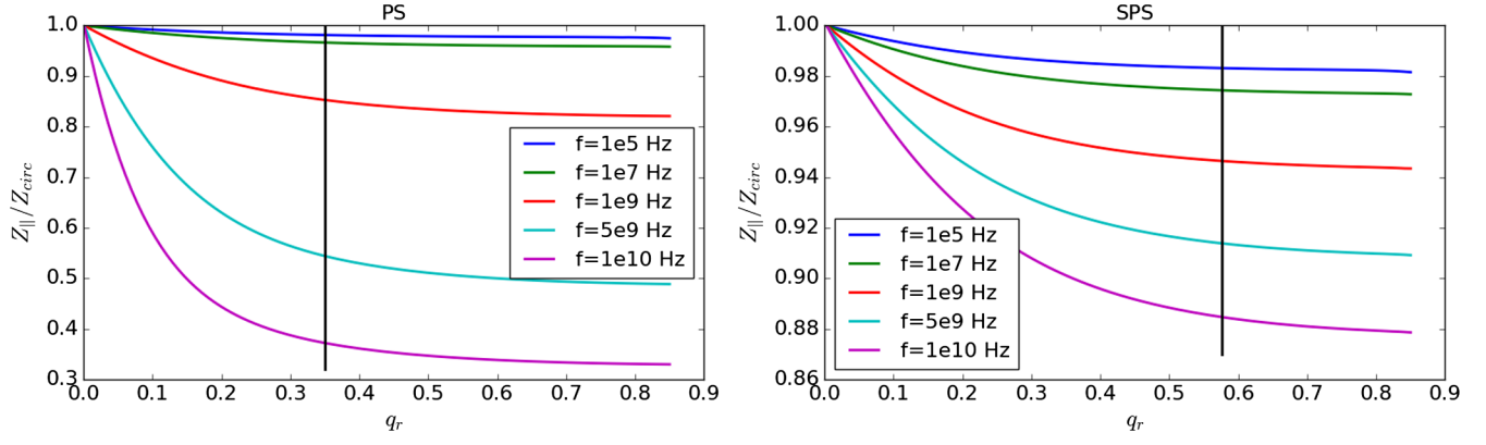
FIG. 7. Longitudinal form factor as a function of q_r = (a - b)/(a + b) for the PS (left) and the SPS (right) injection energies at different frequencies. The vertical black lines correspond to the machines beam pipe geometries.
