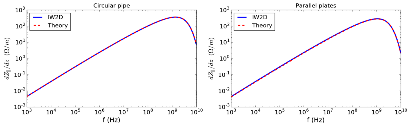
FIG. 6. Longitudinal indirect space charge per unit of length for b = 3.5 cm and \beta = 0.9 as a function of frequency. Comparison between IW2D and Eq. (38) for circular pipe (left) and parallel plates (right).
