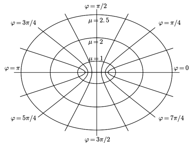
FIG. 1. Elliptic coordinates. The \varphi coordinate describes confocal hyperbolas that are symmetrical about the x-axis. The \mu coordinate describes confocal ellipses centered on the origin of the coordinate system.
