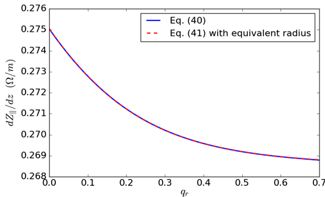
FIG. 8. Longitudinal indirect space charge impedance as a function of q_r = (a - b)/(a + b) for the PS accelerator for a frequency of 100 kHz. Comparison between Eq. (40) and Eq. (41) by using the equivalent radius defined in Eq. (42).
