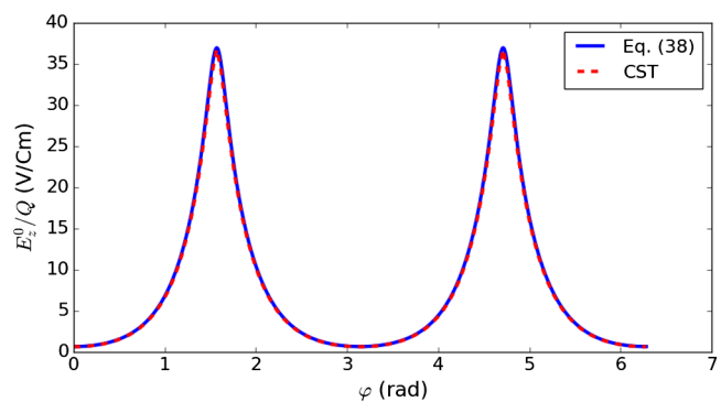
FIG. 4. Comparison between the longitudinal electric field per unit of charge computed with Eq. (38) (blue line) and by CST (red dashed line) with 40 summation terms, calculated in \mu = 0.1 at 100 MHz as a function of \varphi .
