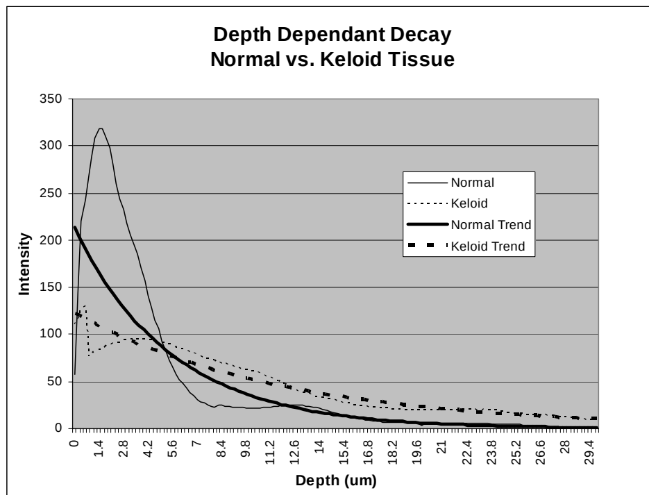
Figure 1. Depth dependant decay curves showing the exponential decrease in signal intensity as depth increases for both normal and keloid tissues. Thin lines represent raw data while thick lines represent trendlines. Solid lines show normal data while broken lines show keloid data.
