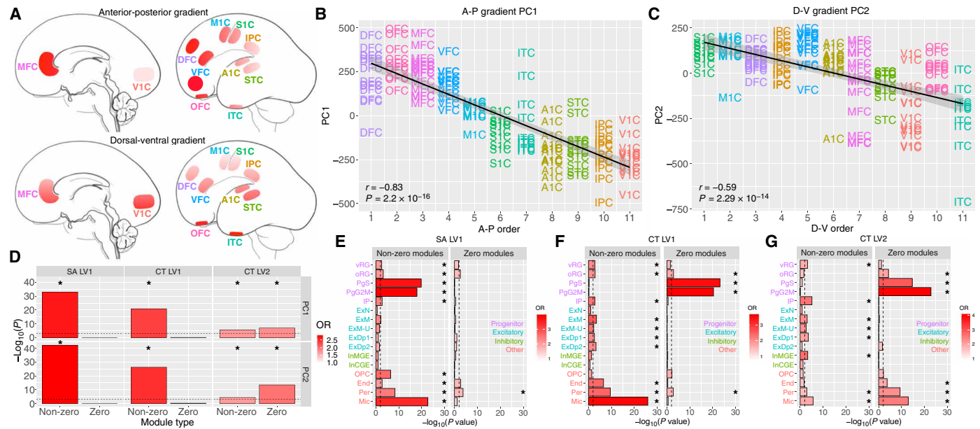
Fig. 5. Enrichment between PLS non-zero modules and genes involved in prenatal A-P and D-V expression gradients and prenatal cell types. (A) Cortical brain areas sampled from 12 to 24 weeks after conception from the Development PsychENCODE RNA-seq dataset from Li and colleagues (17). Adjustment for-confounds PCA (30) was used to isolate (B) A-P (PC1) and (C) D-V (PC2) expression gradients. (D) -\log_{10} P values for enrichment tests of non-zero and zero modules for SA LV1, CT LV1, and CT LV2 for genes isolated from PC1 and PC2. (E to G) Enrichments in prenatal cell types for SA LV1 (E), CT LV1 (F), and CT LV2 (G). Asterisks mark enrichments at FDR q < 0.01 . MFC, medial prefrontal cortex; V1C, primary visual cortex; OFC, orbitofrontal cortex; DFC, dorsolateral refrontal cortex; M1C, primary motor cortex; VFC, ventrolateral prefrontal cortex; A1C, primary auditory cortex; ITC, inferior temporal cortex; STC, superior temporal cortex; IPC, posterior inferior parietal cortex; S1C, primary somatosensory cortex.
