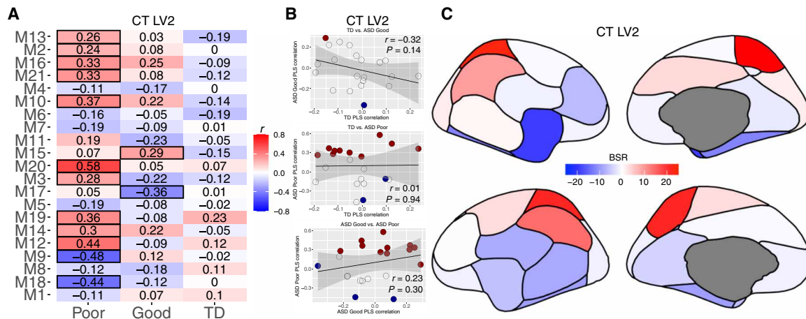
Fig. 3. Atypical association between gene expression and CT that is specific to the ASD Poor subtype. Atypical association specific to ASD Poor between gene coexpression modules and CT, as described in CT LV2. (A) CT LV2 PLS correlations for each gene coexpression module (rows) and each group (columns). Modules with a black outline are non-zero modules where the correlation between gene expression and SA is significantly non-zero, as indicated by 95% bootstrap CIs not encompassing a correlation of 0. Nearly all of the non-zero modules for CT LV2 are present for the ASD Poor subtype. (B) Lack of similarity in CT LV2 PLS correlations between groups. In these scatterplots, each dot is a coexpression module, and the x and y axes indicate the PLS correlations for different groups. Dots colored in dark red and dark blue indicate the non-zero modules (red for positive correlations and blue for negative correlations), while gray dots indicate zero modules. (C) CT LV2 BSRs for each brain region in the GCLUST parcellation. Regions with red BSRs have correlations that manifest in the directionality shown in heatmaps in (A). Brain regions with blue BSRs have correlations where the directionality is flipped relative to the heatmaps in (A). Stronger BSRs indicate regions that are more important in driving the CT LV2 relationship.
