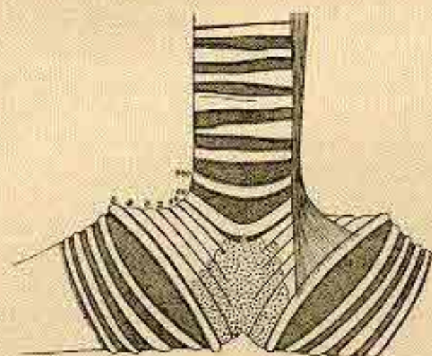
FIG. 29.—Syrinx of Diomedea exulans , from before. About natural size.
