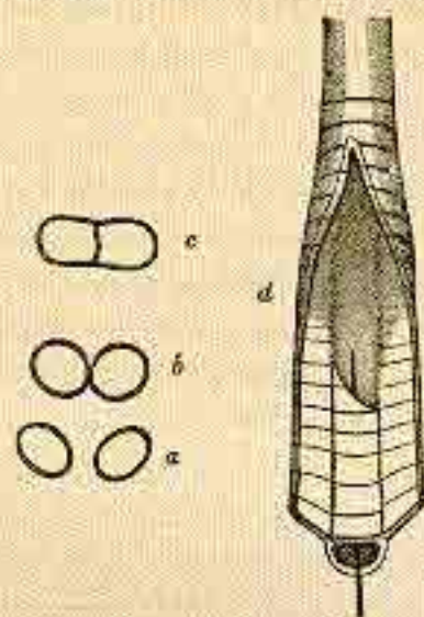
FIG. 19.—a, b, c, sections of syrinx and trachea of Ossifraga along the lines a, b, c, of fig. 17, to show the double nature of the tracheal tube below, and its complete division by a median septum above. d, trachea opened from the side, to show the median septum, dividing it into two parallel tubes, through the left of which a pointer is passed, below, and terminating above by a free margin.
