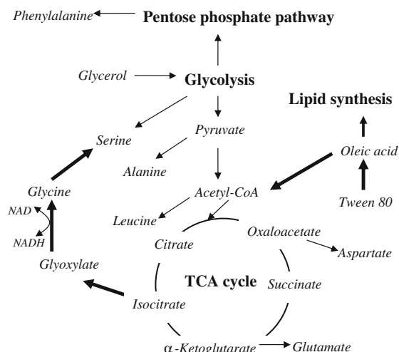
Fig. 5 Central metabolic pathways of M. smegmatis revealed by isotopomer analysis. The thick arrows indicate the pathways up-regulated under hypoxia. The metabolites are in italics
