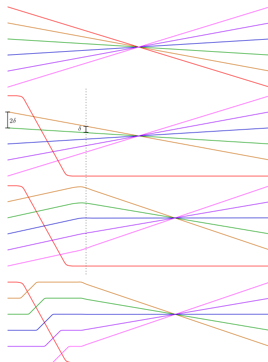
FIGURE 25. Key move used to construct a family of pseudolines, slightly modified from [RS19].
