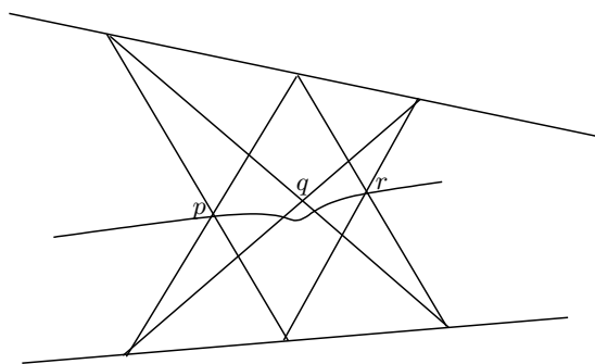
FIGURE 24. The pseudo-Pappus arrangement.
