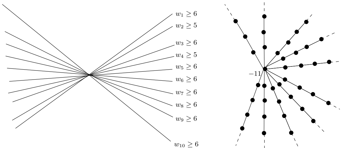
FIGURE 16. Left: a pencil of 10 lines decorated with weights. Right: the plumbing graph for Y , the central vertex has self-intersection -11 , all the rest self-intersection -2 . Eight of the legs have at least 5 vertices each (including the central vertex), and two remaining legs have at least 4 vertices each.
