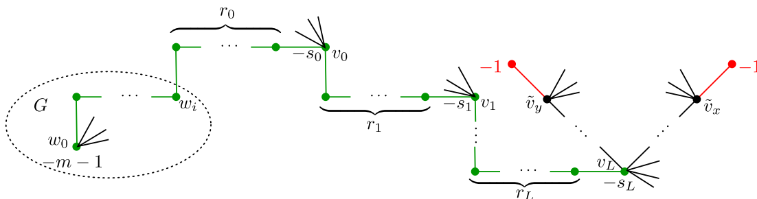
FIGURE 23. How to compute the tangencies from the graph G following the proof of Proposition 7.23.
