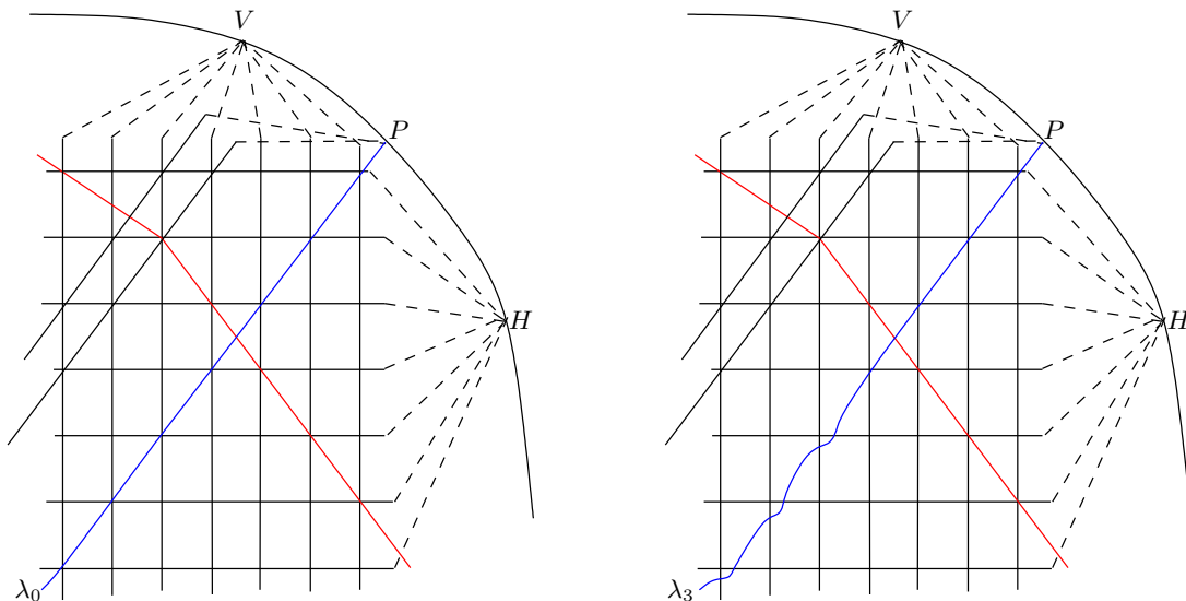
FIGURE 19. Pseudoline arrangements and fillings with different topology.
