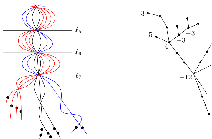
FIGURE 21. In the pseudoline arrangement \mathcal{Q} of Figure 17, we replace \ell_3 with a bundle of curves passing through the existing intersections of \ell_3 with \ell_5 , \ell_6 , \ell_7 , and \ell_0 . (Only part of the arrangement is shown.) Note that the additional curves create no extra intersections with the pseudolines of \mathcal{Q} . All the intersection points are marked, and there are additional free marked points that correspond to higher weights. In the resolution graph of the singularity, the leg corresponding to \ell_3 is replaced by a tree with additional branching, as shown. All unlabeled vertices have self-intersection -2 .
