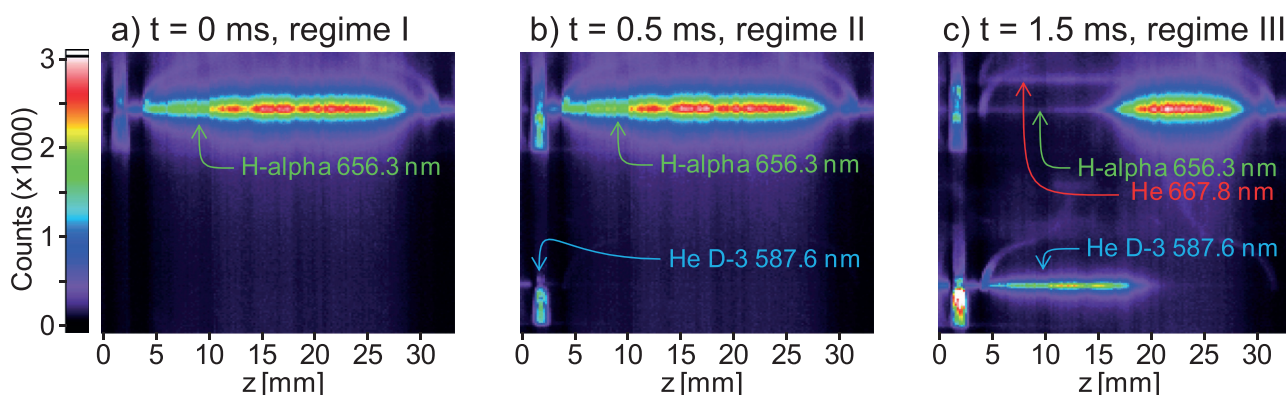
FIG. 2. (a)–(c) Spectrometer images corresponding to region of interest in Fig. 1(c), showing the hydrogen H \alpha (656.3 nm) and helium D 3 (587.6 nm) emission lines for discharge delays of 0 ms, 0.5 ms, and 1.5 ms, respectively, at P_{He} = 65 psi (absolute) and P_{H_2} = 100 Torr.
