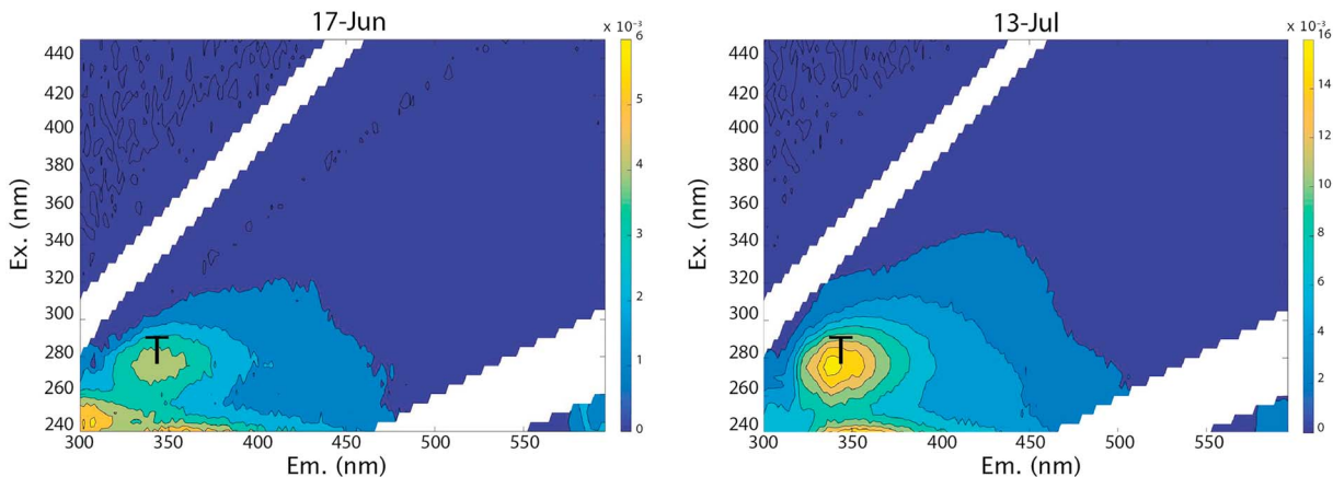
Figure 6. Fluorescence excitation-emission matrices measured in samples from Fox Canyon River taken at the Greenland ice sheet (GIS) source (FCS). T indicates tryptophan protein-like peaks. Peaks are displayed in Ramen units.
