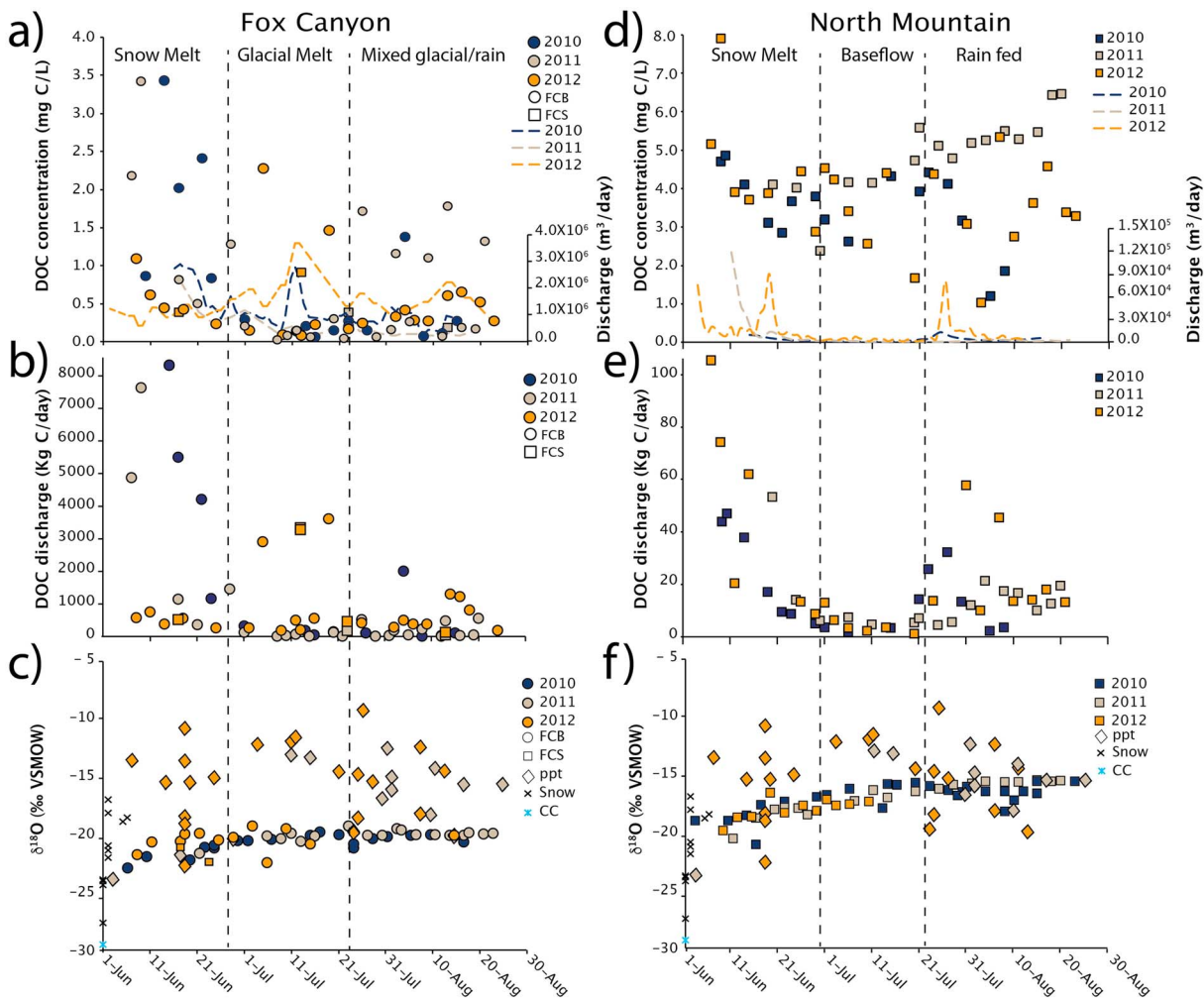
Figure 3. Time series of (a, d) dissolved organic carbon (DOC) concentrations and discharge, (b, e) DOC discharge, and (c, f) \delta^{18}\text{O} (left) from Fox Canyon and North Mountain. Year 2010 is in blue, 2011 in gray, and 2012 in orange. (a) Squares represent samples from the source (FCS) and circles from the bridge (FCB). Note that Fox Canyon River has a higher discharge than North Mountain. Discharge measurements for Fox Canyon were made at the bridge (FCB), and the discharge curves (lines) represent a 2-point moving average of biweekly discharge measurements. (a–c) Circles represent samples taken at the bridge (FCB) squares at the source (FCS). Snow samples refer to samples taken from snow pits each May and any precipitation that fell as snow. Precipitation samples (ppt) represent rain (and sleet) and were collected in a bucket during each precipitation event. CC refers to a snow sample from a pit at Camp Century on the Greenland ice sheet. (d) Squares represent North Mountain DOC samples. Discharge curves were calculated by combining episodic discharge measurements with continuous measurements from a pressure transducer. (f) Squares represent samples from North Mountain; stream, ppt, snow, and CC are the same as those in panel (c).
