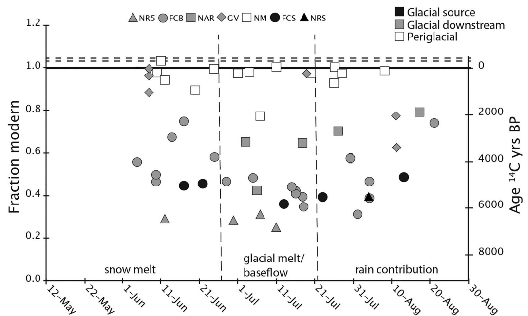
Figure 8. Time series of radiocarbon (in fraction modern [F] ) of particulate organic carbon in (full symbols) four glacially sourced and (open square) one periglacial river in NW Greenland. For glacially sourced rivers, black symbols indicate sampling sites near the source and gray symbols sampling downstream. Solid horizontal line indicates F = 1 (0 years BP). Dashed horizontal lines indicate the range of F in background atmospheric \text{CO}_2 during June to August 2010 to 2012 (Point Barrow, AK, USA; Xu, personal communication, 2016).
